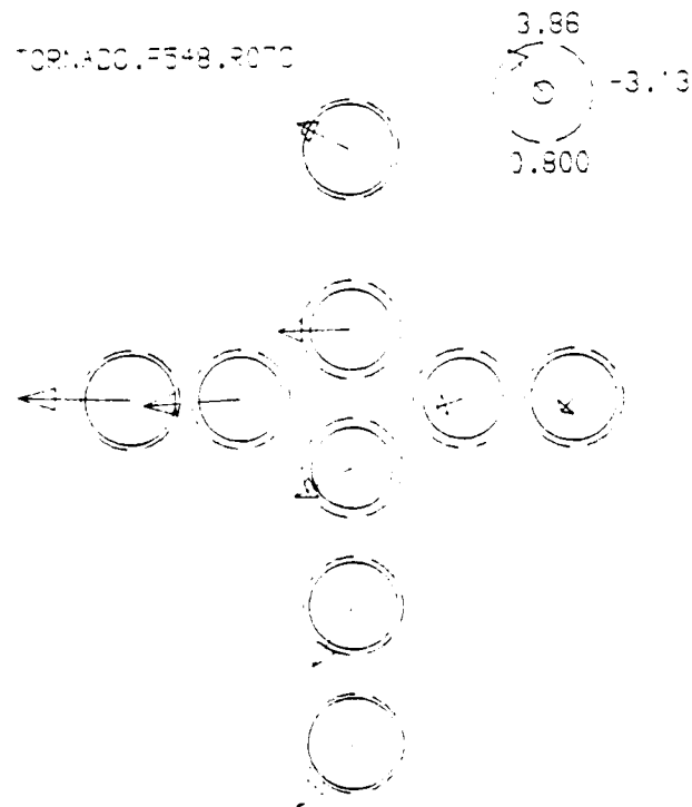
Fig 10 Example of flow survey results with aircraft sideslipping
