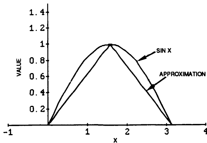
Figure 2. Direct interpolation
