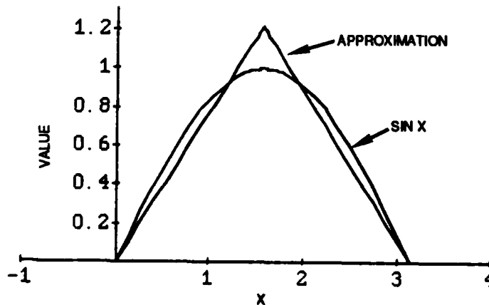
Figure 3. Galerkin approximation
