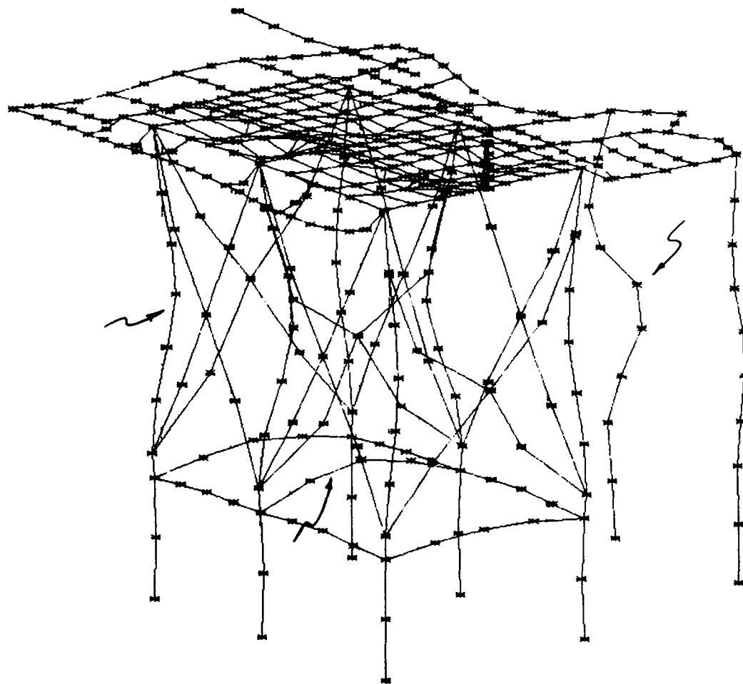
Figure 19: Mode 2-6 (122.2 cps): A Major Structural Mode Involving Nearly All of the Structure (High Damage Potential)
