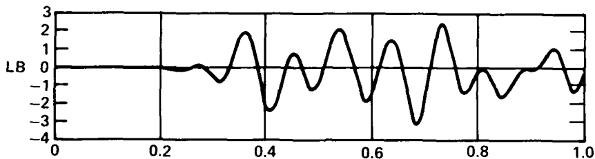
SOLUTION APPROACH 2 (12 MODES)
