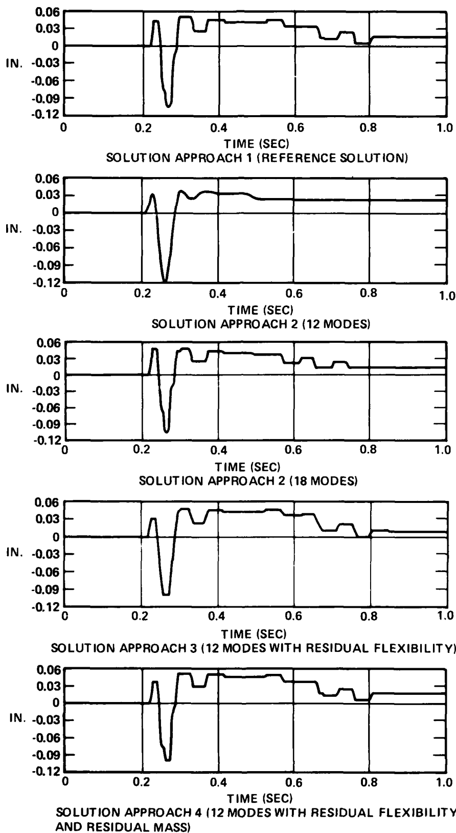
FIGURE 4. — RELATIVE DISPLACEMENT; 17/27
