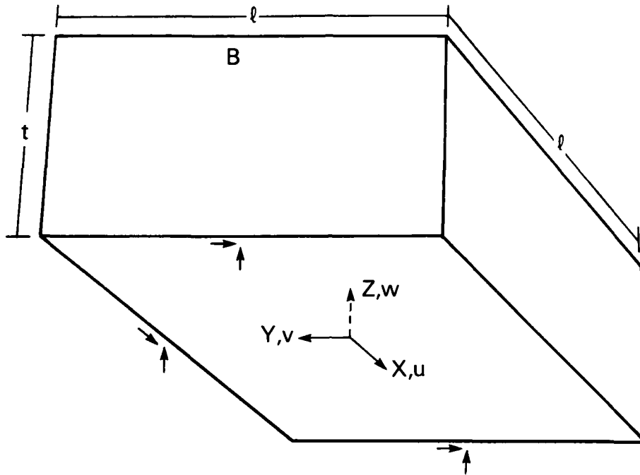
FIG. 1 TEST PROBLEM
