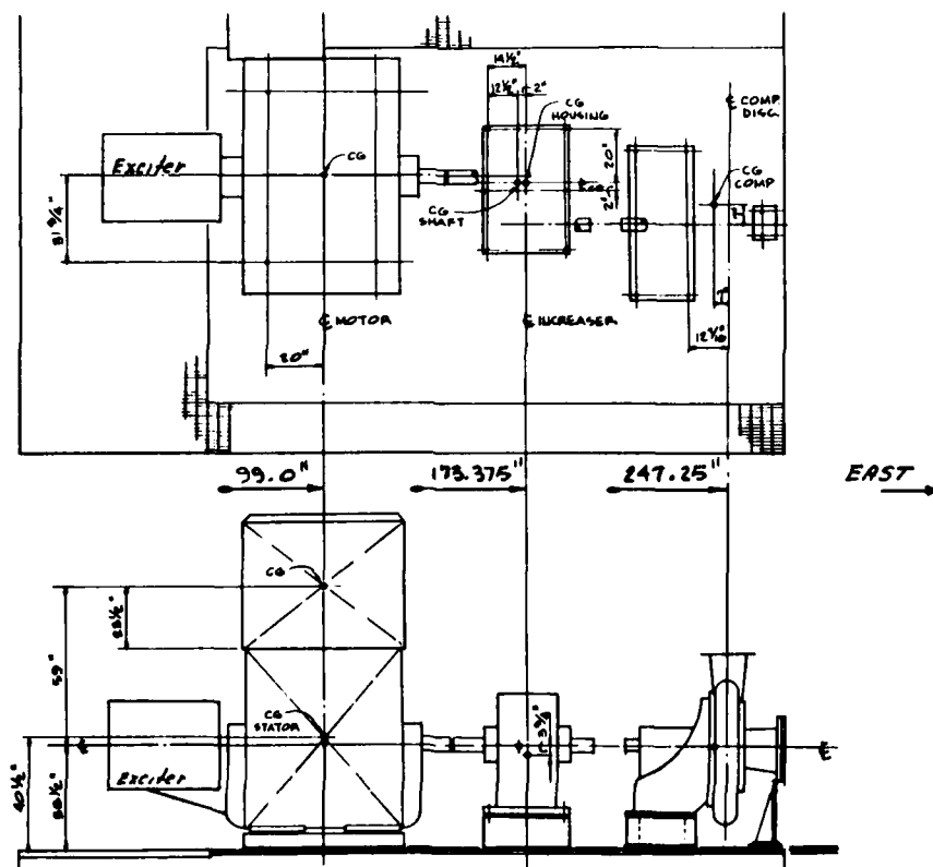
Figure 5: Basic Layout of the Motor, Increaser, Compressor and Shafting
