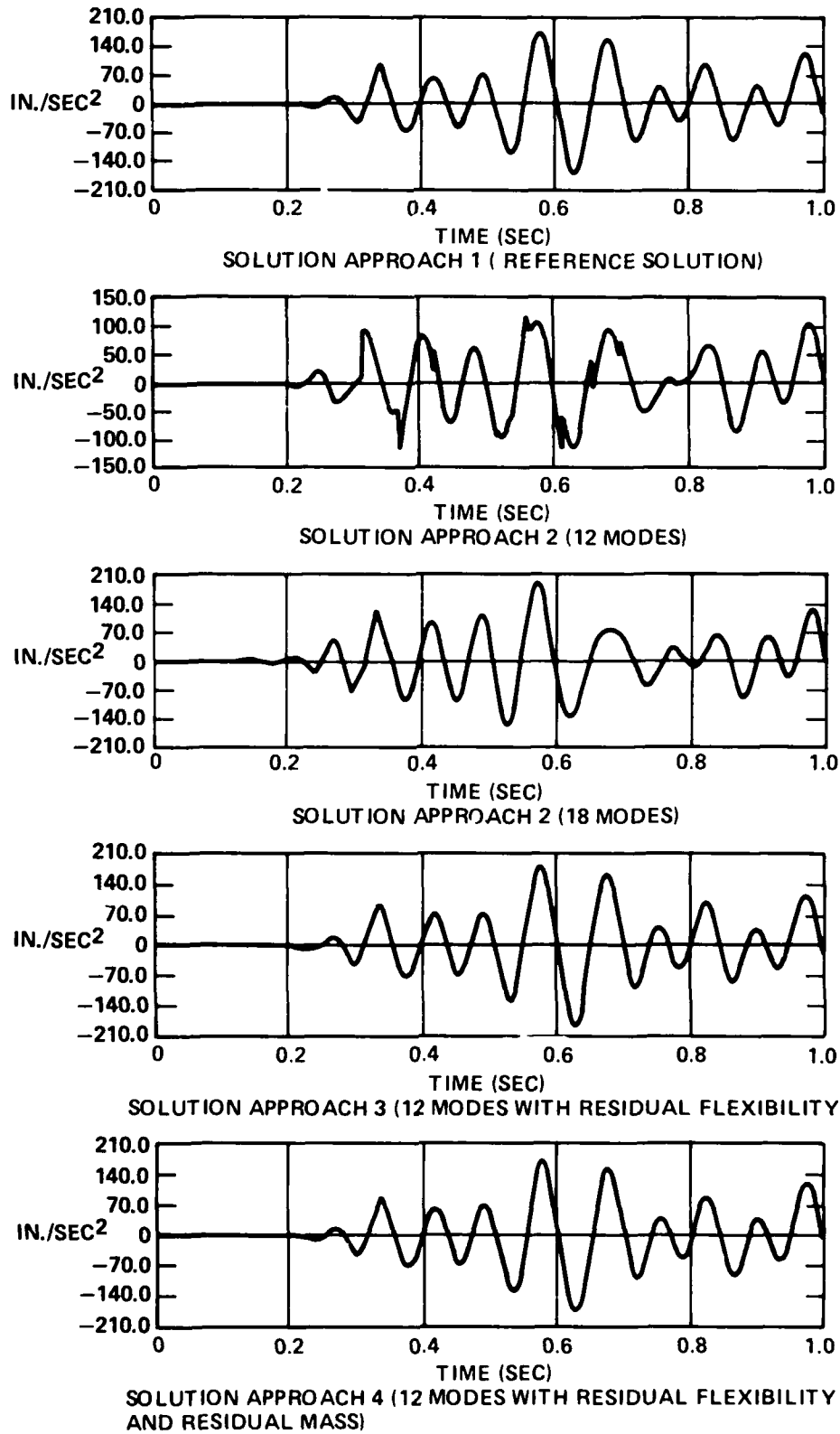
FIGURE 7. — ACCELERATION; 35
