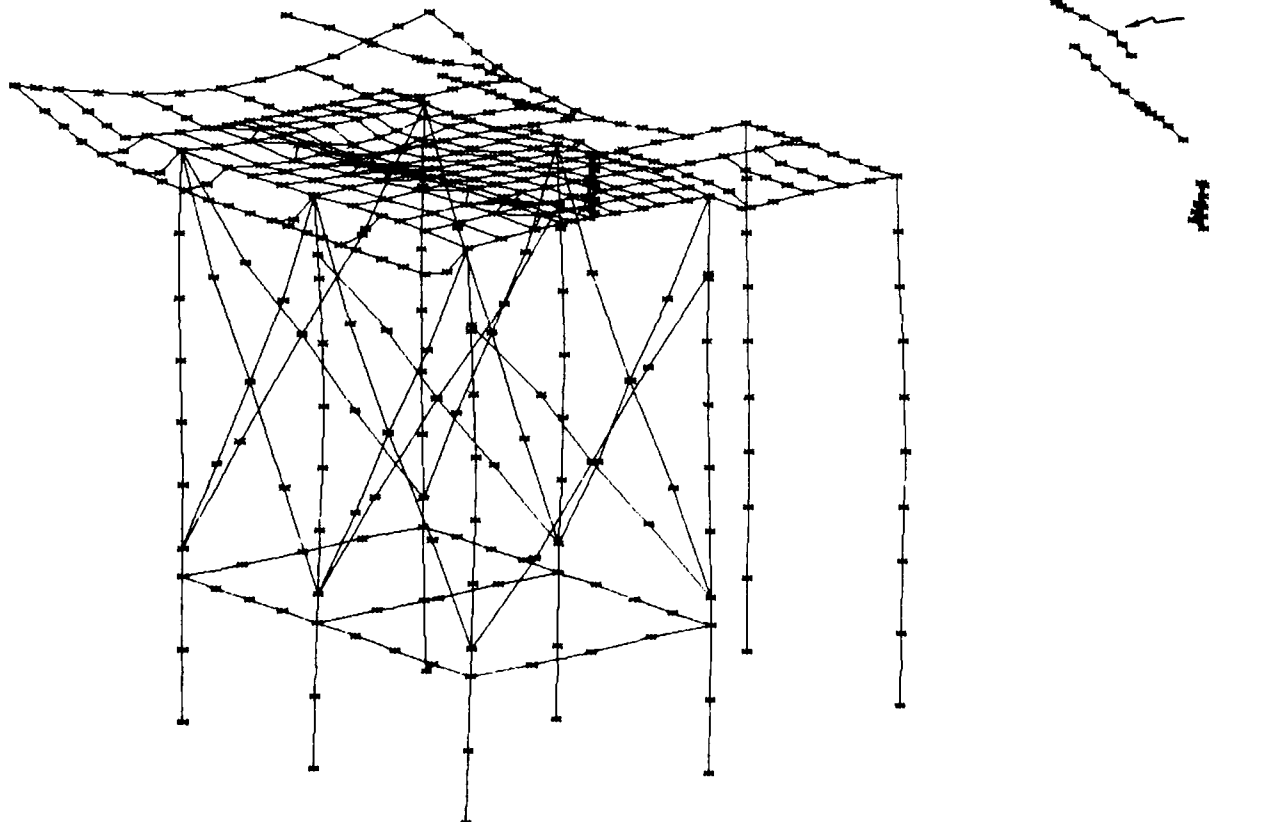
Figure 15: Mode B-23 (49.94 cps): West/North Grating Mode with Considerable Sole Plate Motion Near the Motor and Some Motor Shaft Deflection (Moderate to High Damage Potential)
