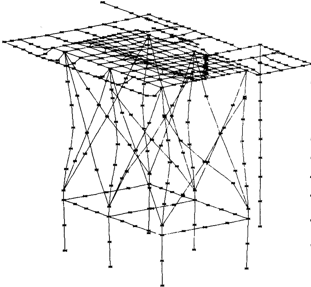
Figure 16: Mode B-46 (71.14 cps): Second Major Structural Mode Involving All Major Columns (High Damage Potential)
