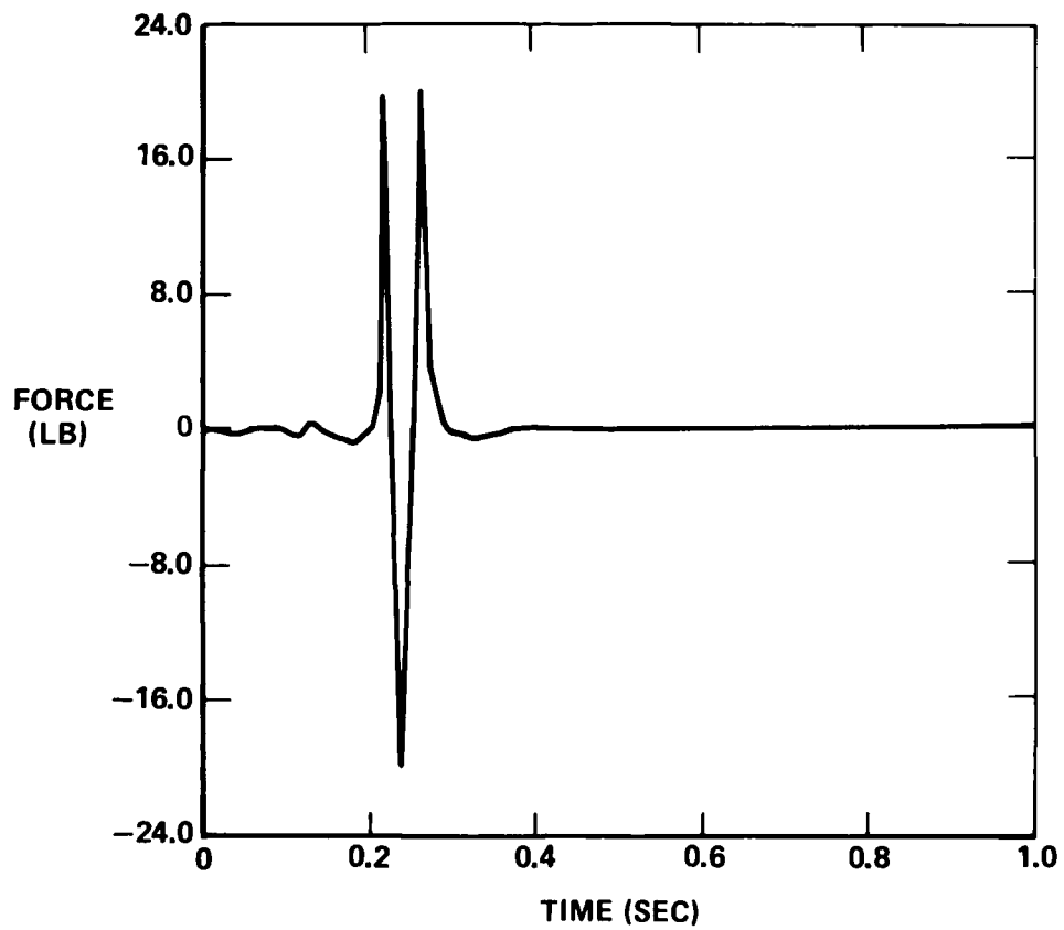
FIGURE 9. — FRICTION DEMONSTRATION PROBLEM WITH APPLIED FORCE; 7 DOF
