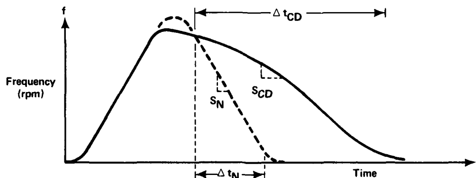
Figure 23: Possible Coast Down Curve
