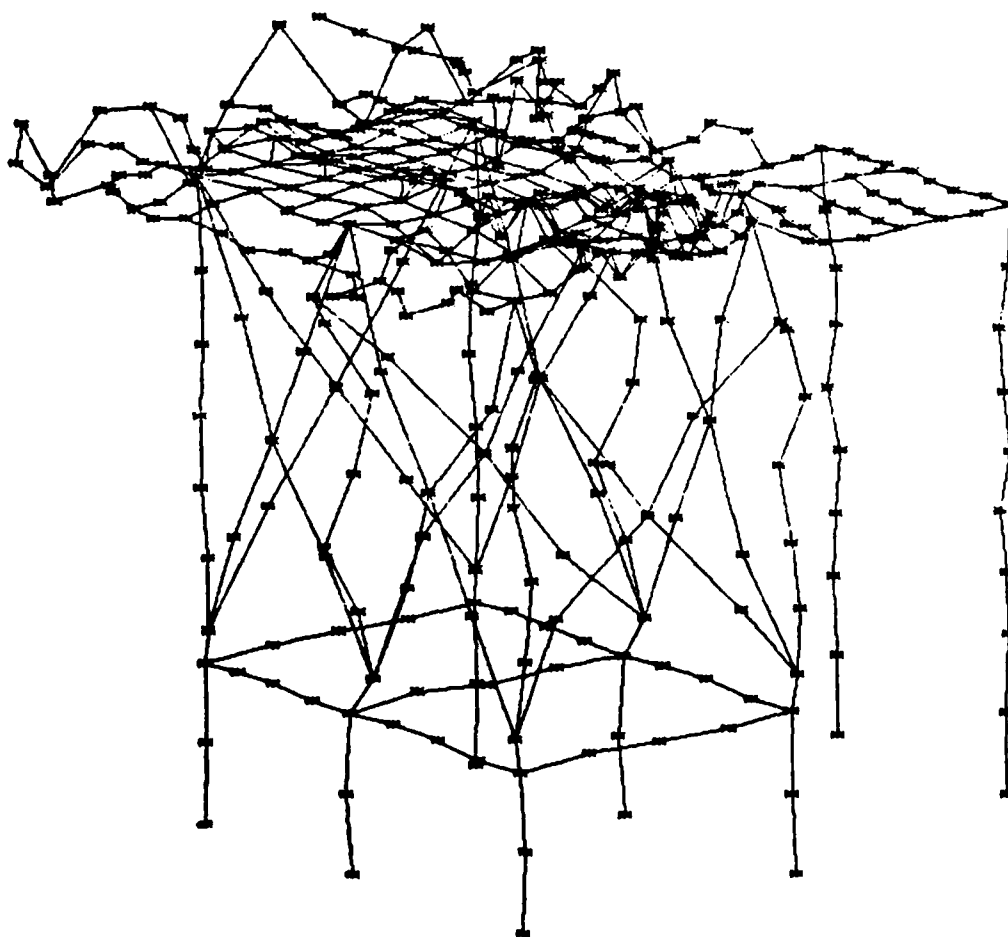
Figure 20: Mode 3-4 (831.16 cps): A Mode Involving Most of the Structure with Quite Severe Increases Shaft Deformation (High Damage Potential)
