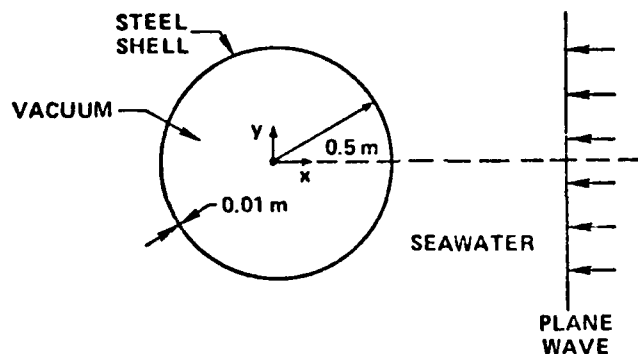
Figure 2 - Scattering from Infinite Cylindrical Shell
