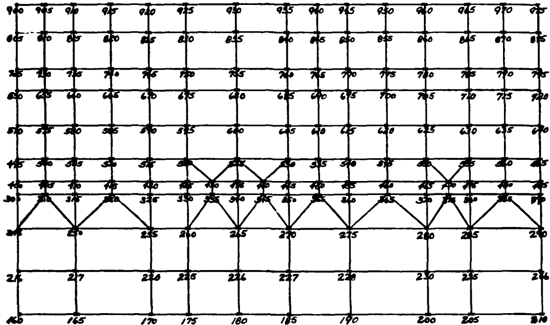
Figure A-3: Grid Point Layout for Sole Plate
