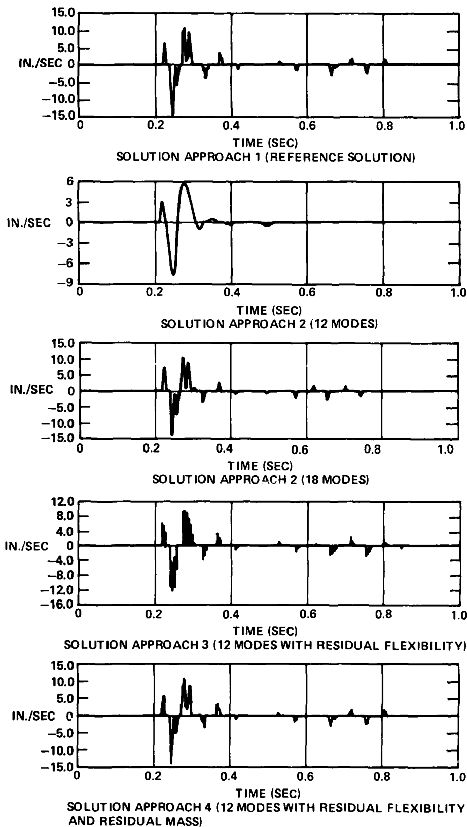
FIGURE 5. — RELATIVE VELOCITY; 17/27
