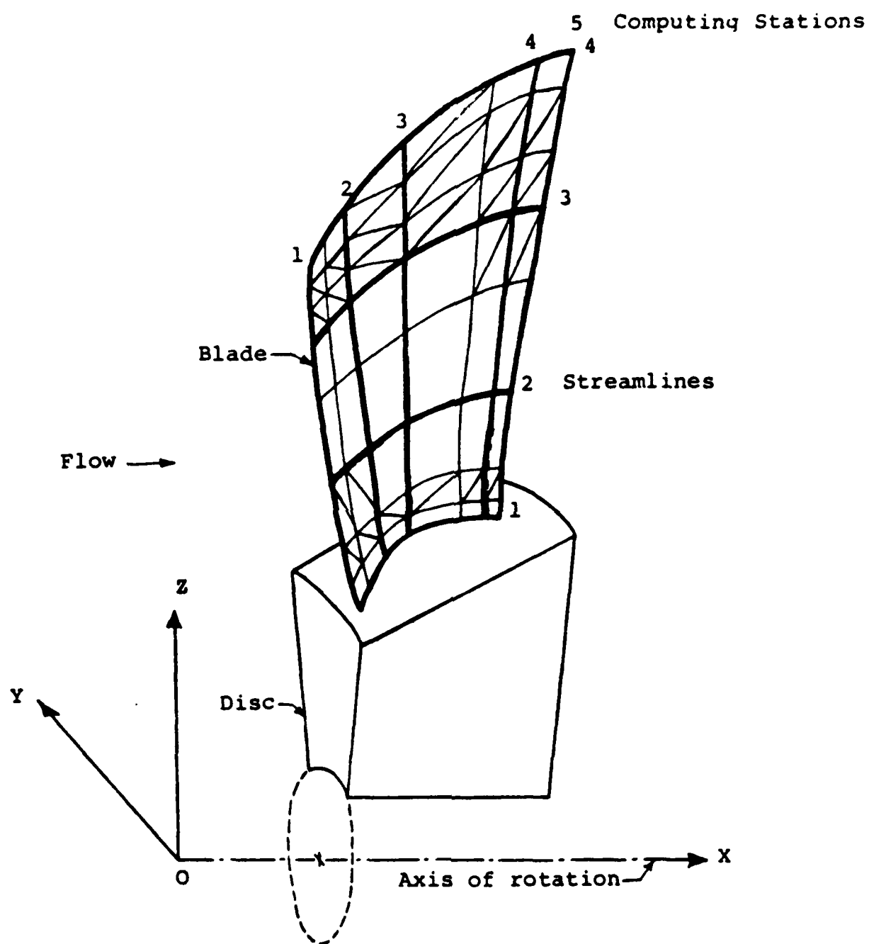
FIGURE 1. ROTATIONAL CYCLIC SECTOR OF A BLADED DISC
