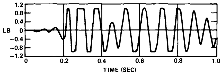
SOLUTION APPROACH 3 (12 MODES WITH RESIDUAL FLEXIBILITY)
