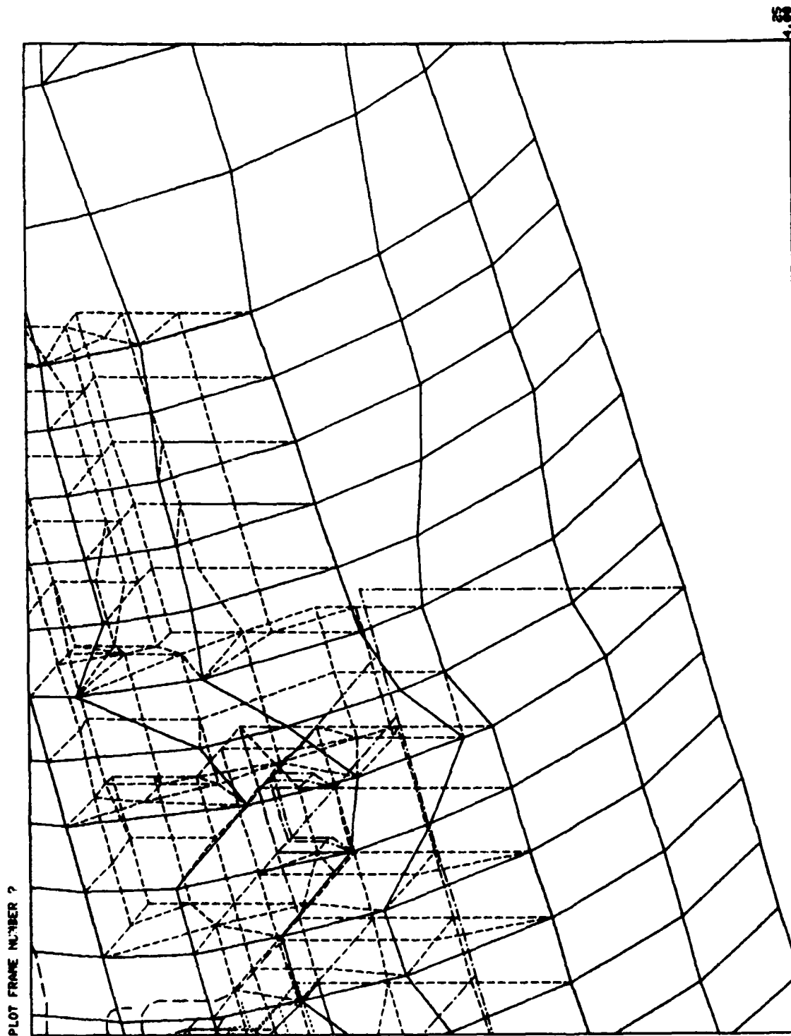
Figure 8 - Undeformed shape of structure plotted with dotted lines
