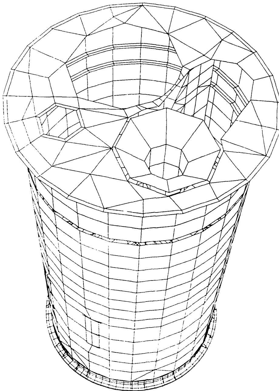
LARGE TEST MODEL - HIDDEN LINE PLOT
