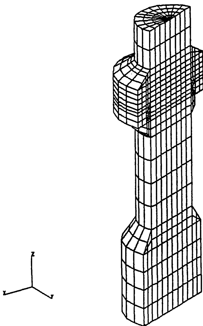
FIGURE 6 - HIDDEN LINE VIEW OF HMF BOLT, 22.5° PIE SECTION
