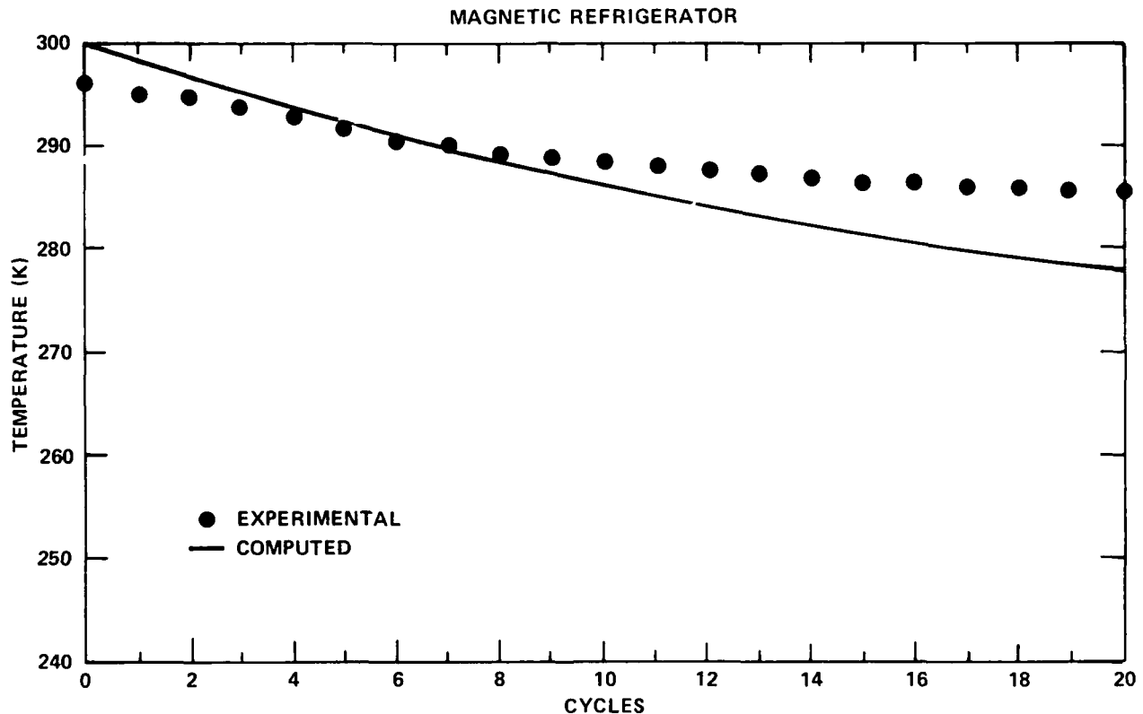
Figure 3. Comparison of Computed and Experimental Temperatures
