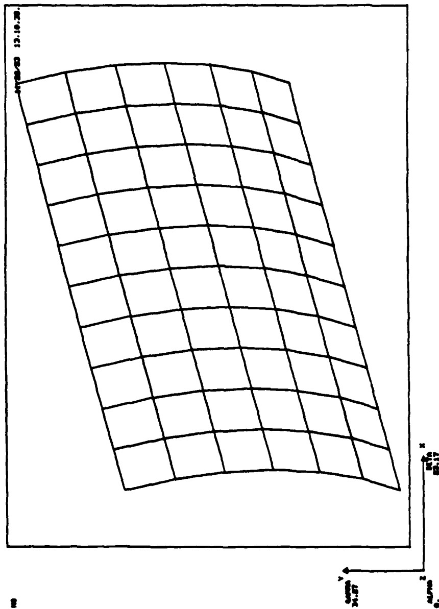
Figure 15 - NASTRAN finite element model for Panel 7, a curved panel. Refer to Table 2 for specific panel characteristics.
