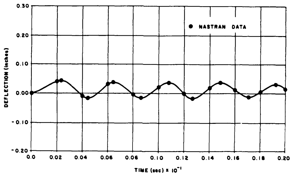
Figure 24 - NASTRAN analysis deflection.
