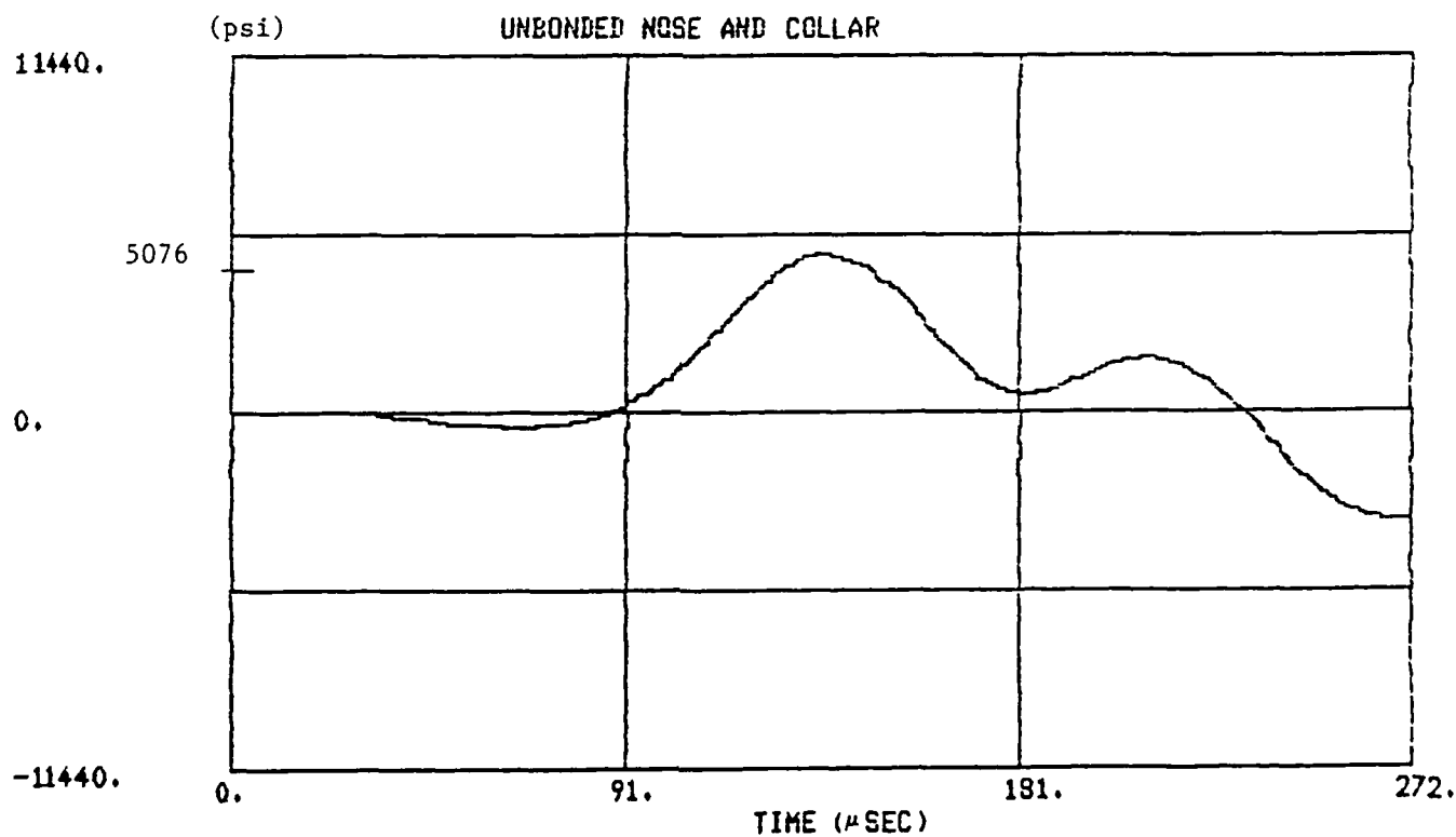
Figure 11 - Dynamic Axial Stresses (Element 105)
