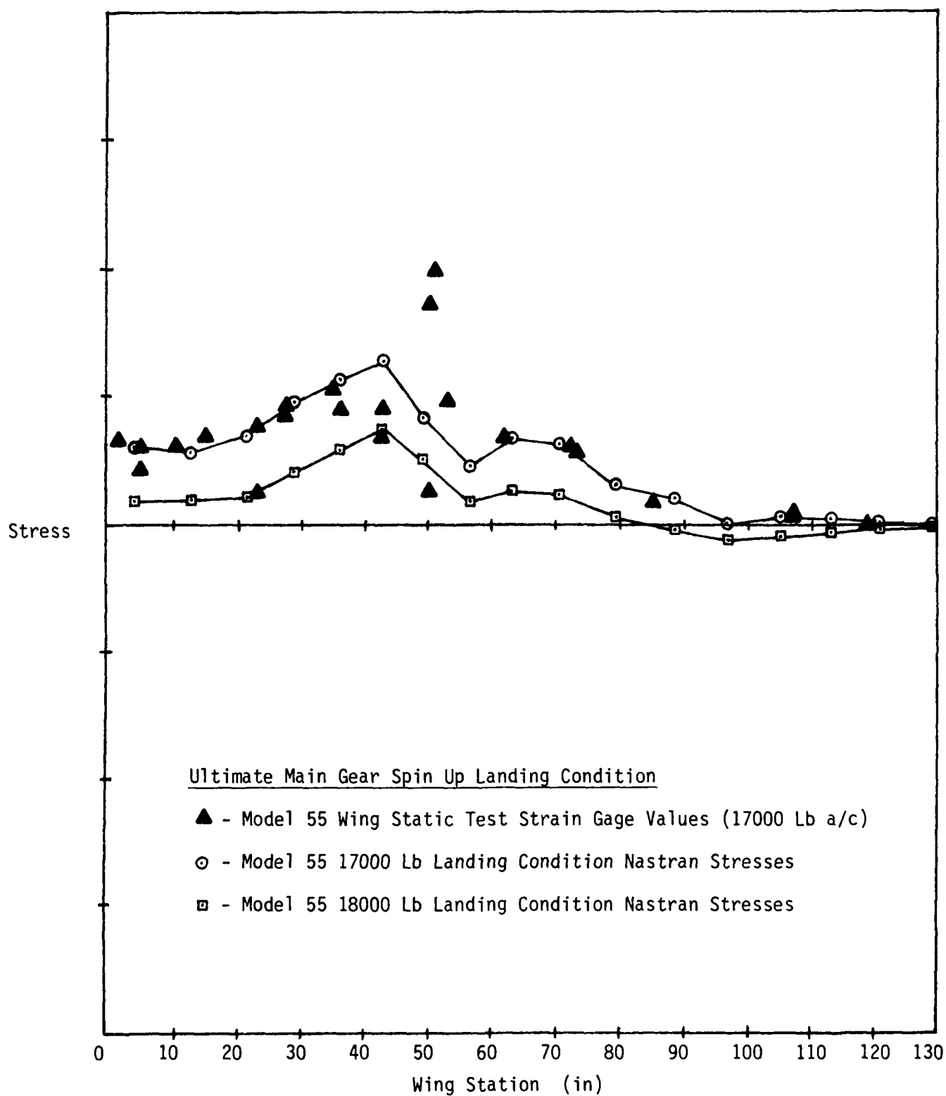
Figure 7 - Stresses In Spar 5 Lower Cap
