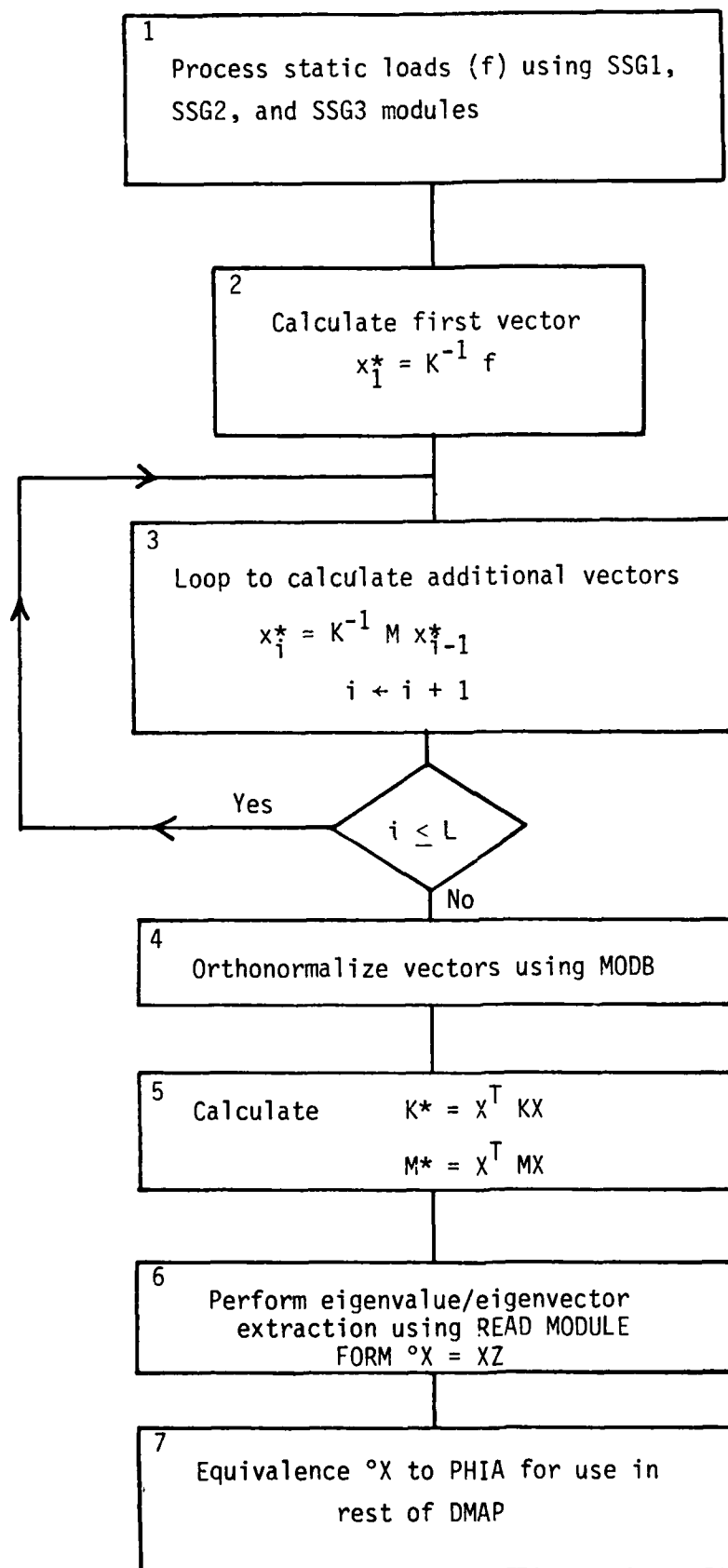
Figure 1 Flow Chart for Implementing Ritz Procedure into NASTRAN
