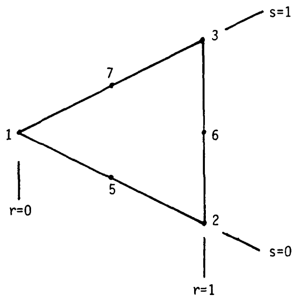
Figure 2 Degeneration of the Eight Node Element to a Six Node Triangular Element
