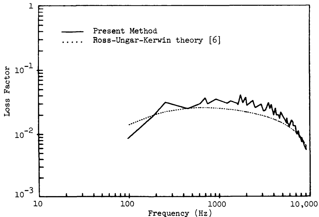
Figure 4 - Comparison of Loss Factors for Sandwich Plate as Predicted by Present Finite Element Method and by Ross-Ungar-Kerwin Theory [6]
