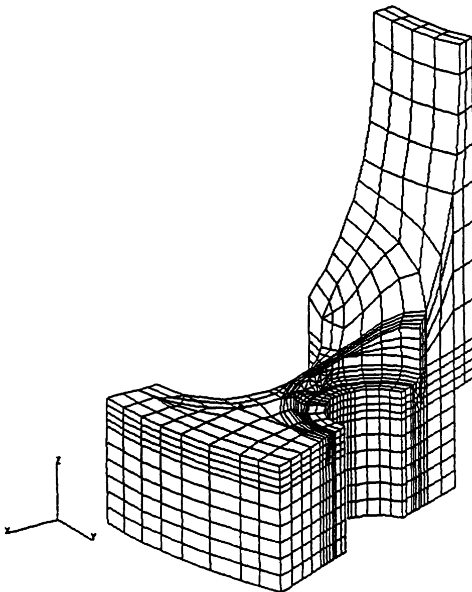
FIGURE 4 - HIDDEN LINE VIEW OF HMF PIN, 22.5° PIE SECTION
