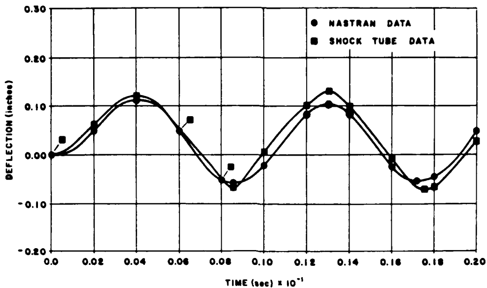
Figure 20 - NASTRAN versus shock tube deflections.
