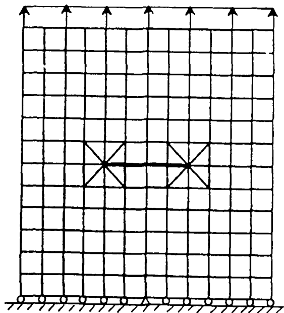
(b) loading condition for K_I calculation
