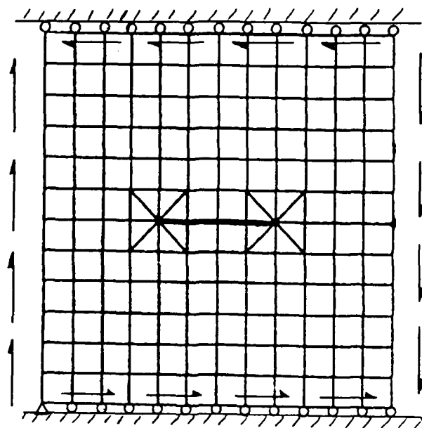
(a) loading condition for K_{II} calculation
