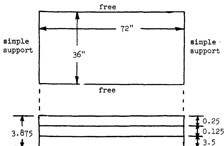
Figure 3 - Three-Layer Sandwich Plate Used for Calculating Loss Factors
