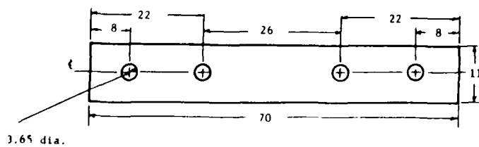
Figure 2. Plate geometry
