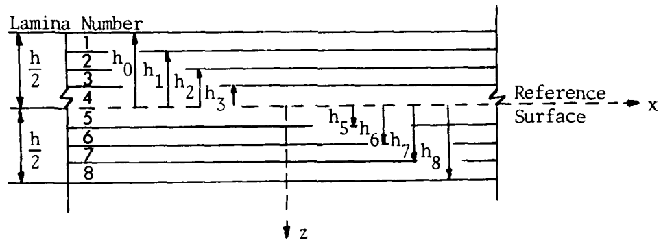
Figure 1. Laminated Plate
