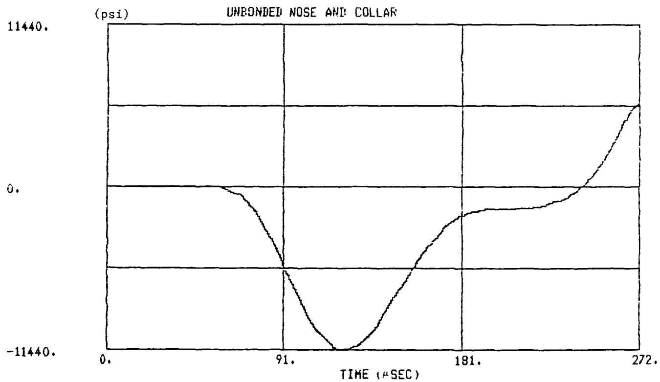
Figure 8 - Dynamic Hoop Stresses (Element 104)
