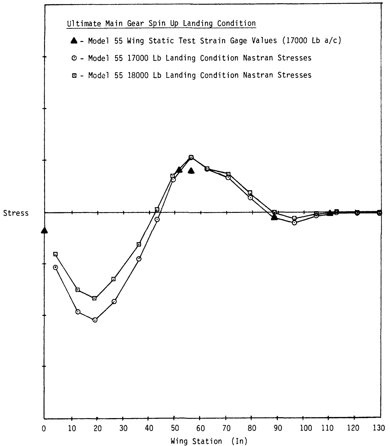
Figure 12 - Stresses In Spar 8 Upper Cap
