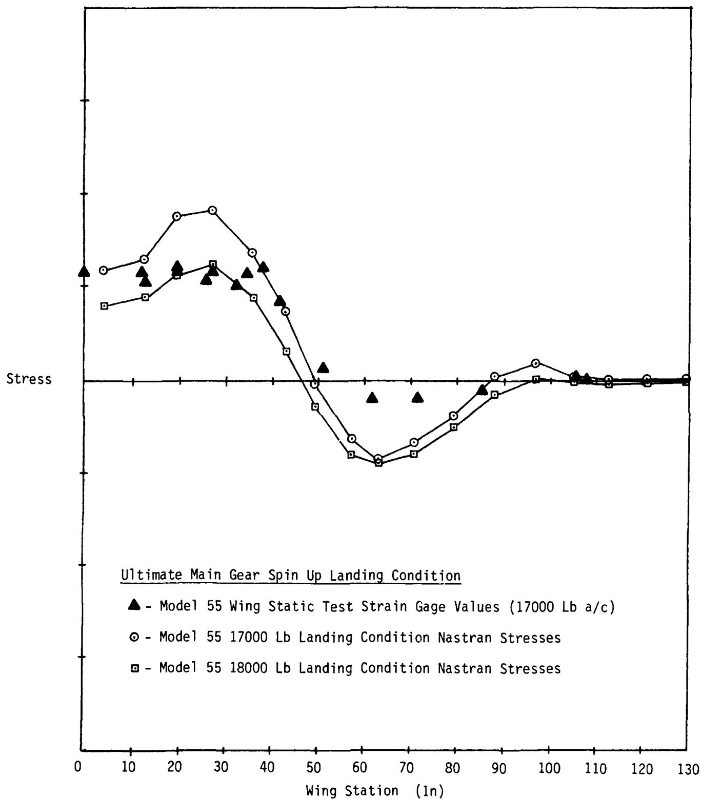
Figure 11 - Stresses In Spar 8 Lower Cap
