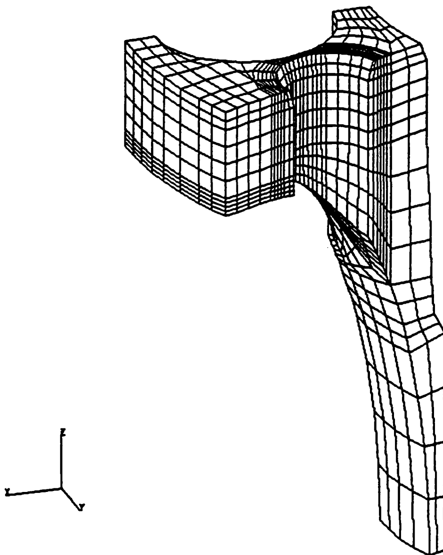
FIGURE 5 - HIDDEN LINE VIEW OF HMF BOX, 22.5° PIE SECTION
