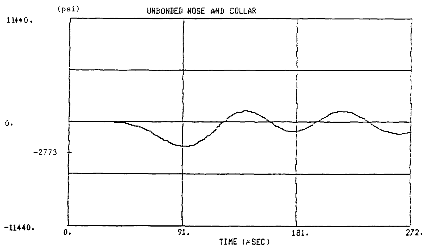
Figure 10 - Dynamic Hoop Stresses (Element 105)
