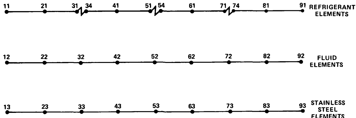
Figure 2. The Finite Element Model
