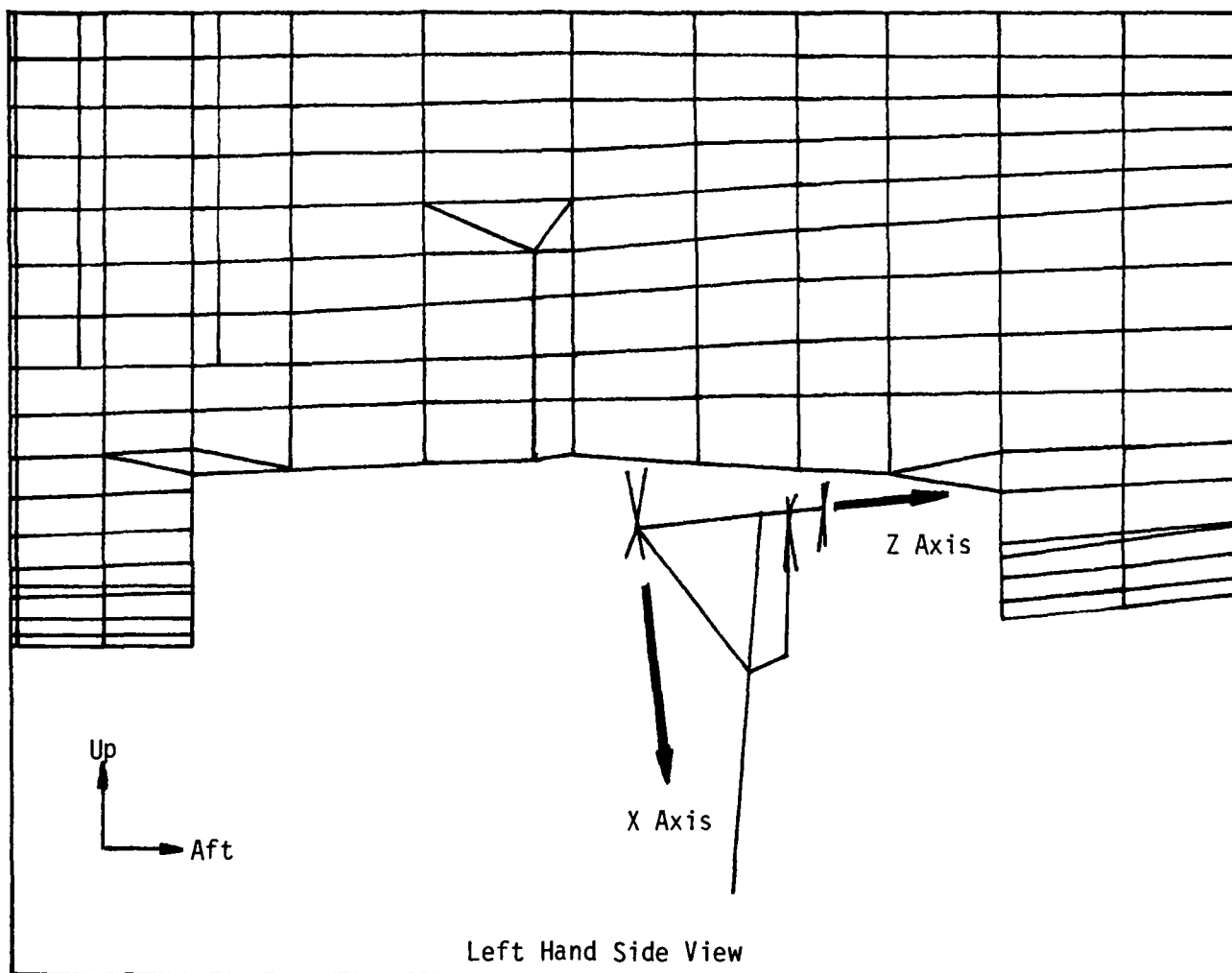
Figure 1 - Landing Gear Coordinate System
