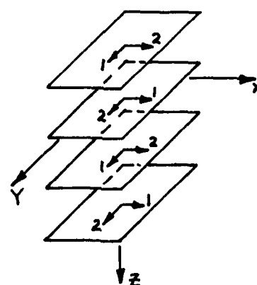
Figure 8. Simply Supported Composite Plate Example
