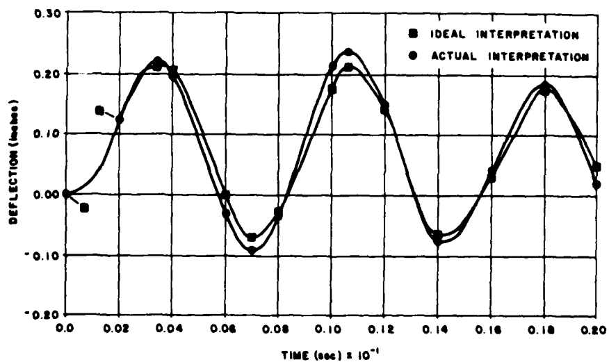
Figure 12 - Error effects study #3. Deflections resulting from pressures depicted in Figure 11.
