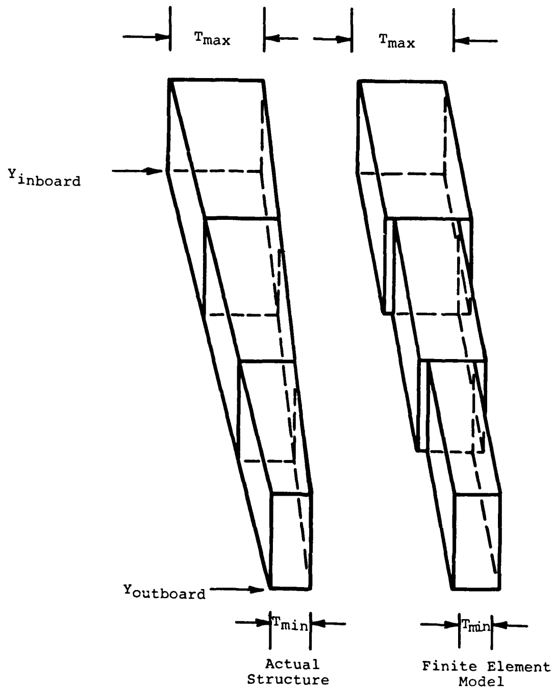
FIGURE 2 SKIN TAPERING
