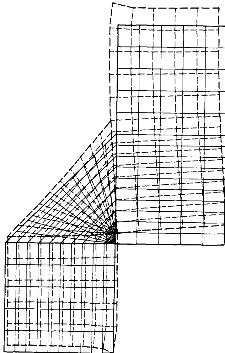
FIGURE 3 DEFORMED GEOMETRY, CASE I
