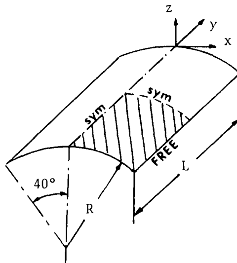
Figure 7. Rectangular Plate
