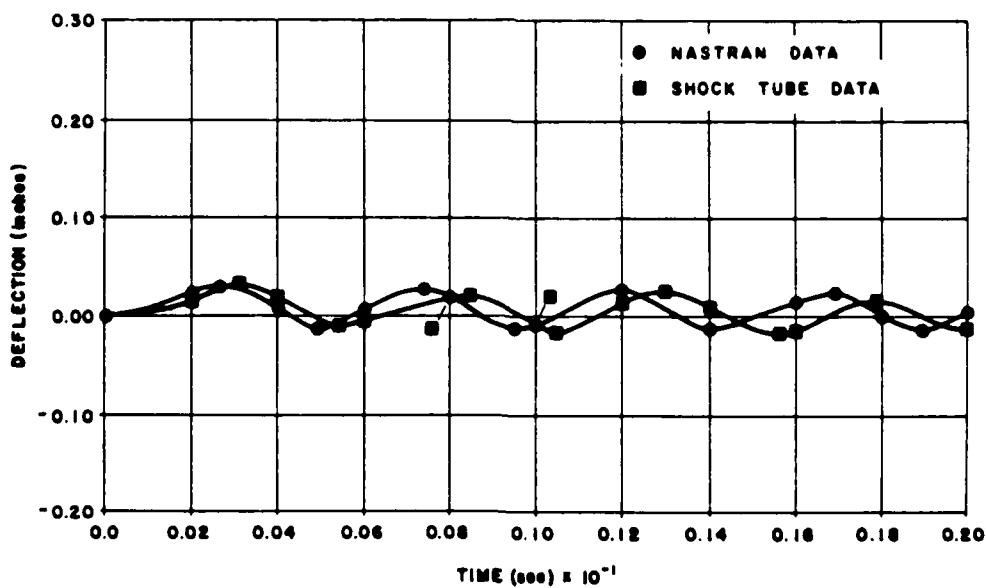
Figure 21 - NASTRAN versus shock tube deflections.
