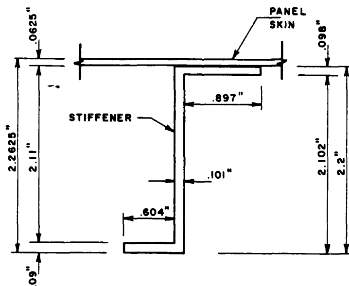
PANEL 6 STIFFENER CROSS SECTION
