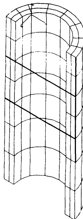
Figure 3. 180 degree model
