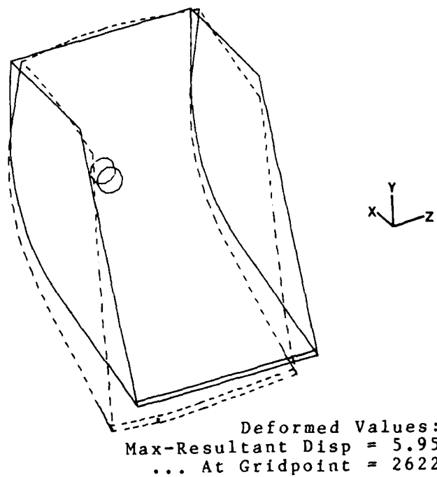
FIGURE 18 FORE-AFT CONSTRAINTS
