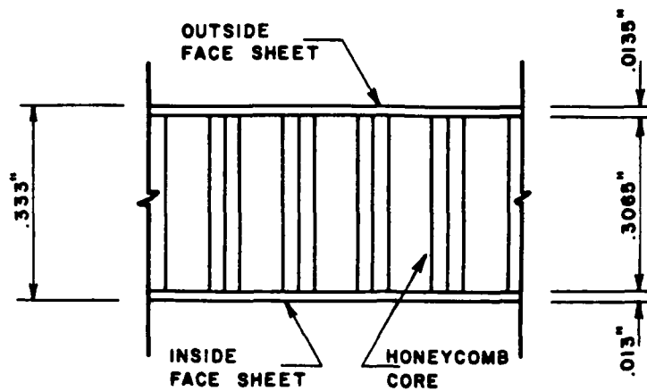
PANEL 5 CROSS SECTION
