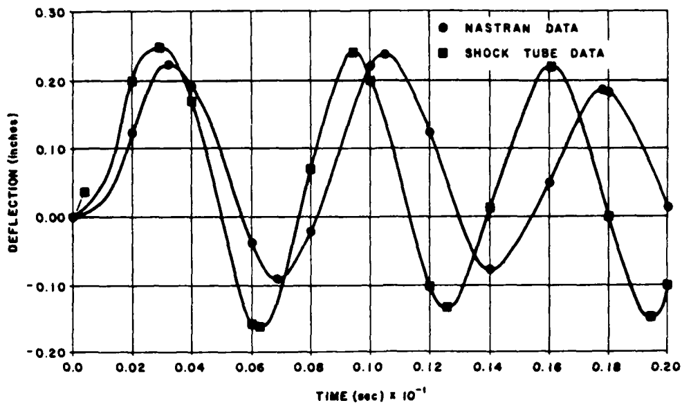
Figure 18 - NASTRAN versus shock tube deflections.
