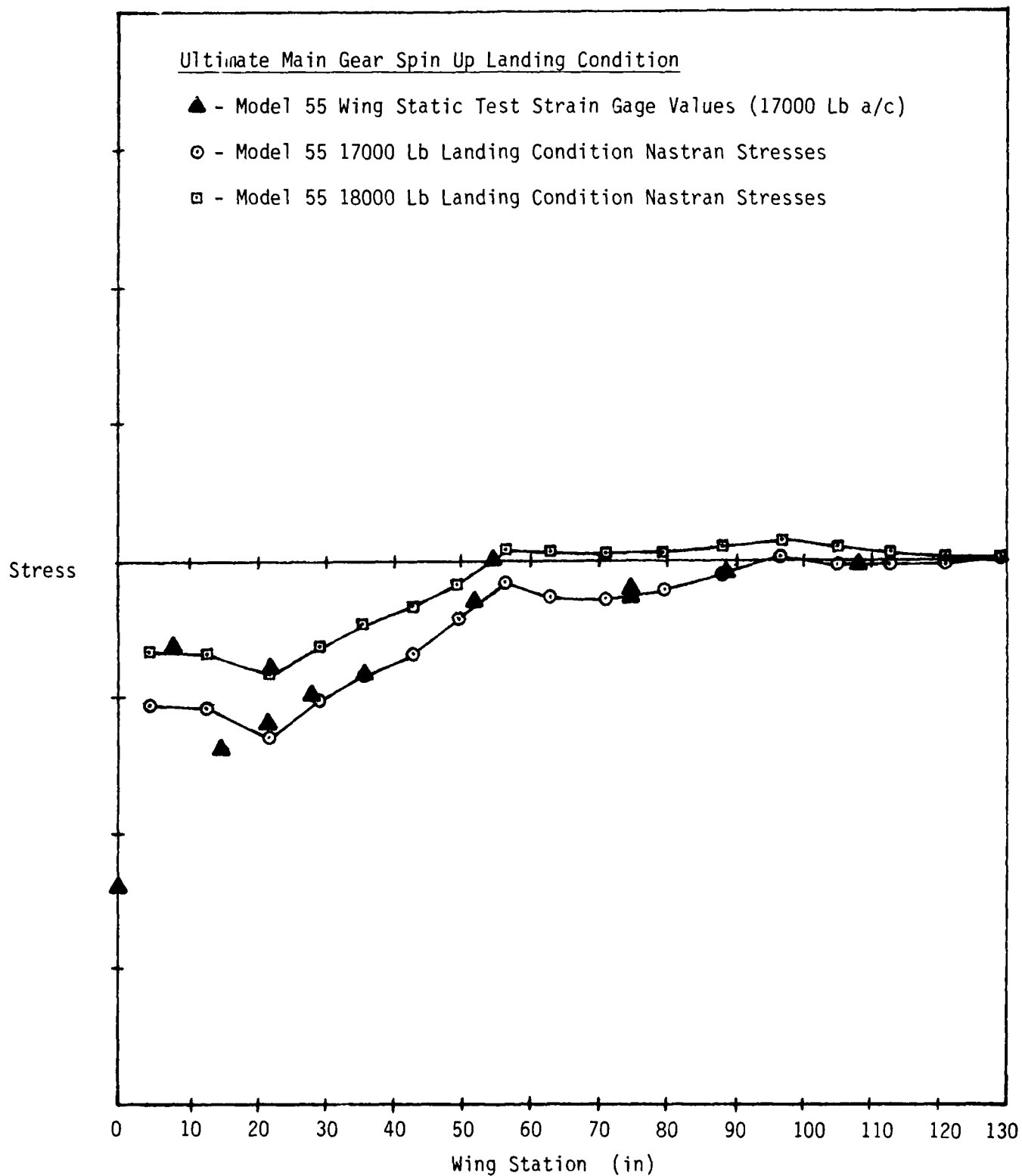
Figure 8 - Stresses In Spar 5 Upper Cap
