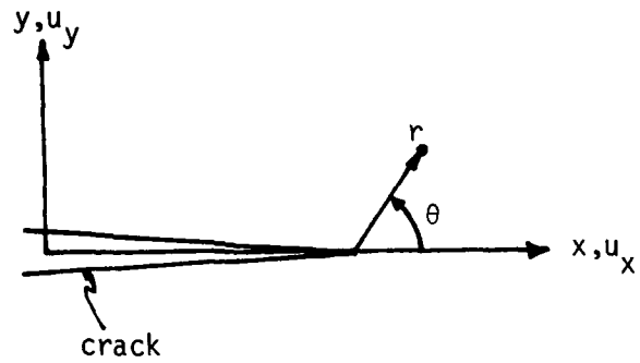
Figure 3 Nomenclature for Crack Geometry
