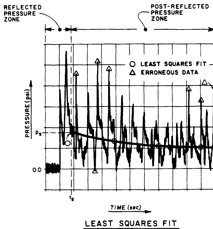
Figure 3 - Approximated least squares fit on a typical plot of experimental post-reflected data.
