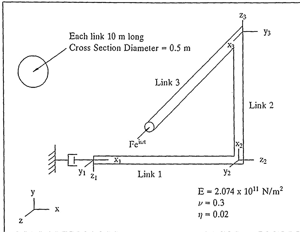
Fig. 3. Test Problem Geometry
