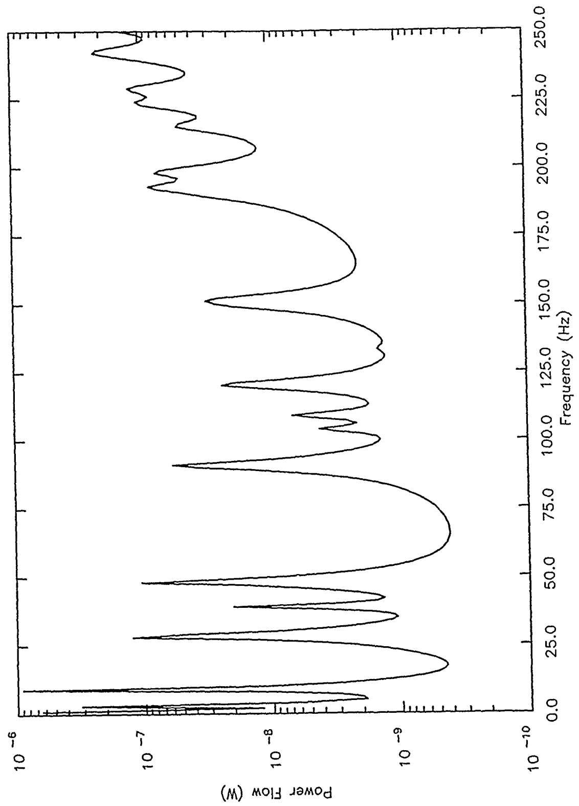
Fig. 4. Power inputs for test problem.
