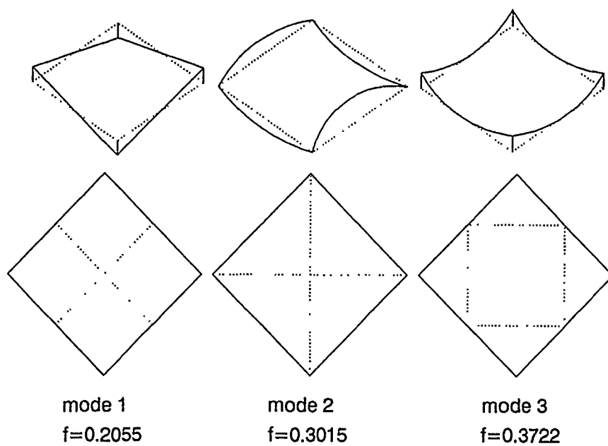
Figure 1. Mode shapes and frequencies (Hz) for flat plate.
