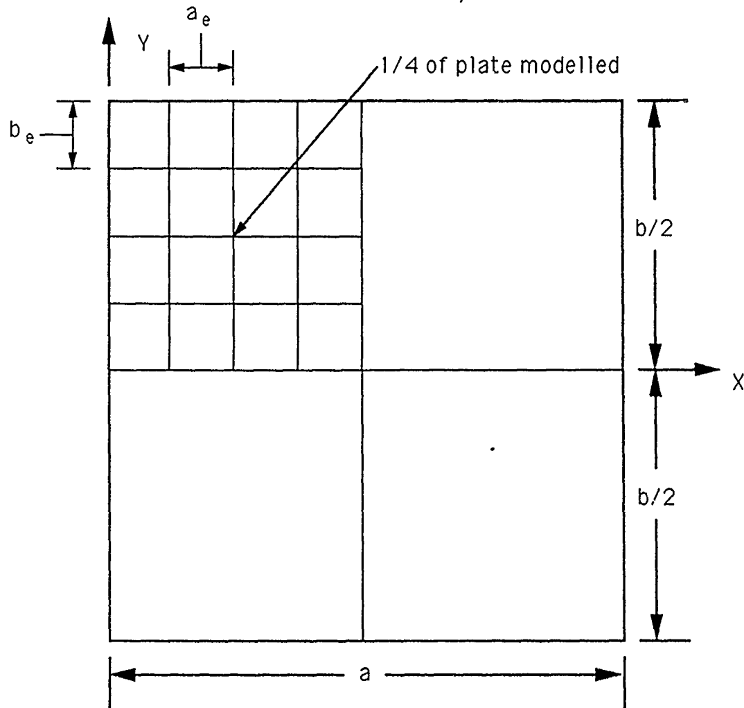
Fig. 2 Mesh Geometry
