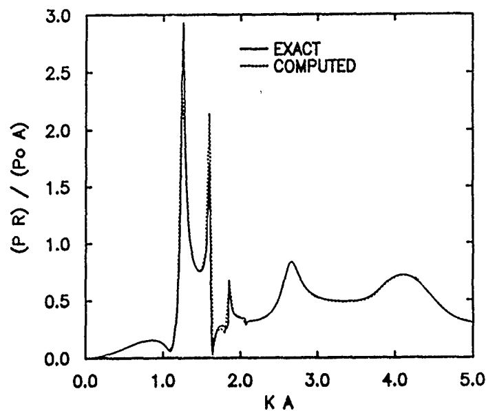
Fig. 4. Backward Scattering from a Fluid-Filled Spherical Shell
