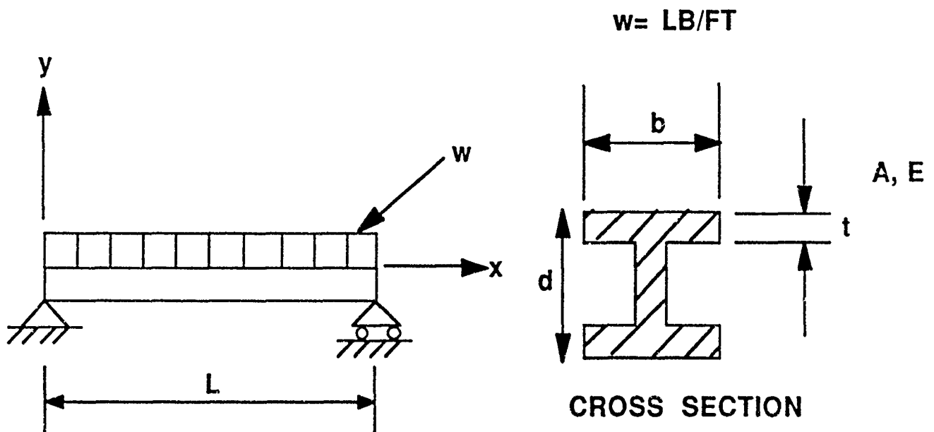
Figure 5. Simply Supported Beam with Uniformly Distributed Mass (Example 2)
