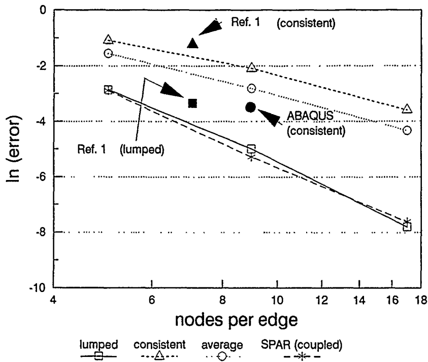
Figure 7. Frequency convergence for mode n=6 , n=1 of a cylindrical shell as a function of mesh density for different finite elements.
