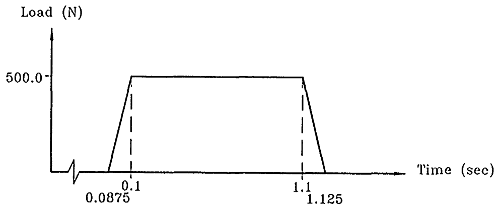
Fig. 3 Sample 2 - Load vs. Time
