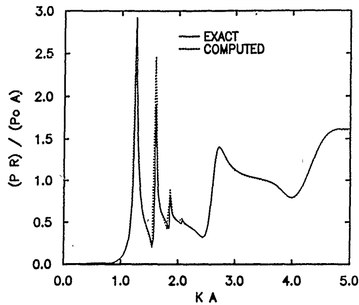
Fig. 3. Forward Scattering from a Fluid-Filled Spherical Shell
