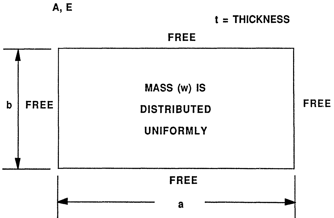
Figure 9. Rectangular Plate Free on All Sides (Example 6)
