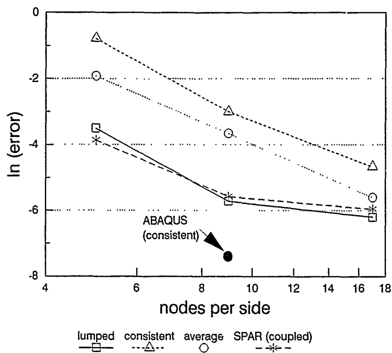
Figure 3. Frequency convergence for mode 2 of a flat plate as a function of mesh density for different finite elements.
