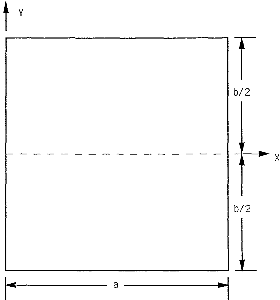
Fig. 1 Test Problem
