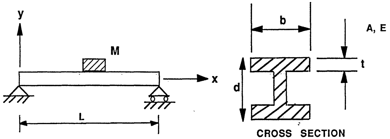
Figure 4. Simply Supported Beam with Concentrated Mass (Example 1)
