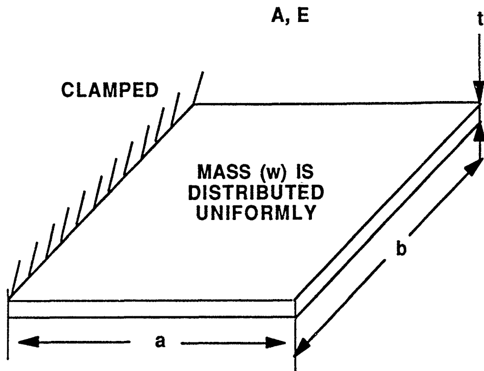
Figure 8. Rectangular Plated Clamped at One Edge (Example 5)
