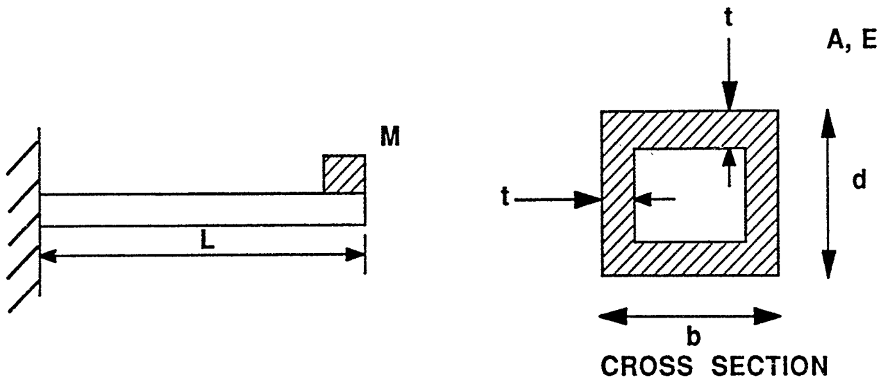
Figure 6. Cantilever Beam with Concentrated Mass (Example 3)
