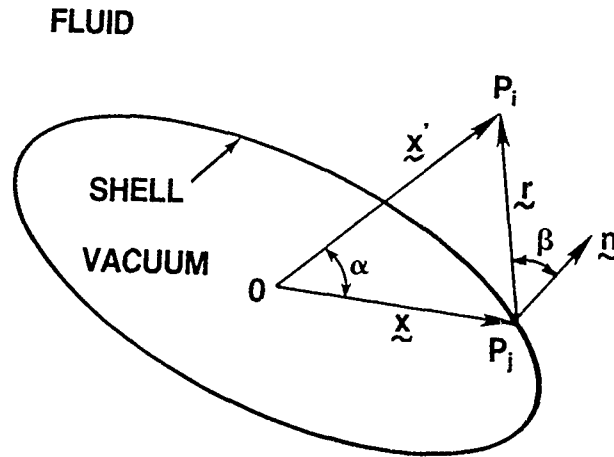
Fig. 1. Notation for Helmholtz Integral Equation
