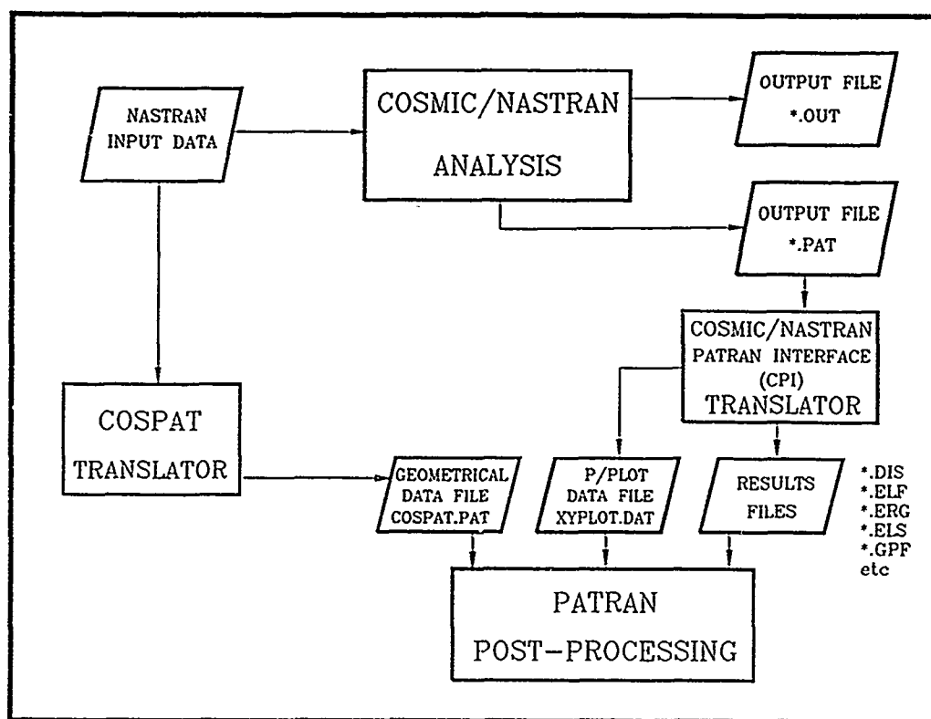
Fig. 1 Code and File Relationships
