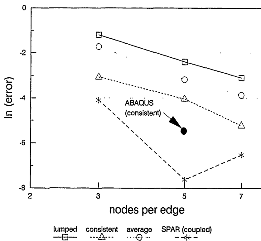
Figure 2. Frequency convergence for mode 1 of a flat plate as a function of mesh density for different finite elements.
