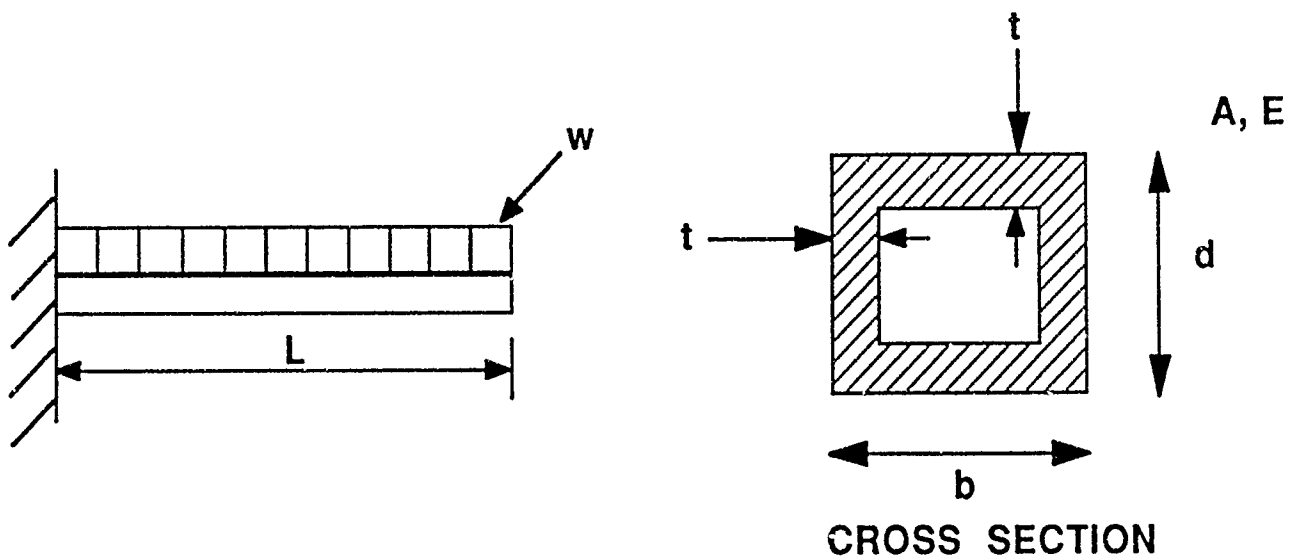
Figure 7. Cantilever Beam with Uniformly Distributed Mass (Example 4)
