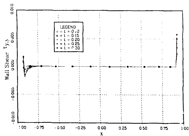
Fig.6 Lee-side crosswise skin friction \tau_{y,y} ( \hat{\alpha} = 0^\circ ).
