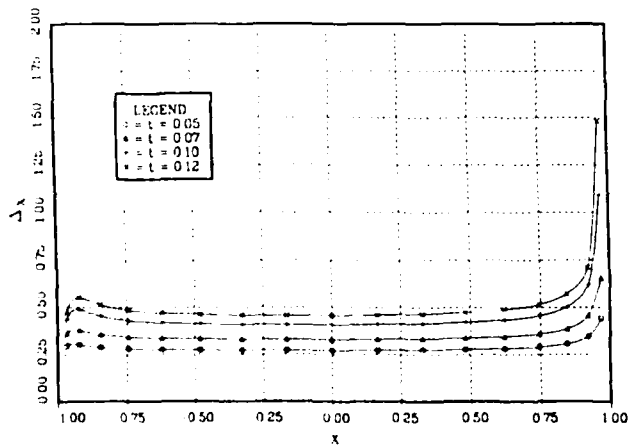
Fig.18 Lee-side displacement thickness \bar{\Delta x} ( \hat{\alpha} = 50^\circ ).
