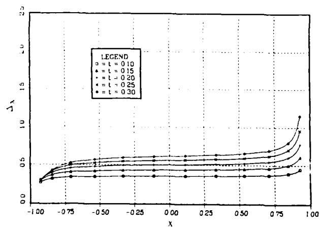
Fig.7 Lee-side displacement thickness \Delta_x ( \hat{\alpha} = 0^\circ ).
