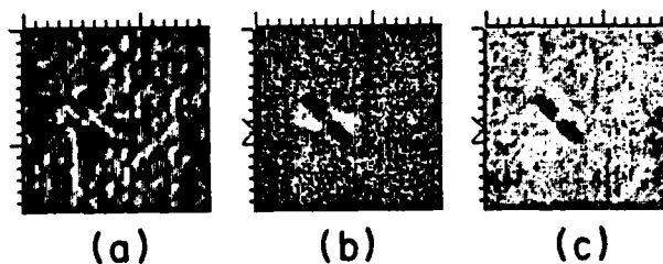
Fig. 3. C-scan images: (a) from rectified and filtered A-scan; (b) from rf A-scan; (c) from deconvolved A-scan.
