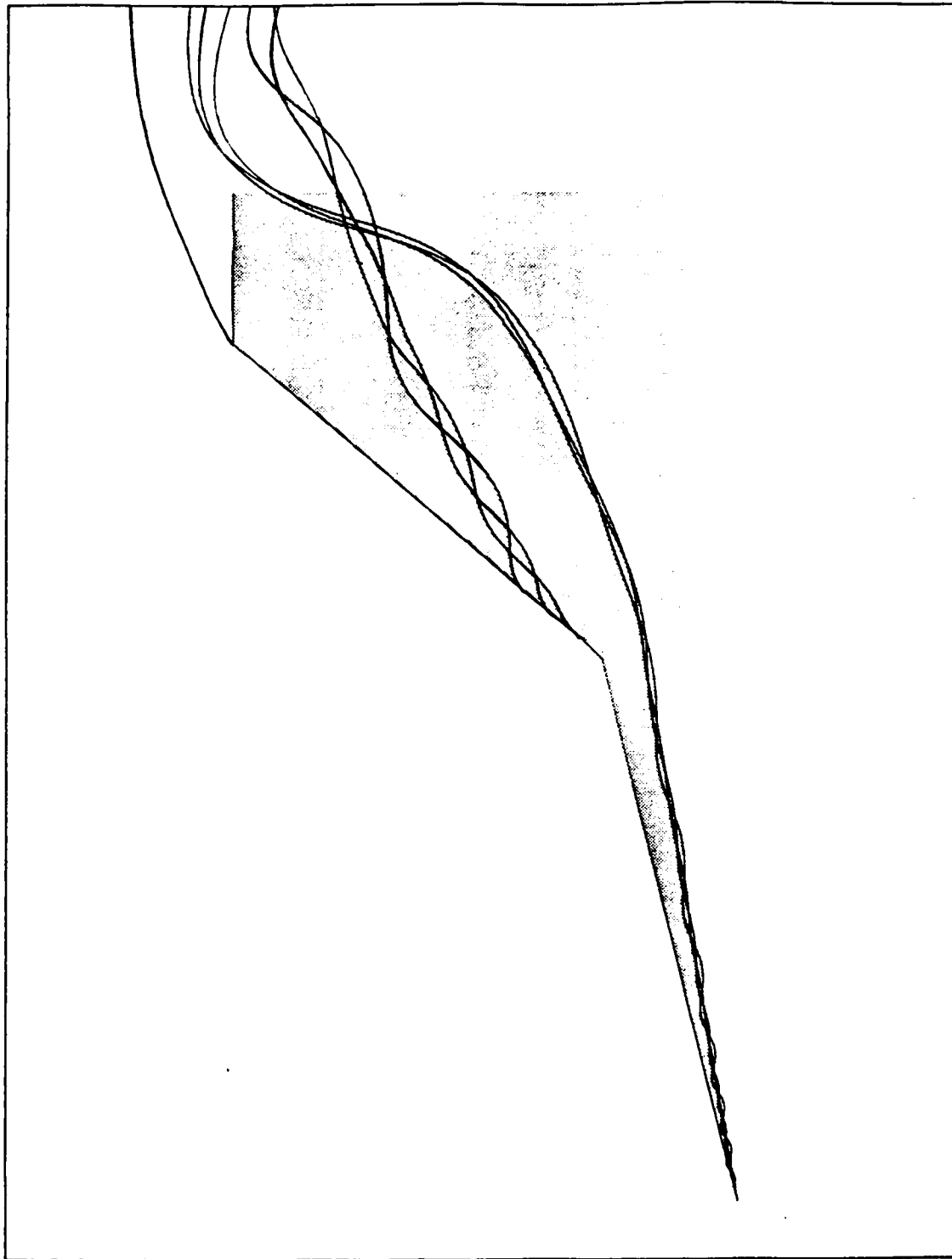
Figure 64. Particle Traces at 19^\circ - M = 0.22 , Re = 3.8 \times 10^6 , (70x63x68)
