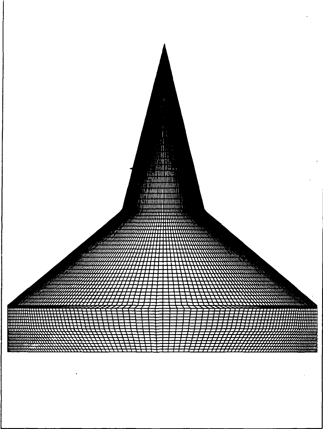
Figure 9. Double-Delta Wing - top view (100x240x1)
