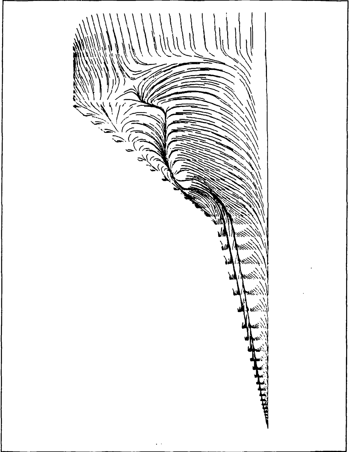
Figure 69. Surface Flow Pattern at 22.4^\circ - M = 0.22 , Re = 3.8 \times 10^6 , (70 \times 63 \times 68)
