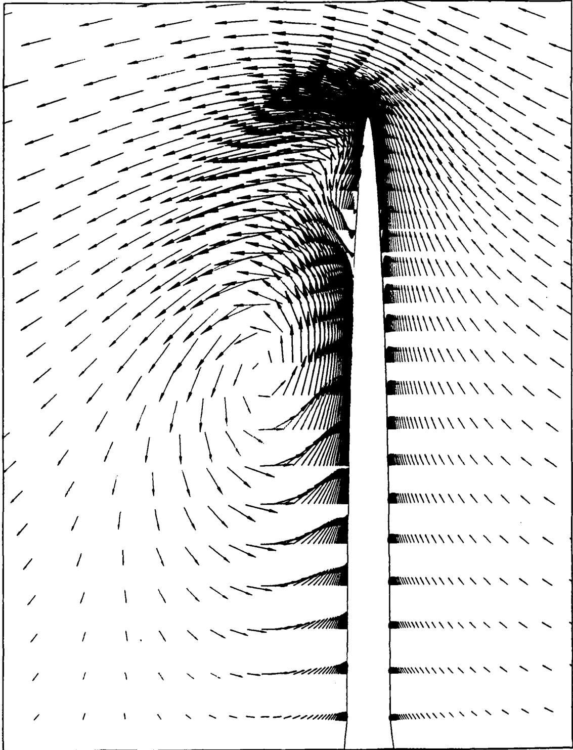
Figure 73. Wing Velocity Vectors at 22.4^\circ - M = 0.22 , Re = 3.8 \times 10^6
