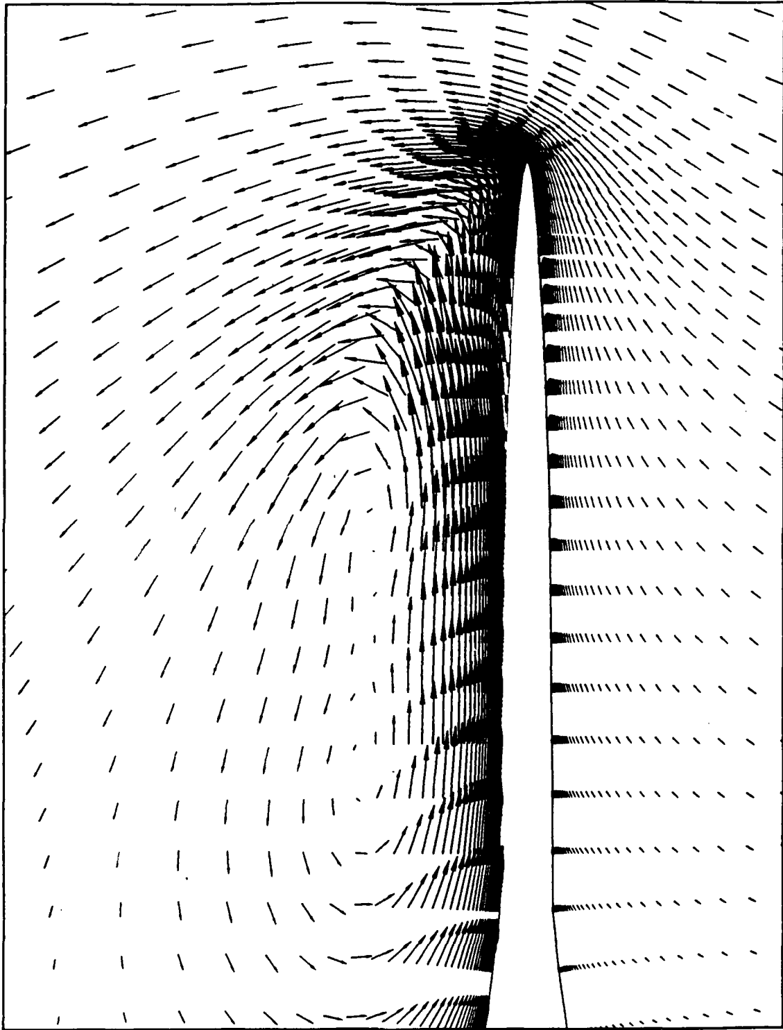
Figure 67. Wing Velocity Vectors at 19^\circ - M = 0.22 , Re = 3.8 \times 10^6
