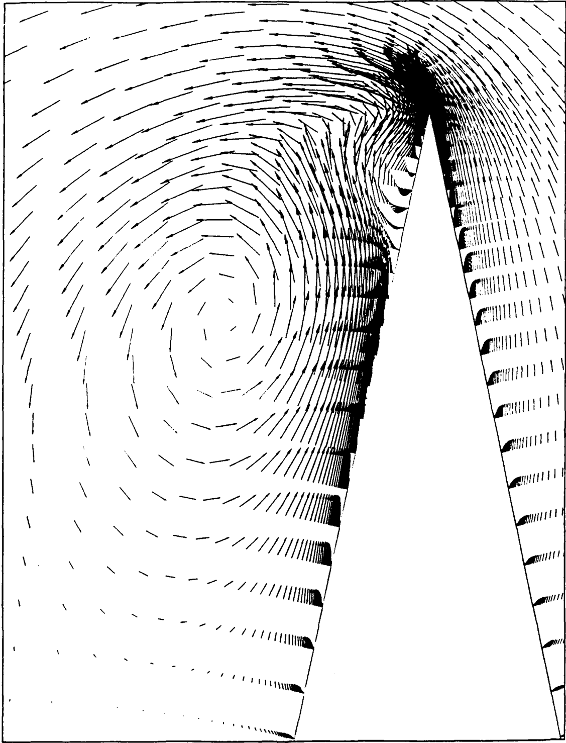
Figure 60. Strake Velocity Vectors at 10^\circ - M = 0.22 , Re = 3.8 \times 10^6
