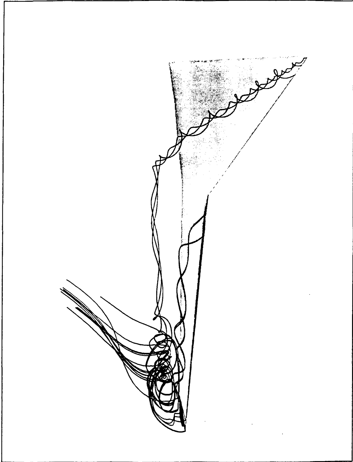
Figure 71. Vortex Location at 22.4° - M = 0.22 , Re = 3.8 \times 10^6 , (70x63x68)
