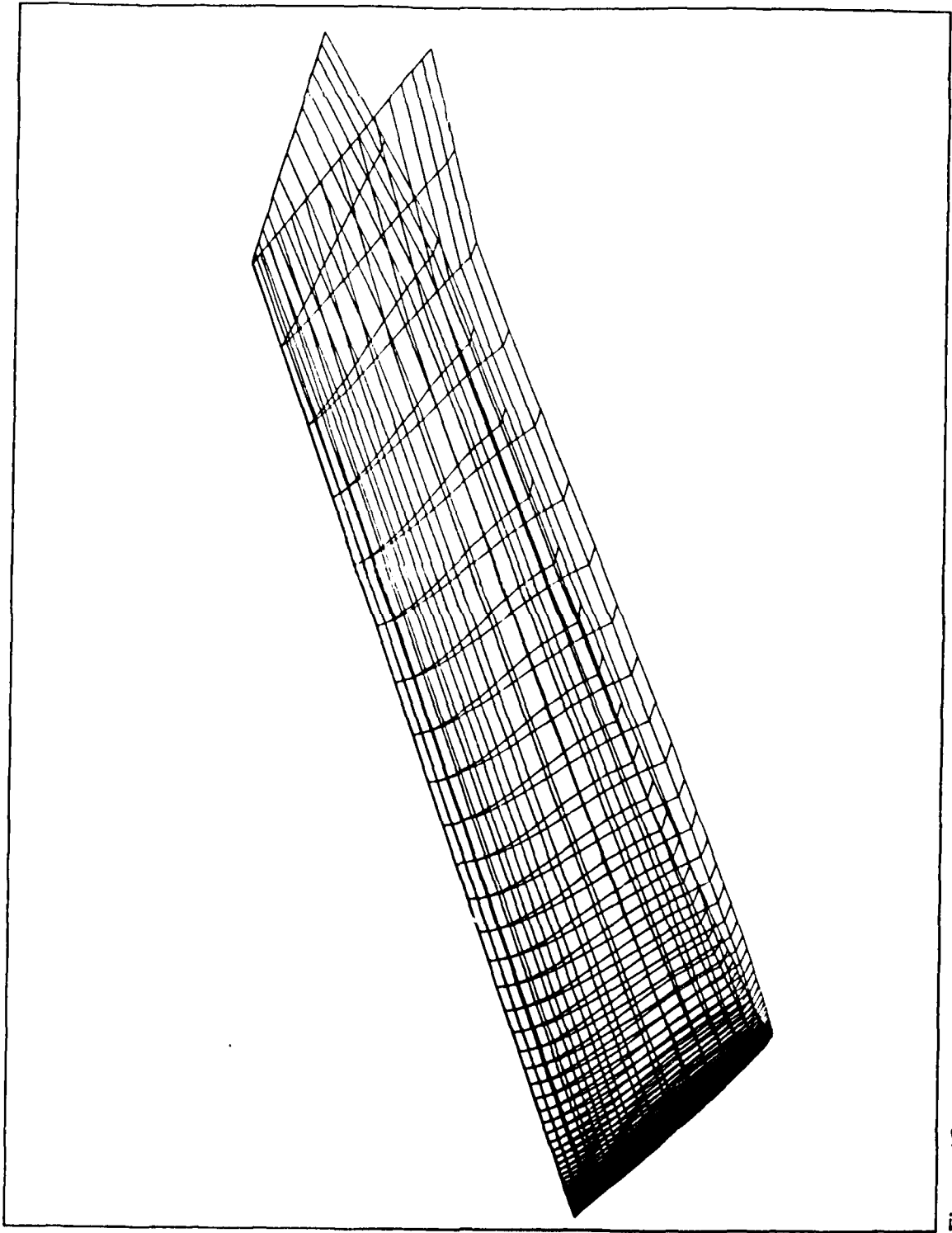
Figure 18. Grid Distribution of the Rectangular Section (16x240x1)
