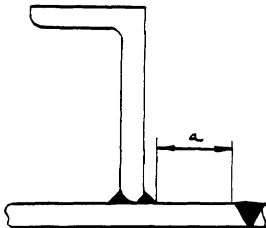
Figure 10: DISTANCE BETWEEN BUTT WELD AND FILLET WELD
