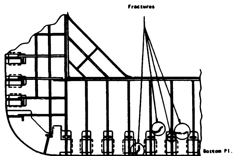
Figure 15: TRANSVERSE WEB FRAME AT BOTTOM
