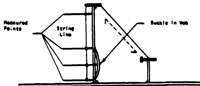
Figure 21: BUCKLING OF CENTERLINE GIRDER
