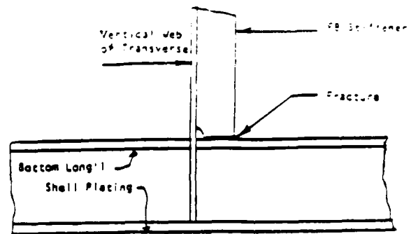
Figure 19: FRACTURE IN BOTTOM TRANSVERSE WEB
