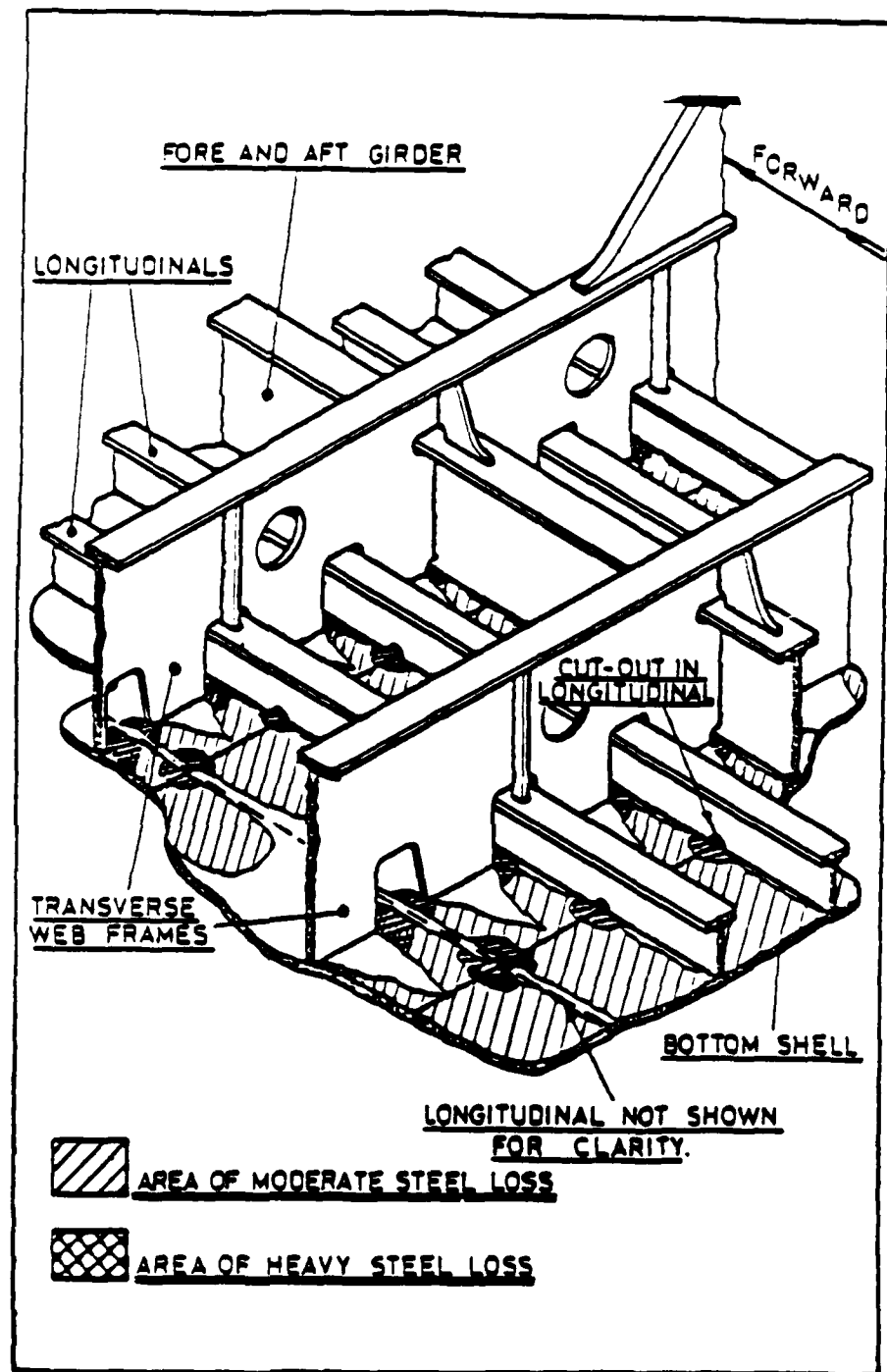
Figure 22: TYPICAL BOTTOM SHELL LOSS PATTERNS
