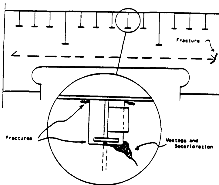
Figure 14: HORIZONTAL STRINGER IN WING TANKS
