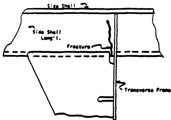
Figure 17: SIDE SHELL LONGITUDINAL FRACTURE
