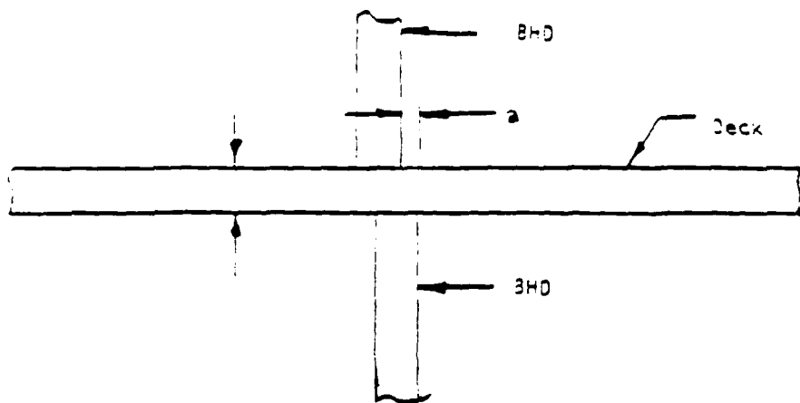
Figure 4: BULKHEAD MISALIGNMENT
