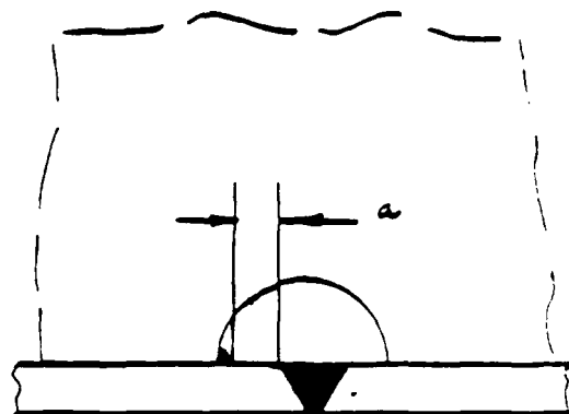
Figure 8: DISTANCE BETWEEN BUTT WELD AND SCALLOP
