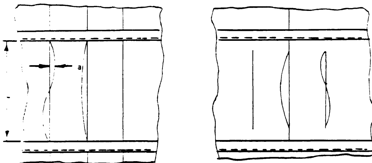
Figure 11: DISTORTION OF BEAMS, FRAMES, STIFFENERS
