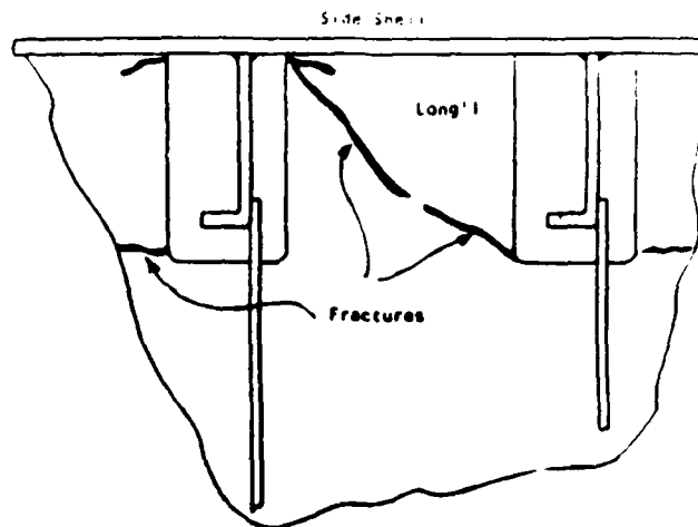
Figure 16: TRANSVERSE WEB FRAME AT SIDE SHELL
