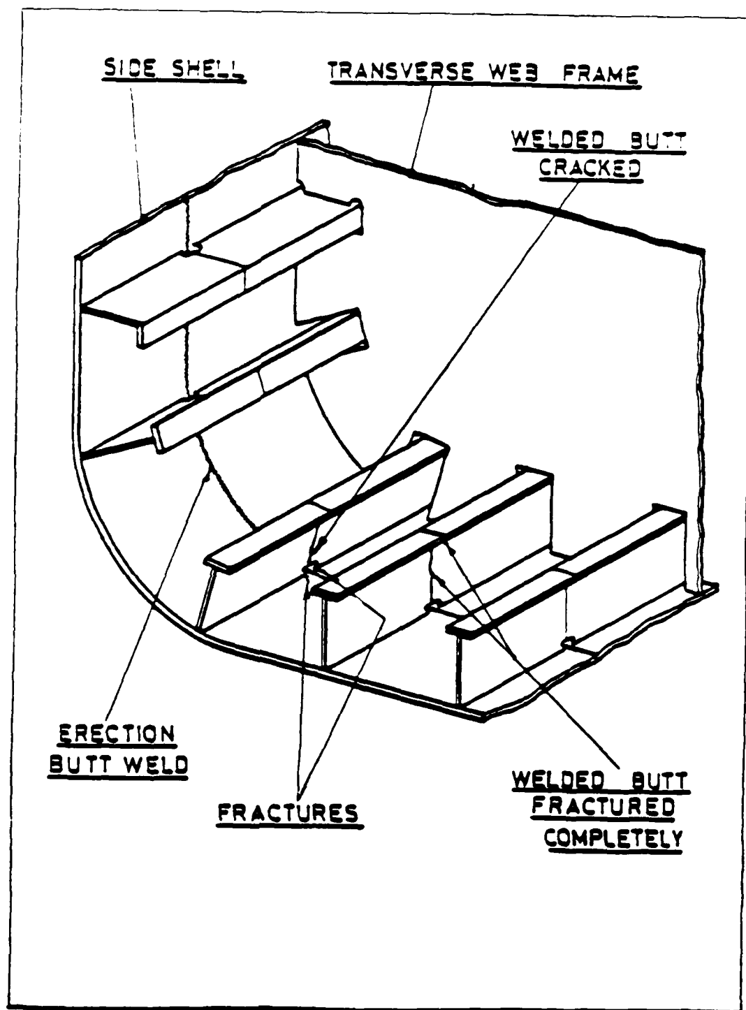
Figure 24: TYPICAL BOTTOM LONGITUDINAL CRACKING
