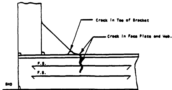
Figure 20: FRACTURE IN LONGITUDINAL INTERCOSTAL GIRDER
