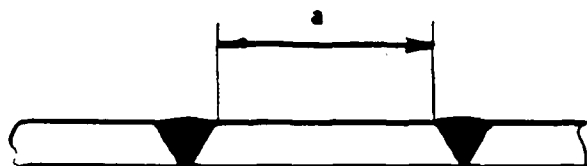
Figure 9: DISTANCE BETWEEN ADJACENT BUTT WELDS
