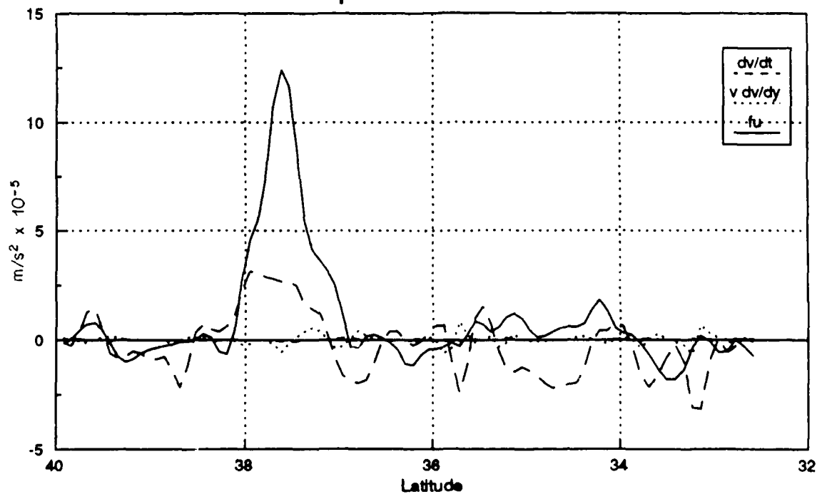
Y momentum equation terms at 200 meters
