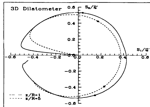
Figure 5.7: Normalized stress paths for DMT.
