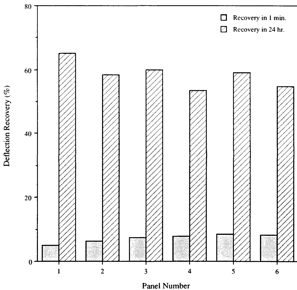
Figure 3-49: Mid-Span Deflection Recovery of Candidate Panels Following Static Pressure Testing
