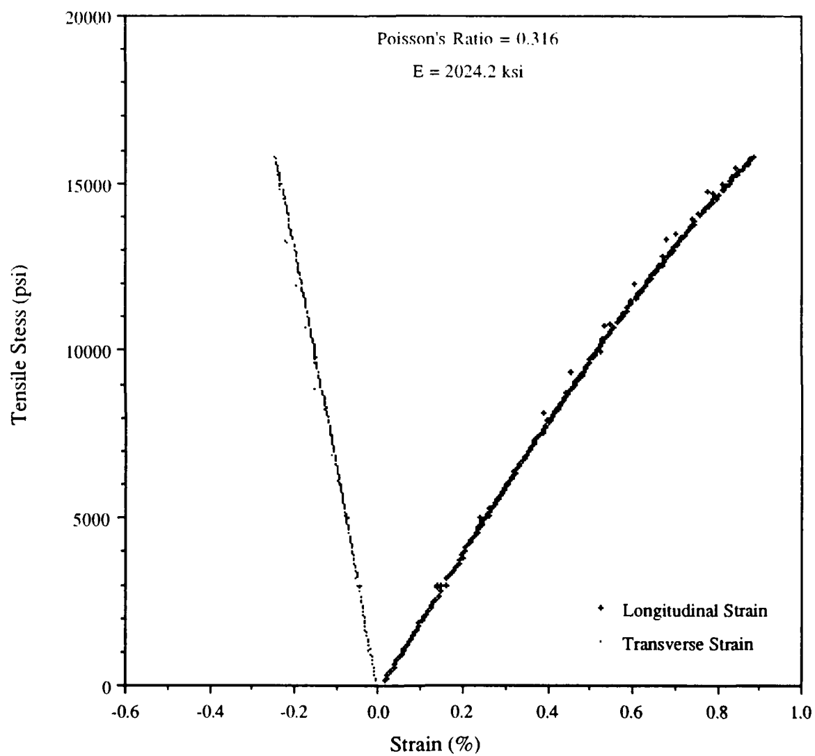
Figure A-2: Tensile Stress vs. Strain for Panel Specimen 1-4 Based on Bi-axial Strain Gage Measurements
