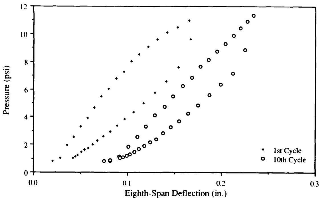
Figure F-10: Eighth-Span Deflection Response of Panel-2 to Cyclic Pressure Loading (Cycles 1 & 10)
