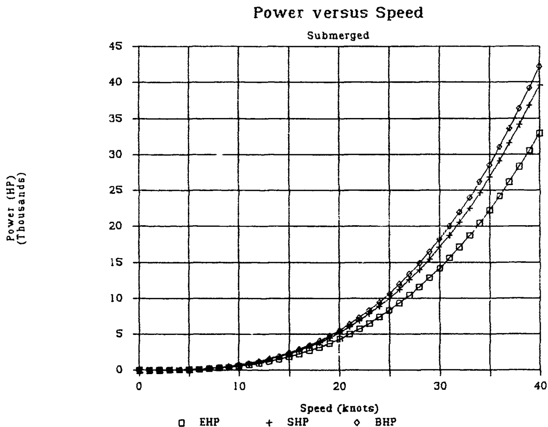
Figure 1 - Power versus Speed Relationship
