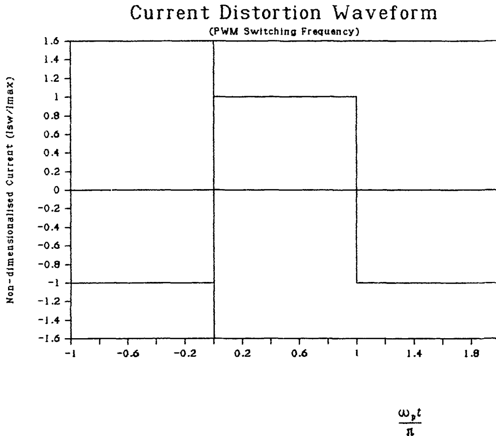
Figure 3 - Current Distortion Waveform
