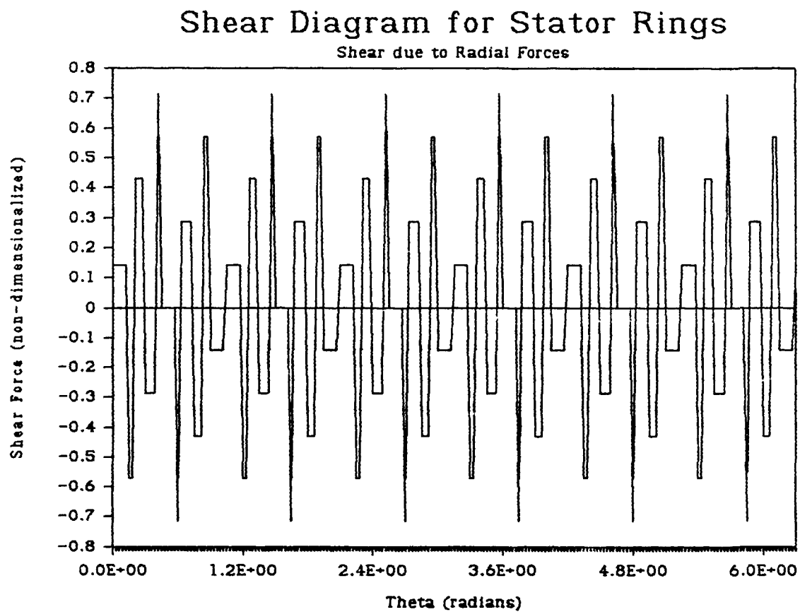
1.16 Figure 2 - Stator Ring Shear Diagram
