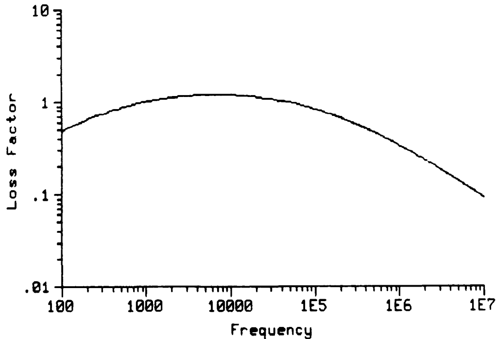
Figure 4. Loss Factor vs Frequency of 4-Parameter Fractional Derivative Model
