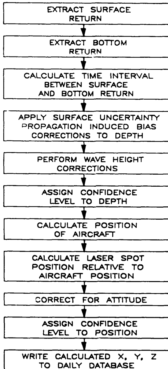
Figure 5-16. Phase I processing summary
