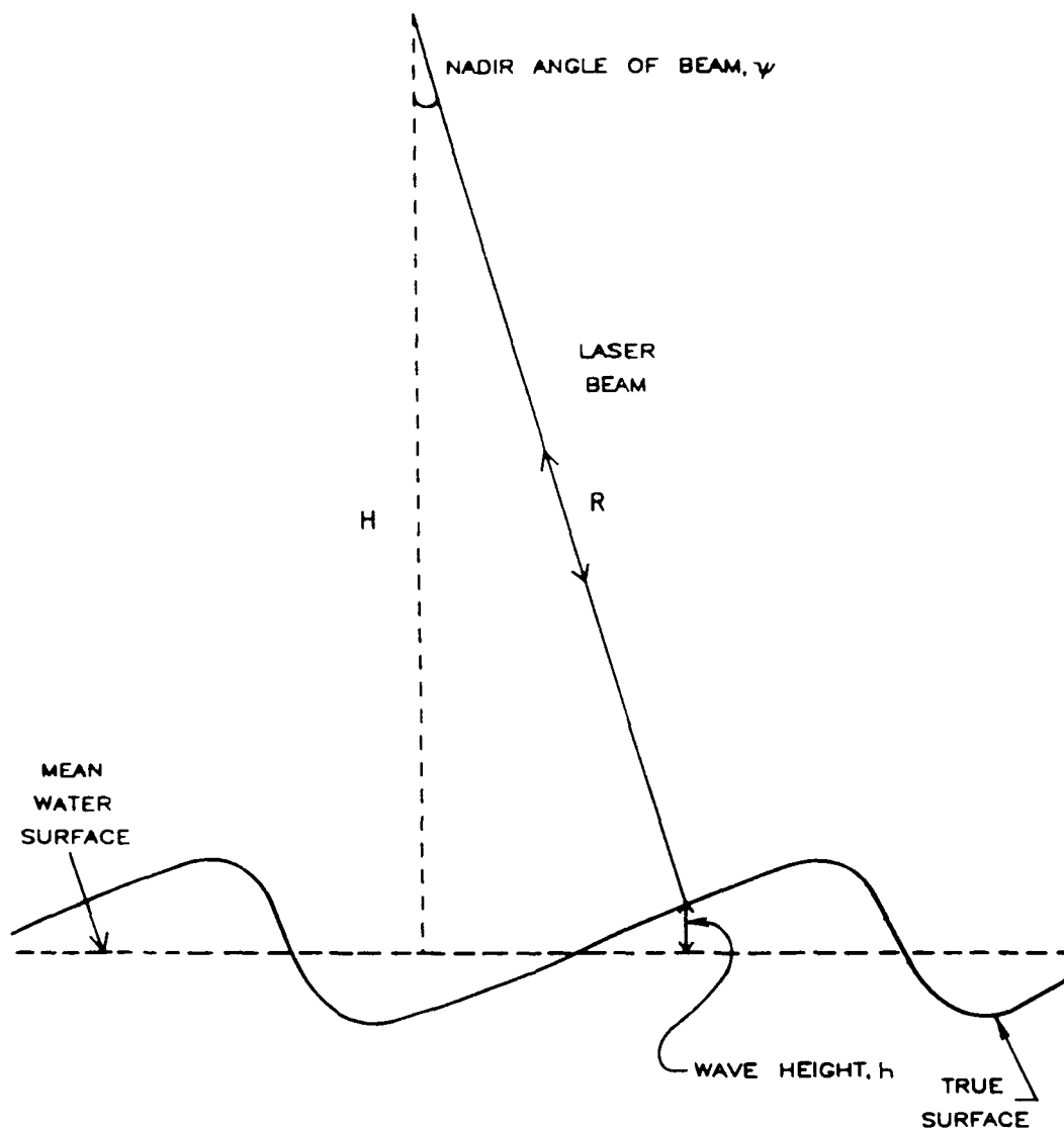
Figure 4-4. Wave correction geometry
