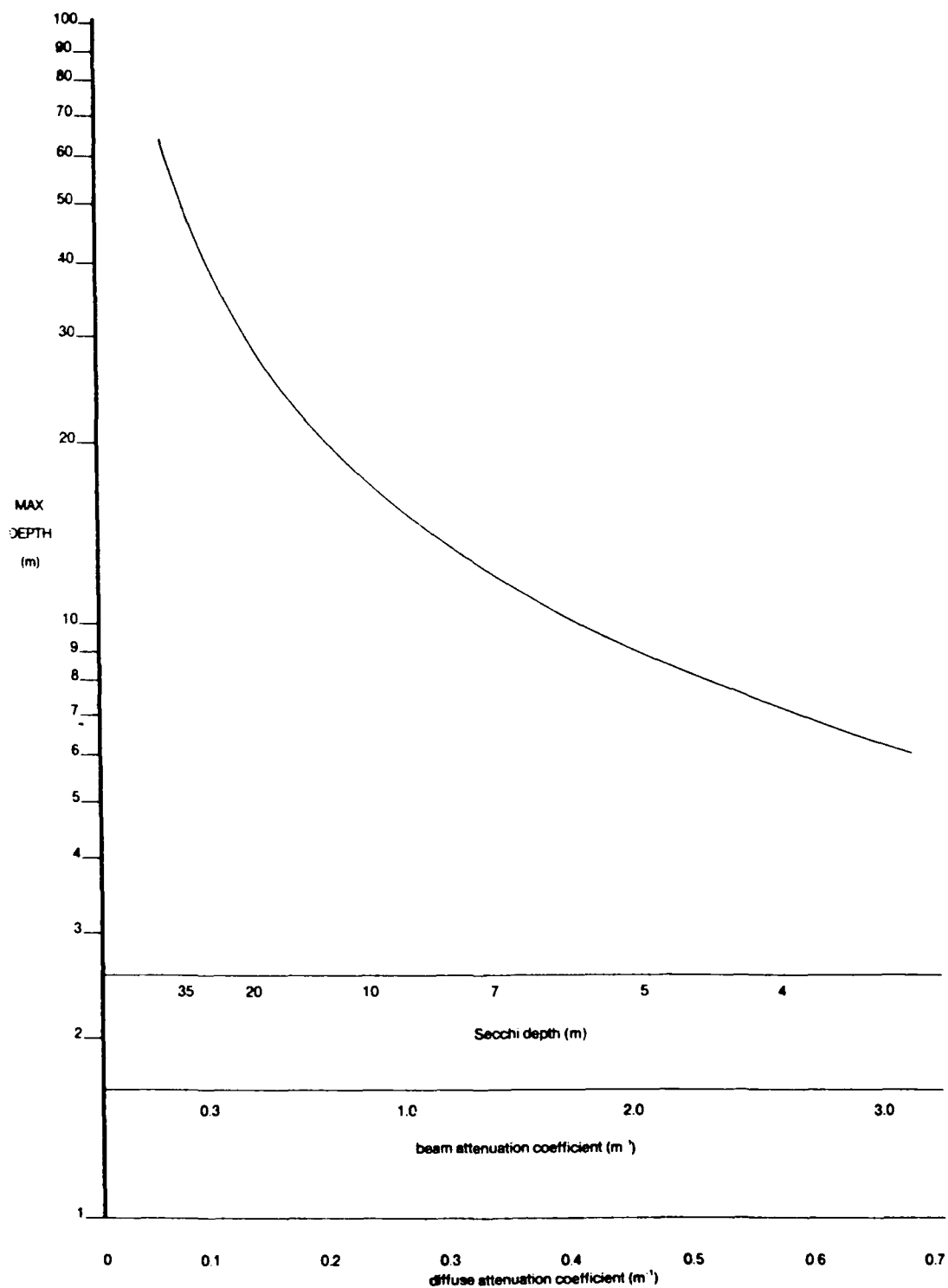
Figure 4-3. Depth penetration versus water clarity
