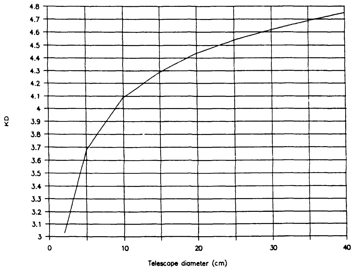
Figure 4-2. Effect of receiver aperture size on depth penetration
