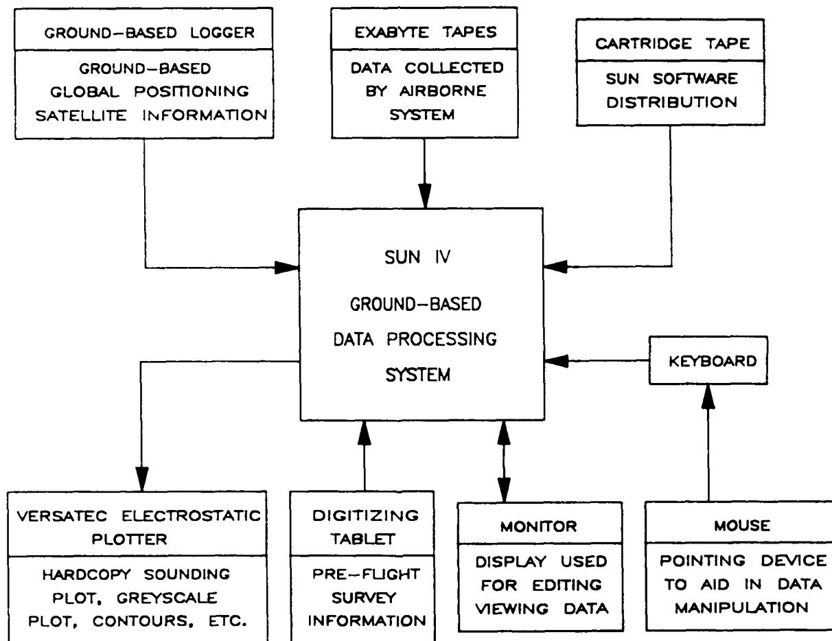
Figure 5-20. System input/output
