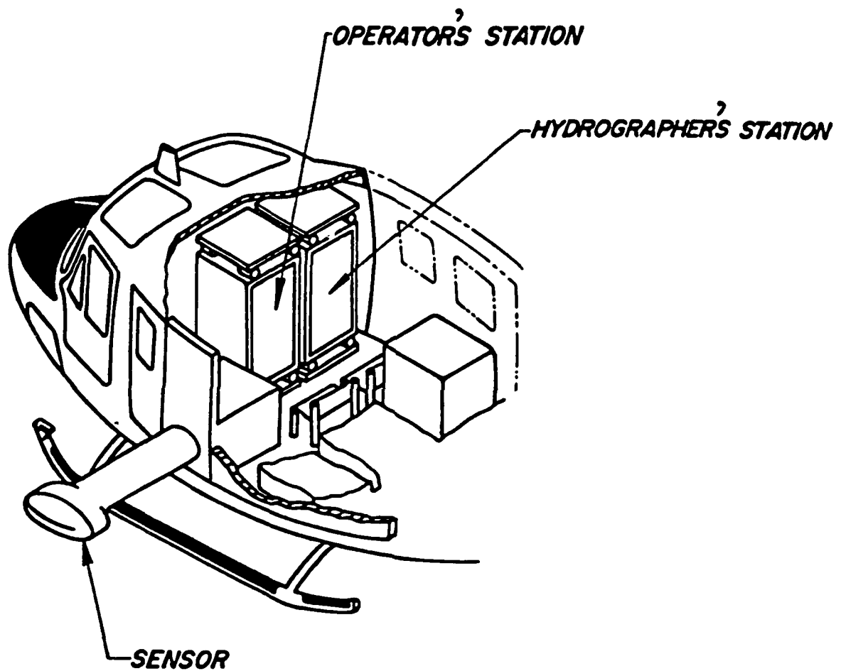
Figure 6-2. Arrangement of equipment
