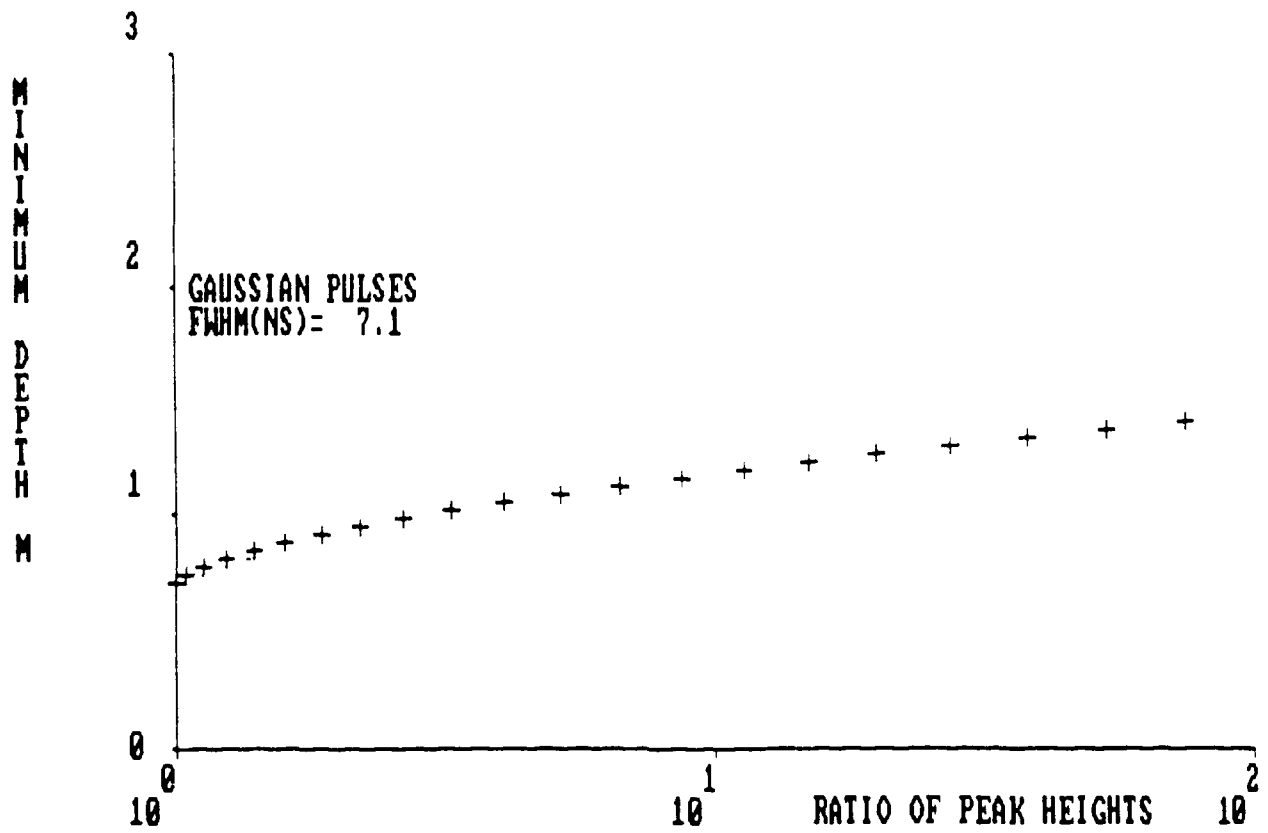
Figure 4-6. Minimum depth versus amplitude ratio for 7.1 ns pulses
