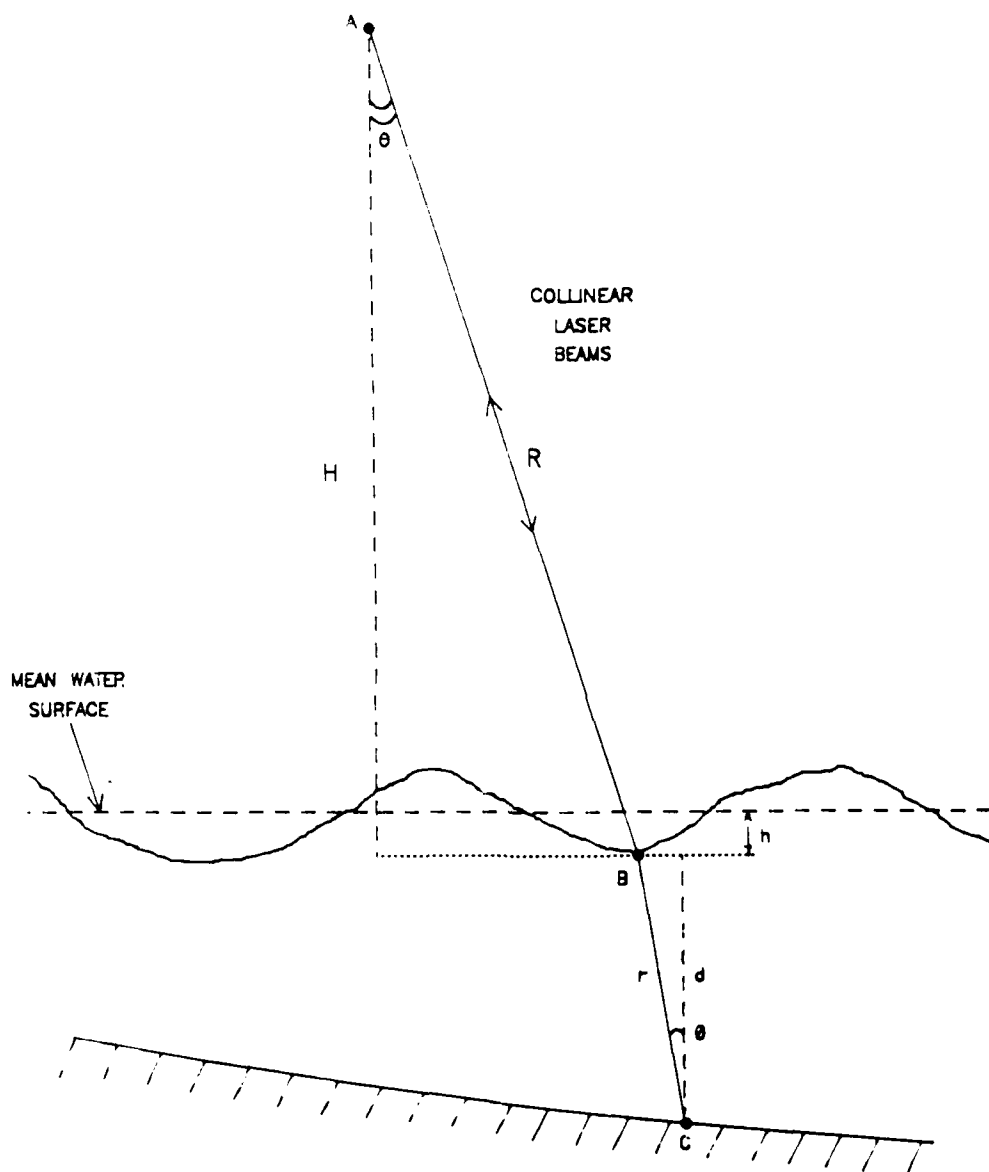
Figure 3-1. Operating principle
