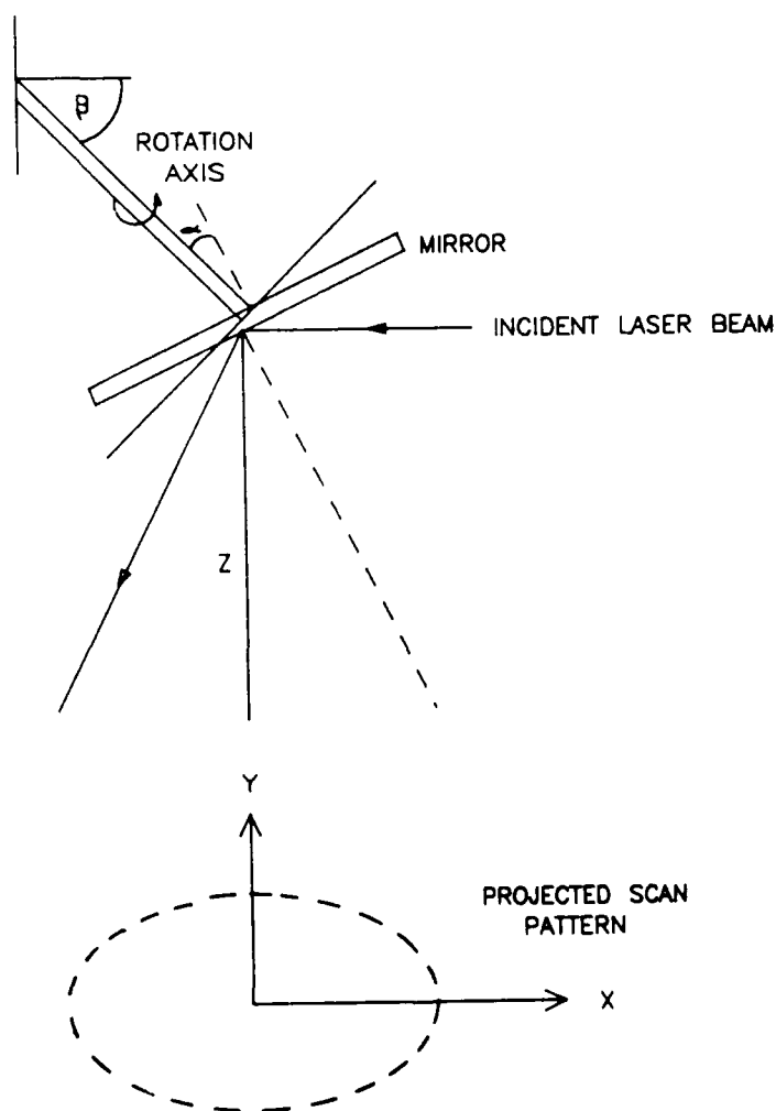
Figure 5-3. Scanner configuration
