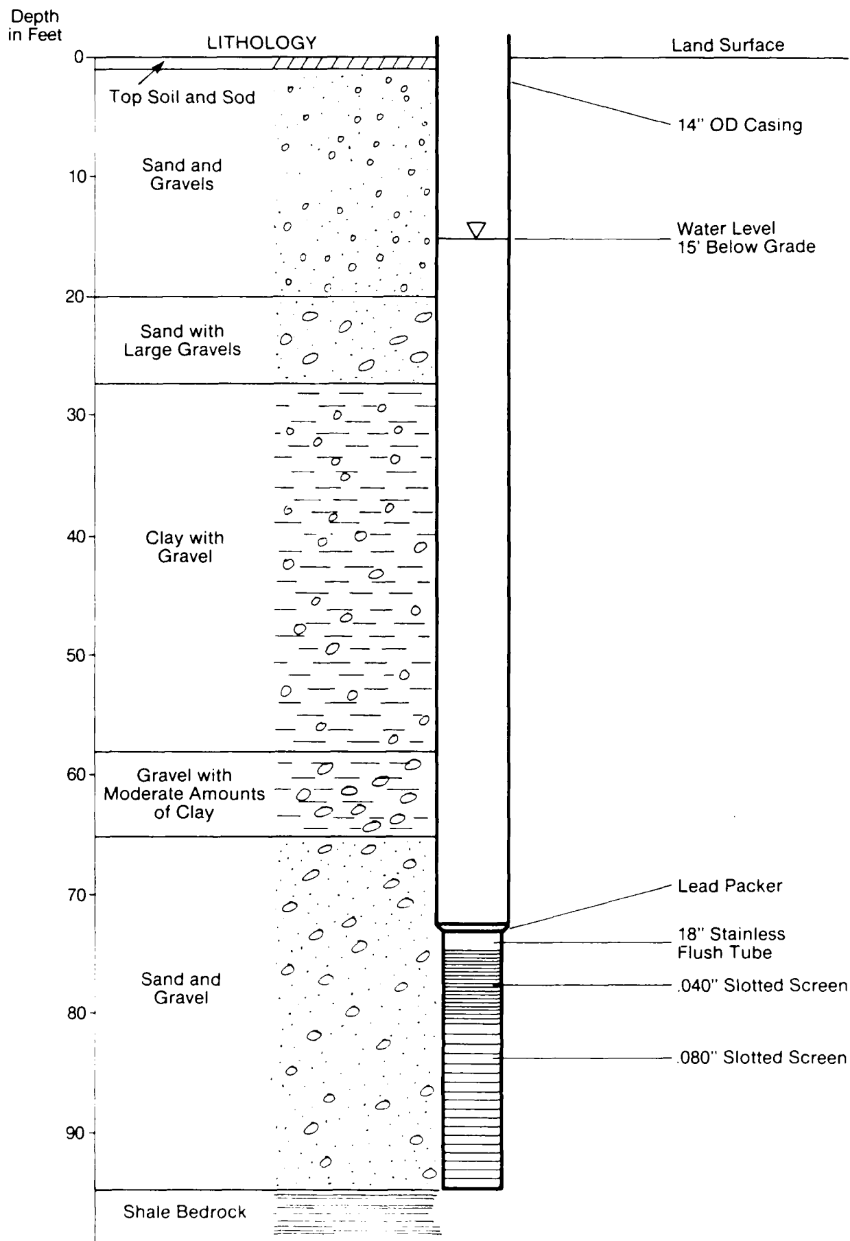
FIGURE 6. Well Construction Detail and Lithologic Log for Well No. 1. AF Plant 59—Drilled May 16, 1974.
