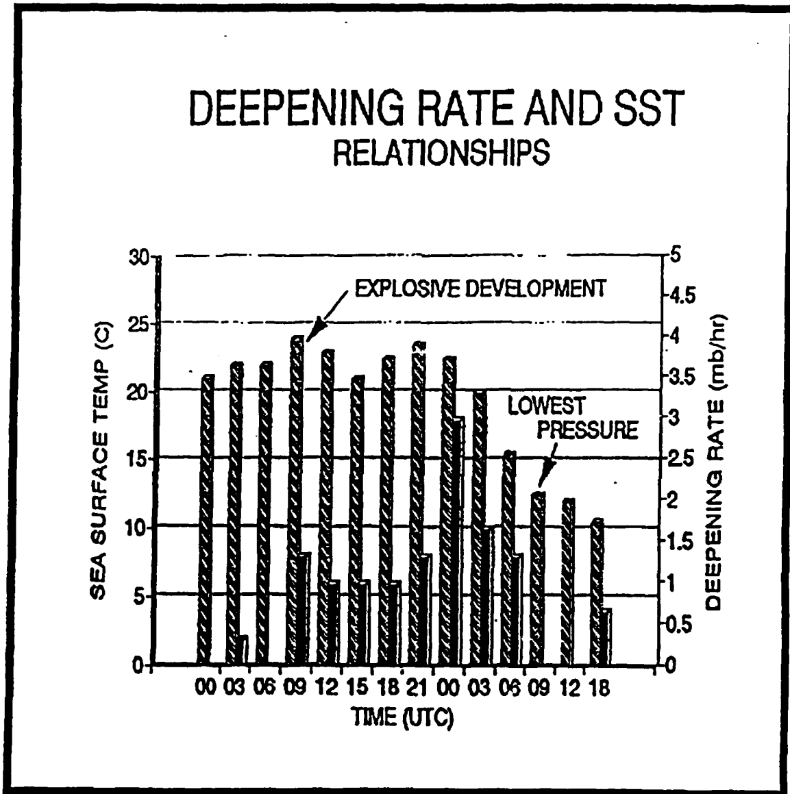
Figure 36. The diagram above suggests the relationship between sea surface temperature (hatched bars) and deepening rate (solid bars) from 0000 UTC on 11 November to 1800 UTC on 12 November.
