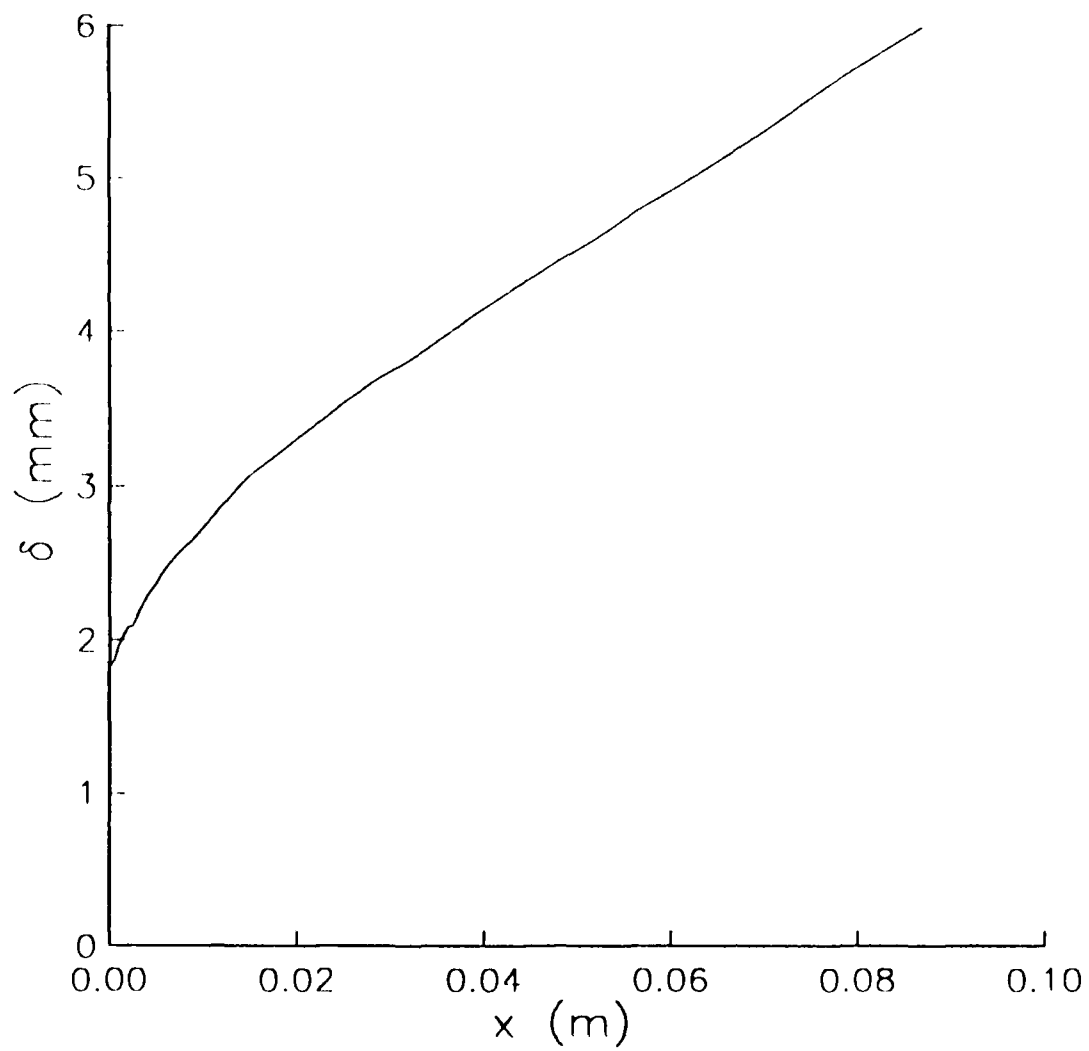
Figure 2. Downstream evolution of the shear layer thickness.
