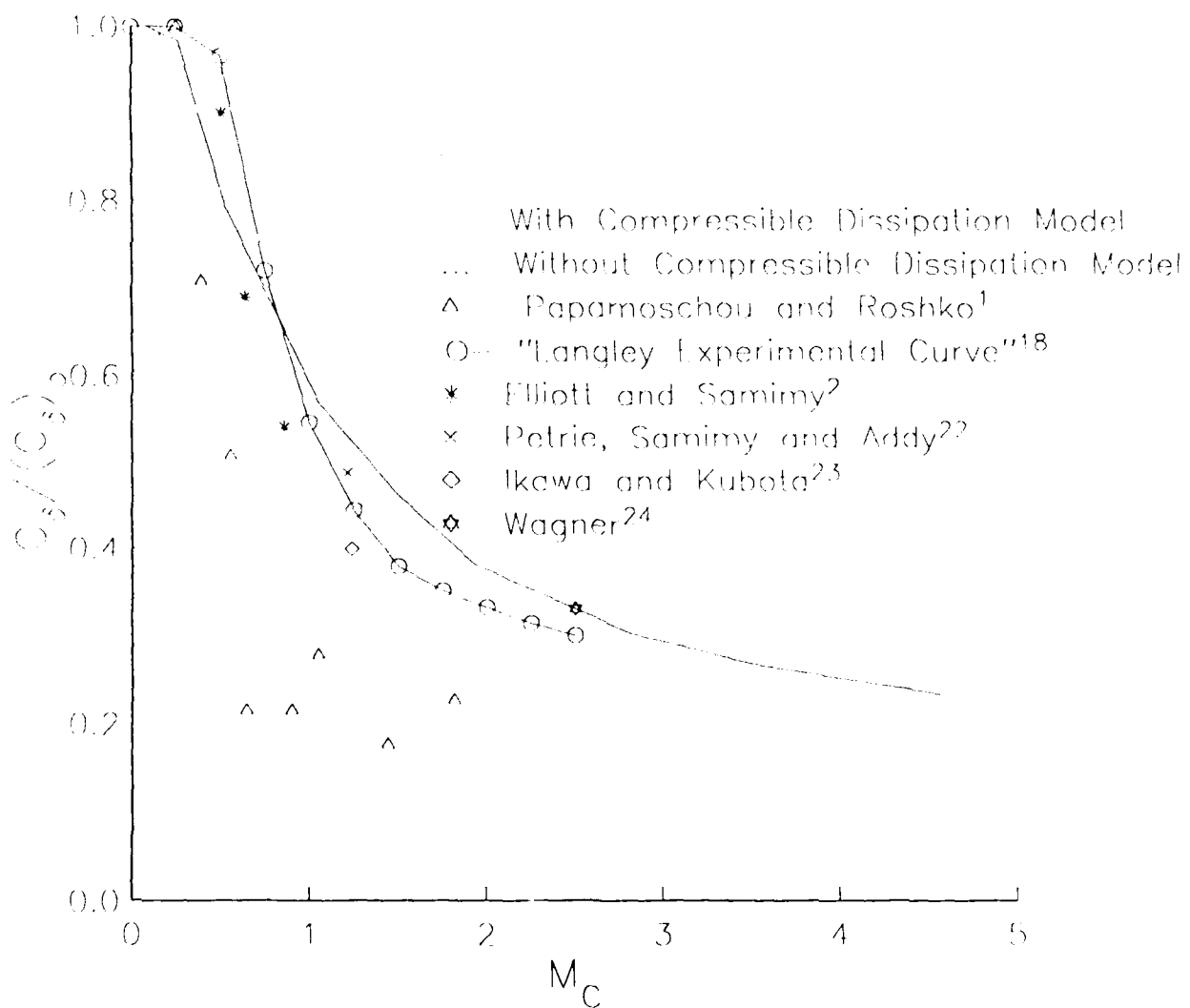
Figure 7. Variation of the growth rate of the compressible shear layer with the convective Mach number.
