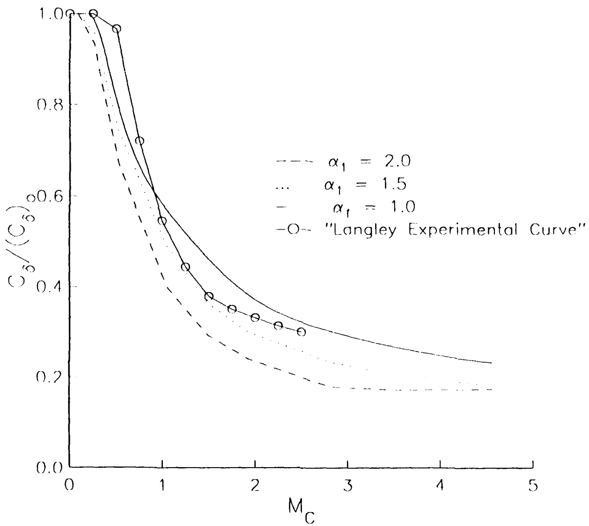
Figure 9. Computed growth rate curves for various values of the parameter \alpha_1 in the model for compressible dissipation.
