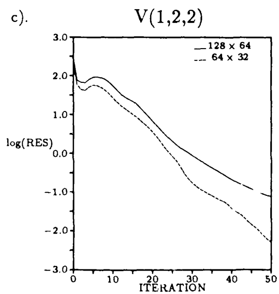
Figure 2: Flow over a bump in a channel, Mach 10
