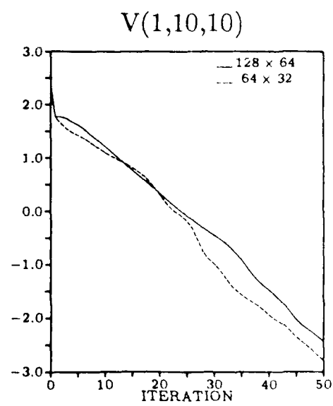
Figure 2: Flow over a bump in a channel, Mach 10
