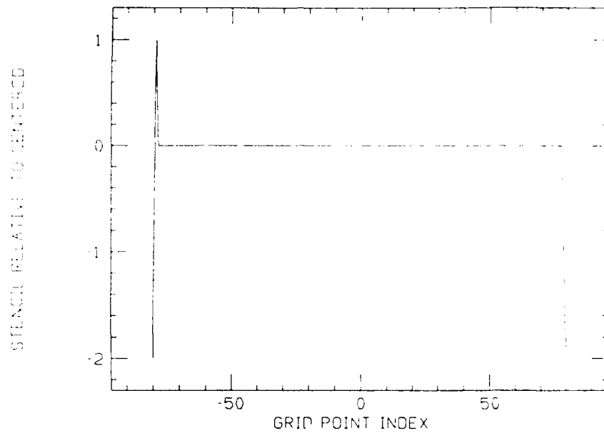
Figure 3h: same as 3b except that a modified ENO is used
