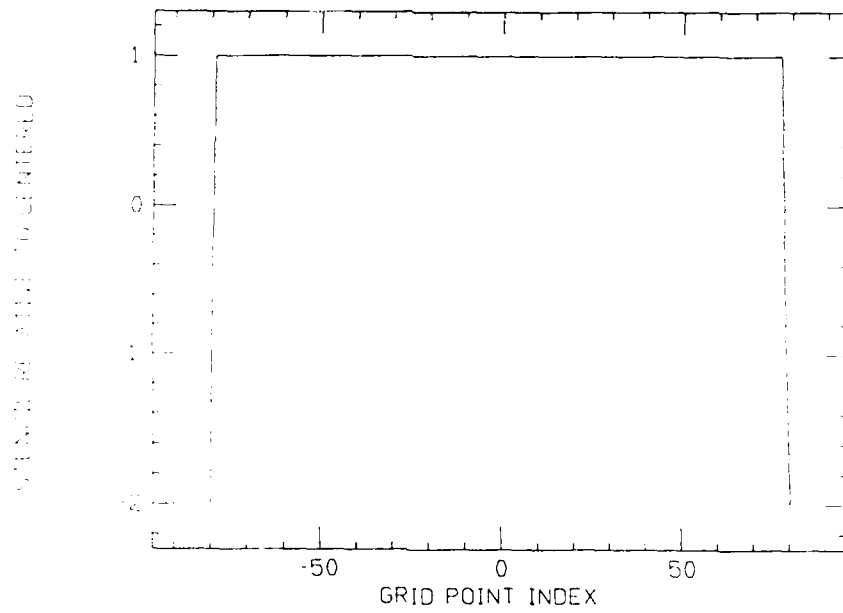
Figure 3b: same as 1b except that u^0(x) = e^{-x}
