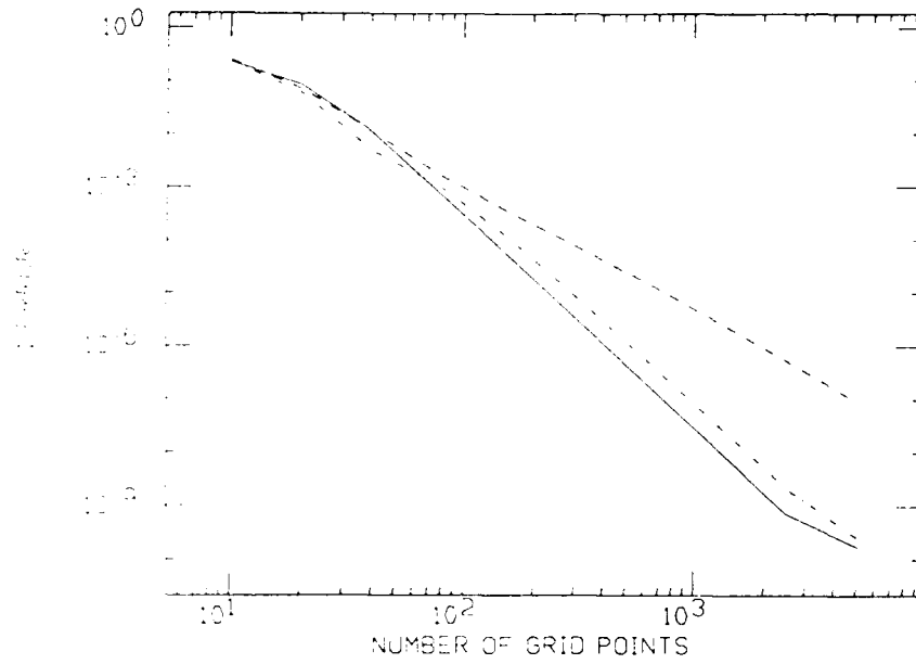
Figure 4a: same as 2a except that the exact time evolution is used
