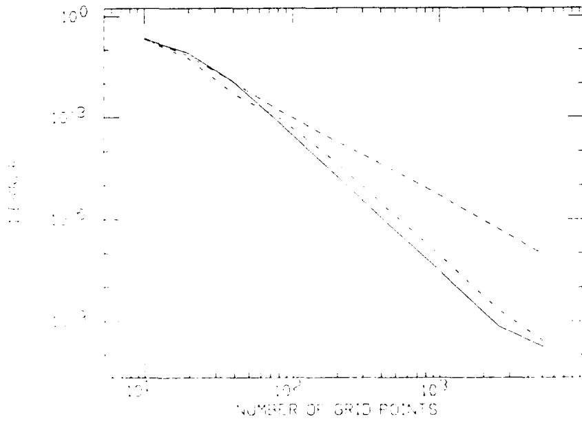
Figure 4b: same as 4a except that the cell-averaged ENO is used
