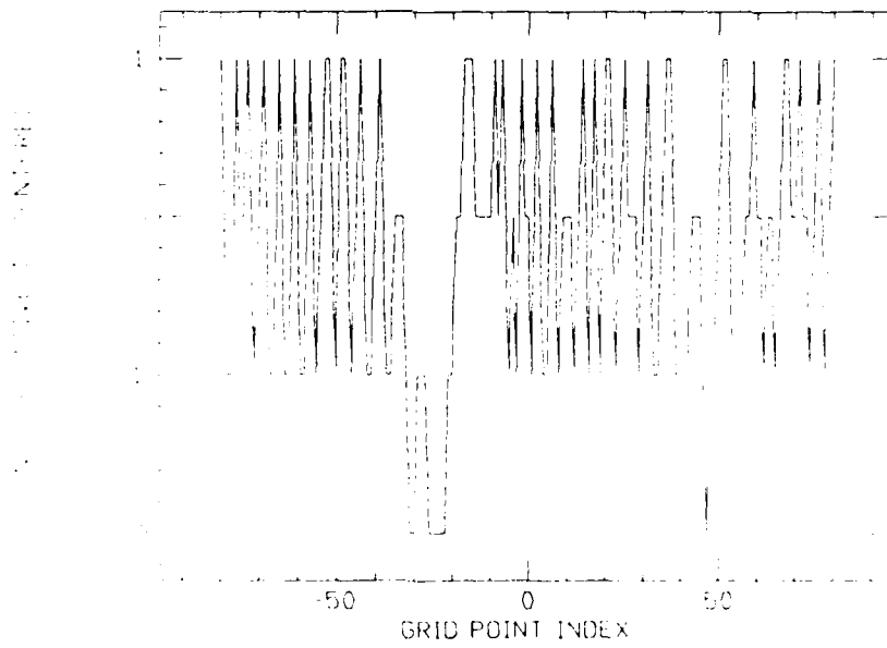
Figure 3c: same as 3b except that t = 100\Delta t
