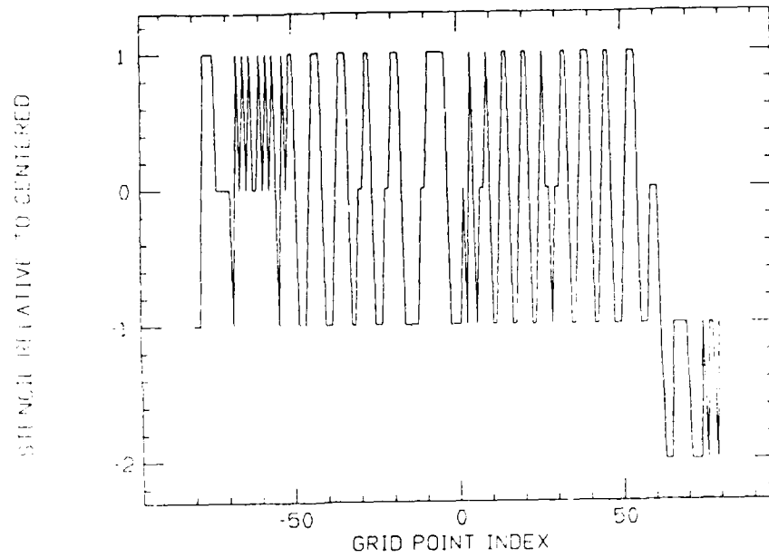
Figure 3d: same as 3b except that t = 4
