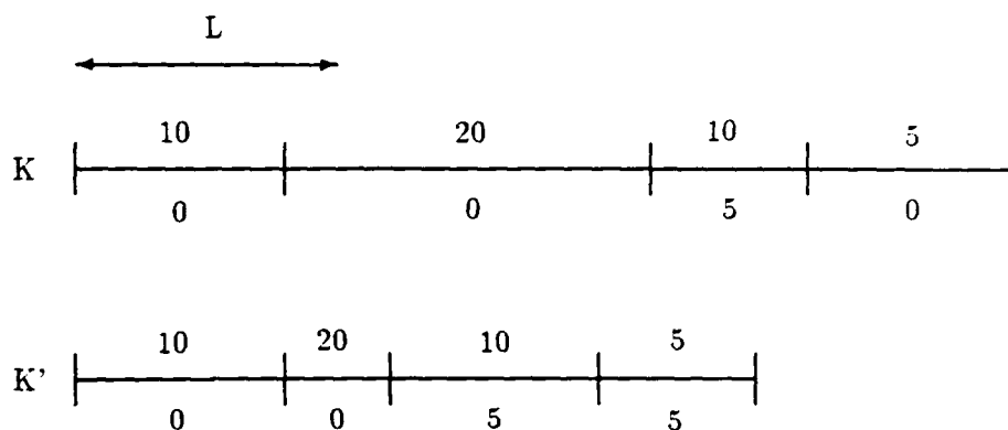
Figure 11: Configuration Space
