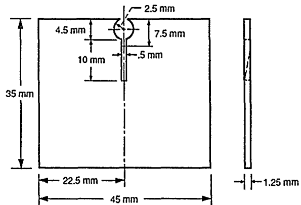
Figure 2. - Specimen geometry.
