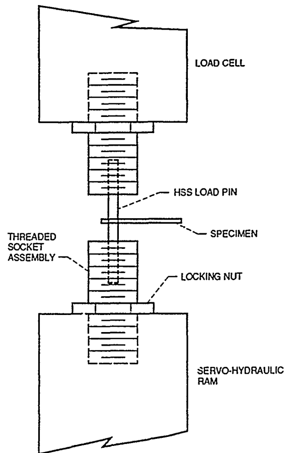
Figure 3. - Socket assembly.
