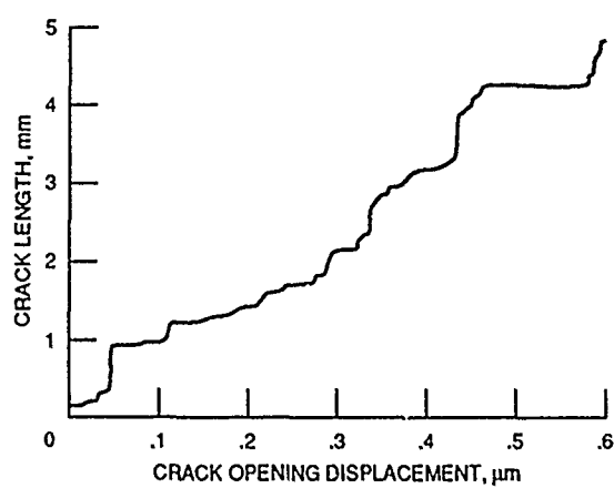
Figure 5. - Typical experimental results for monolithic \text{Al}_2\text{O}_3 ceramic specimen.
