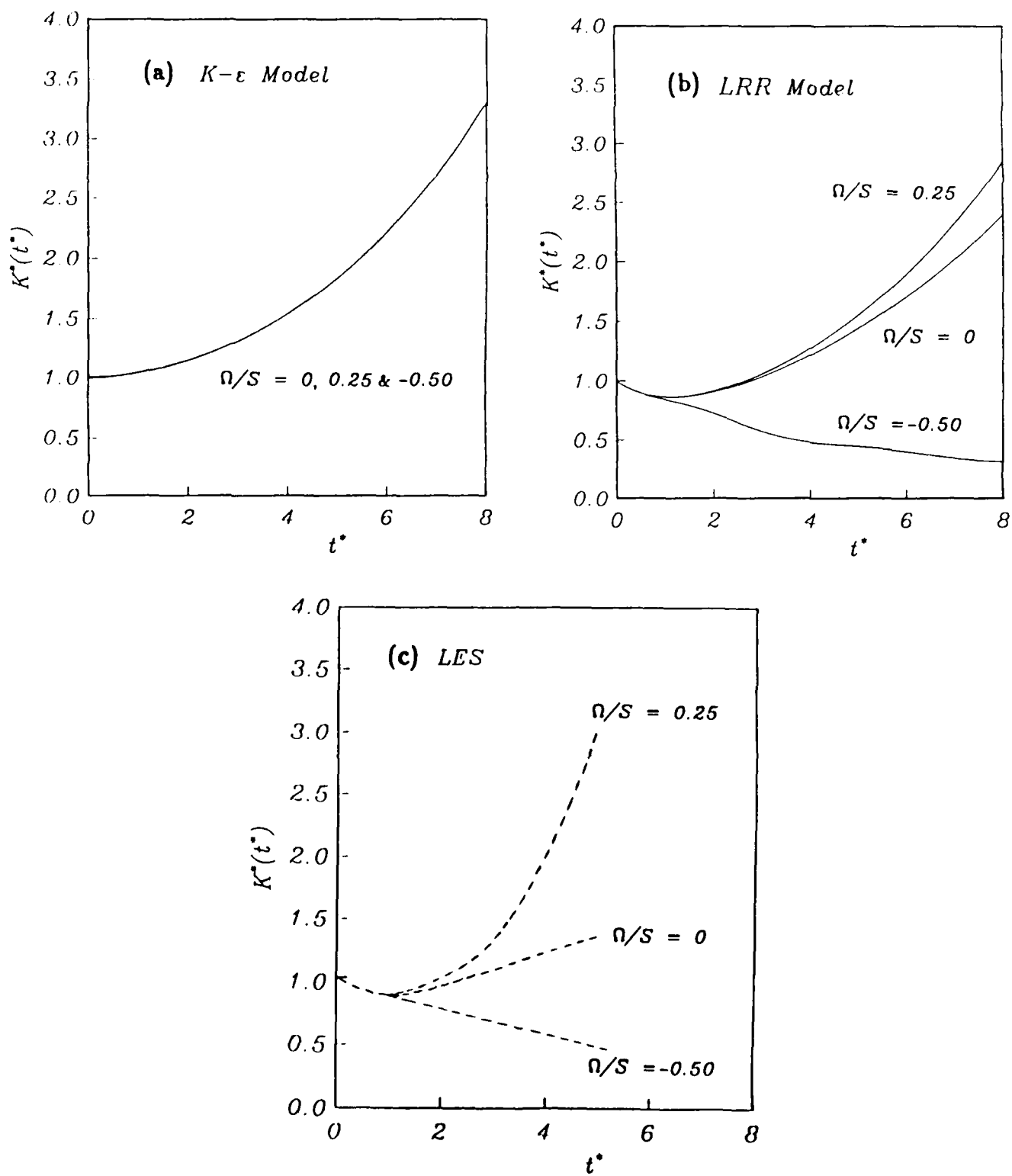
Figure 9. Time evolution of the turbulent kinetic energy in rotating shear flow for \epsilon_0/SK_0 = 0.296 : (a) standard K - \epsilon model, (b) Launder, Reece, and Rodi model, and (c) large-eddy simulations of Bardina, Ferziger, and Reynolds (1983).
