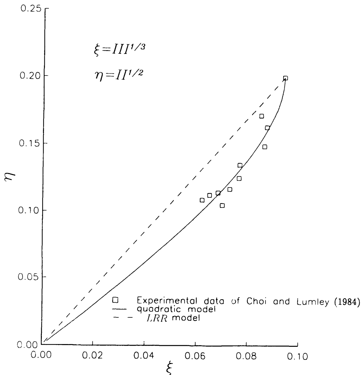
Figure 6. Phase space portrait of the return to isotropy problem: Comparison of the predictions of the Launder, Reece, and Rodi model and the quadratic model of Sarkar and Speziale (1990) with the experimental data of Choi and Lumley (1984) for the relaxation from plane strain.
