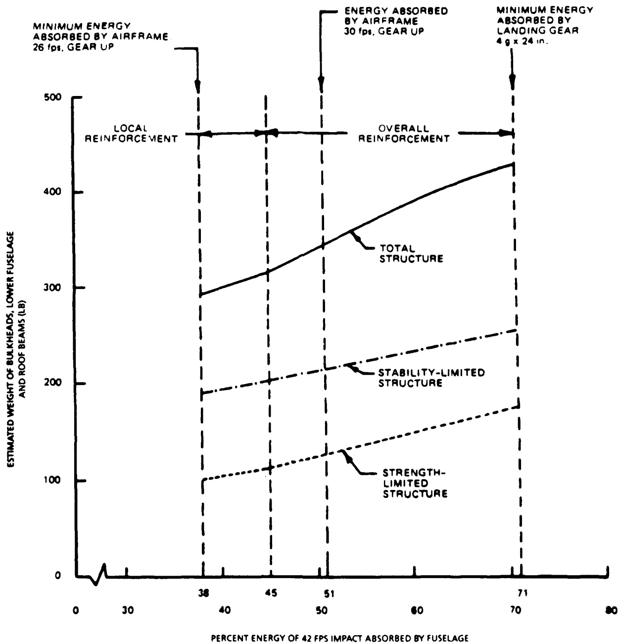
Figure 19. Typical variation of required fuselage weight versus energy absorbed for a utility helicopter.
