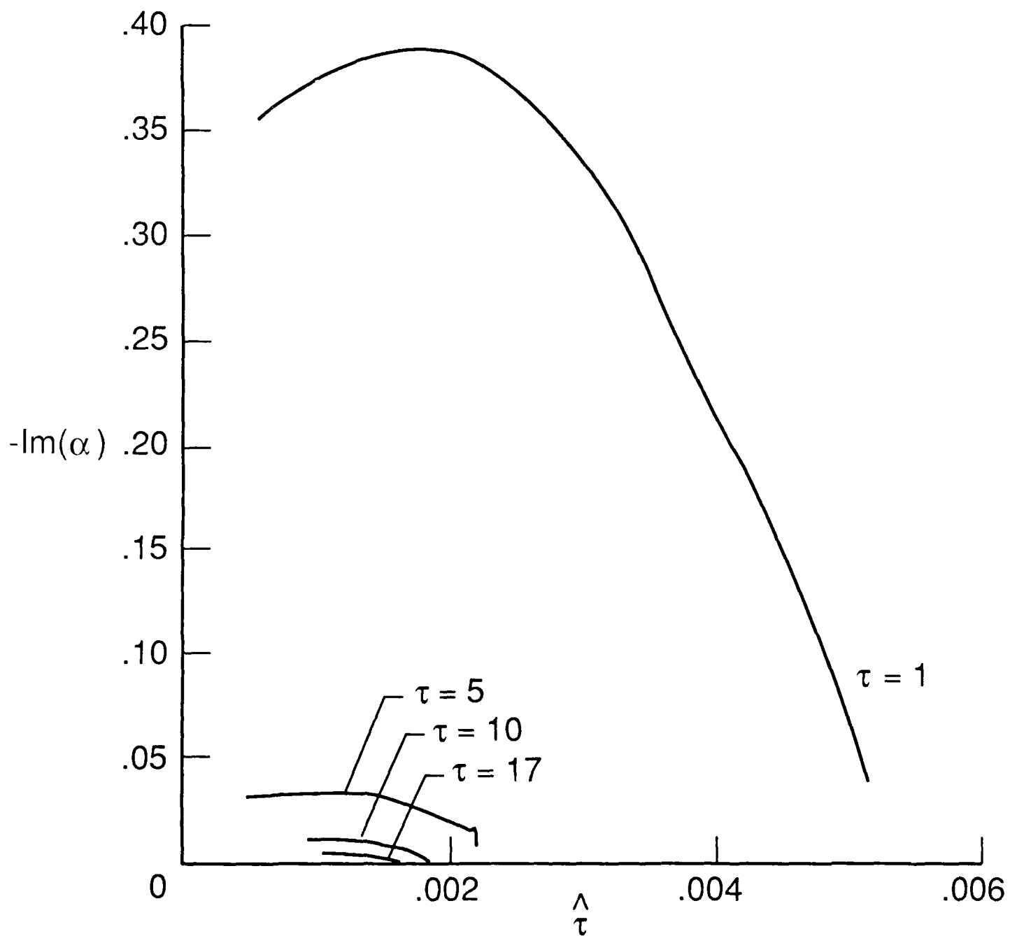
Figure 4(d). -\text{Im}(\alpha) as a function of \hat{\lambda} for M_\infty = 2 , \beta = 0 and \tau = 1, 5, 10, 17 .
