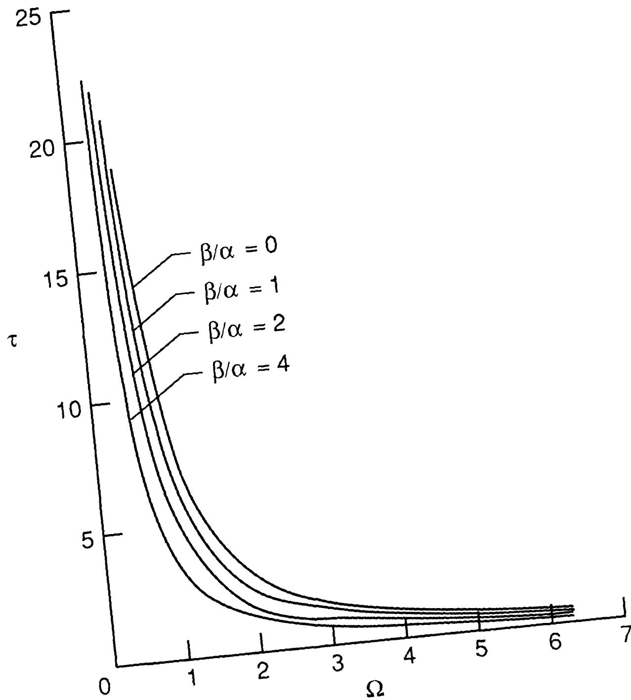
Figure 2(a). Neutral value of \tau versus frequency \Omega for M_\infty = 0.5 and \beta/\alpha = 0, 1, 2, 4 .
