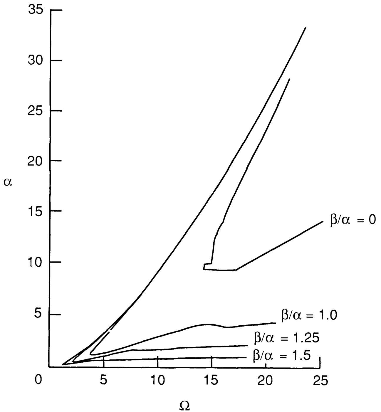
Figure 2(c). Neutral value of \alpha versus frequency \Omega for M_\infty = 2 and \beta/\alpha = 0, 1, 1.25, 1.5 .
