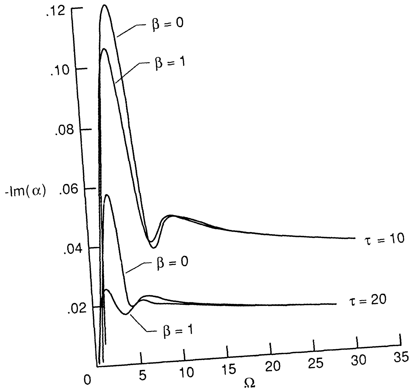
Figure 2(g). Growth rate versus frequency \Omega for M_\infty = 0.5 , \beta = 0, 1 and \tau = 10, 20 .
