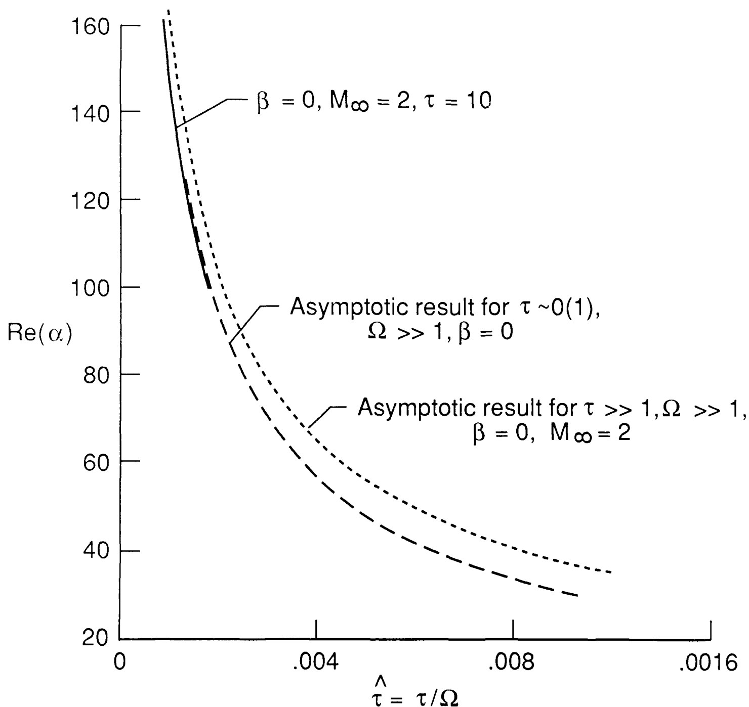
Figure 4(a). Asymptotic solution for \text{Re}(\alpha) as a function of \hat{\tau} = \tau/\Omega , for \tau \gg 1 and \Omega \gg 1 for \beta = 0 and M_{\infty} = 2 , for \tau \sim O(1), \Omega \gg 1 and \beta = 0 from (3.12), along with the full computational solution for M_{\infty} = 2, \beta = 0 and \tau = 10 .
