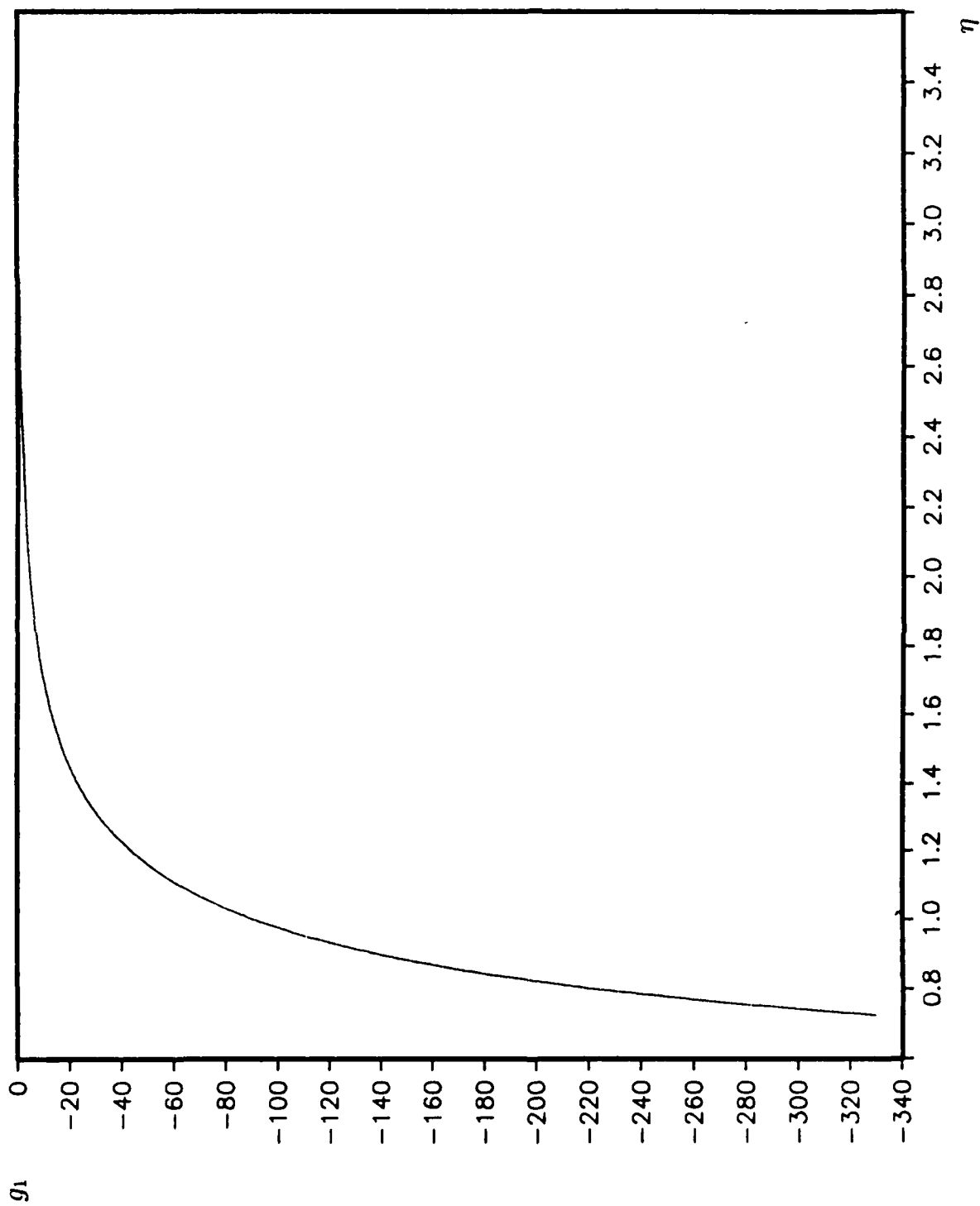
Figure (2.1b) The solution of the transition layer equation (2.10a) for the adiabatic case T_i = 1 with \gamma = 1.4 .
