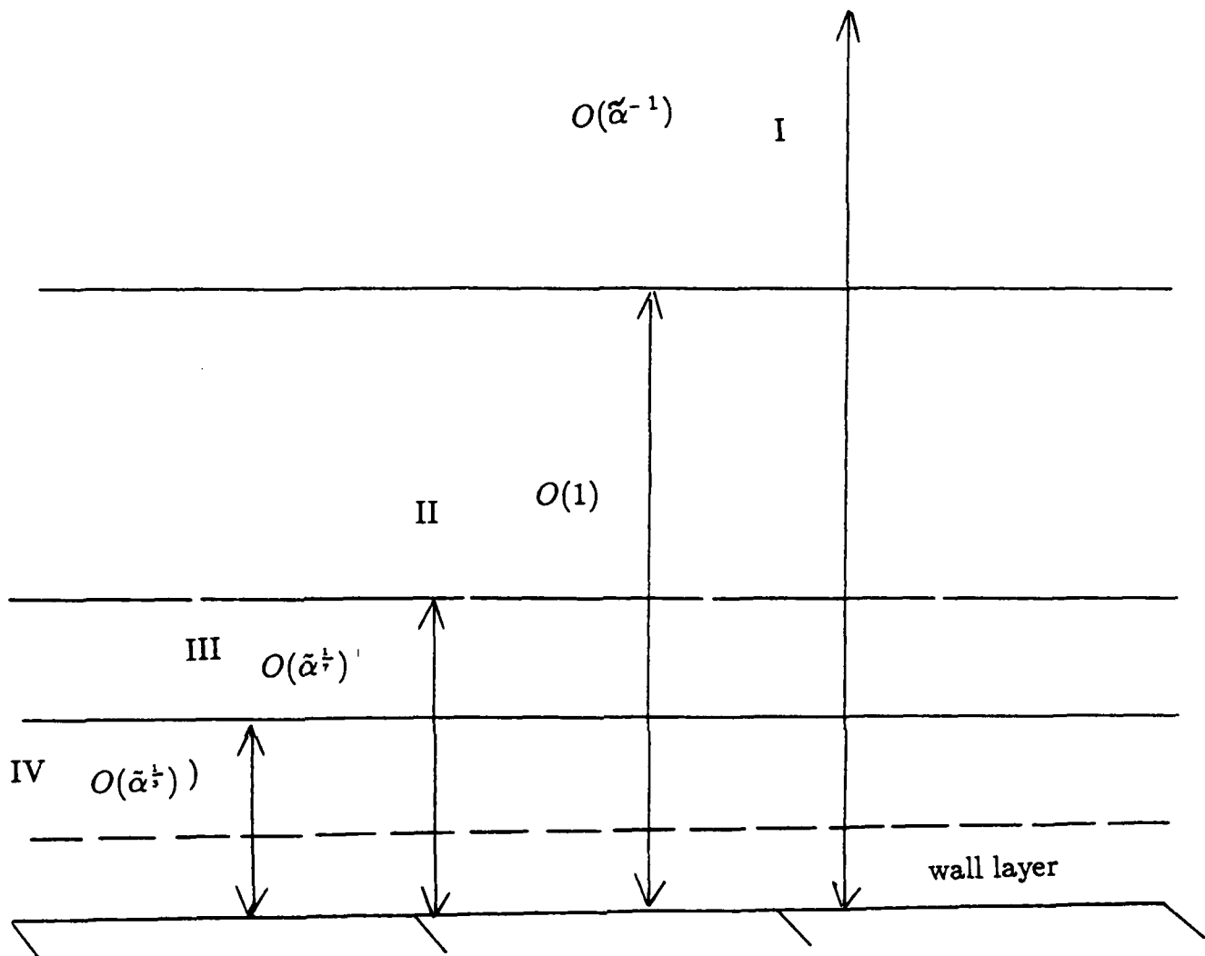
Figure (3.3) The different regions which emerge in the small \tilde{\alpha} limit.
