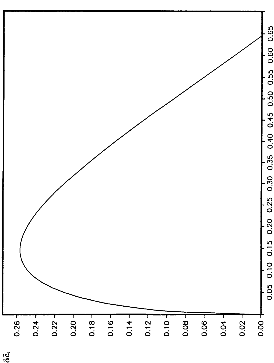
Figure (3.1) The dependence of the vorticity mode growth rate \tilde{\alpha} \tilde{c}_i on the wavenumber \tilde{\alpha} .
