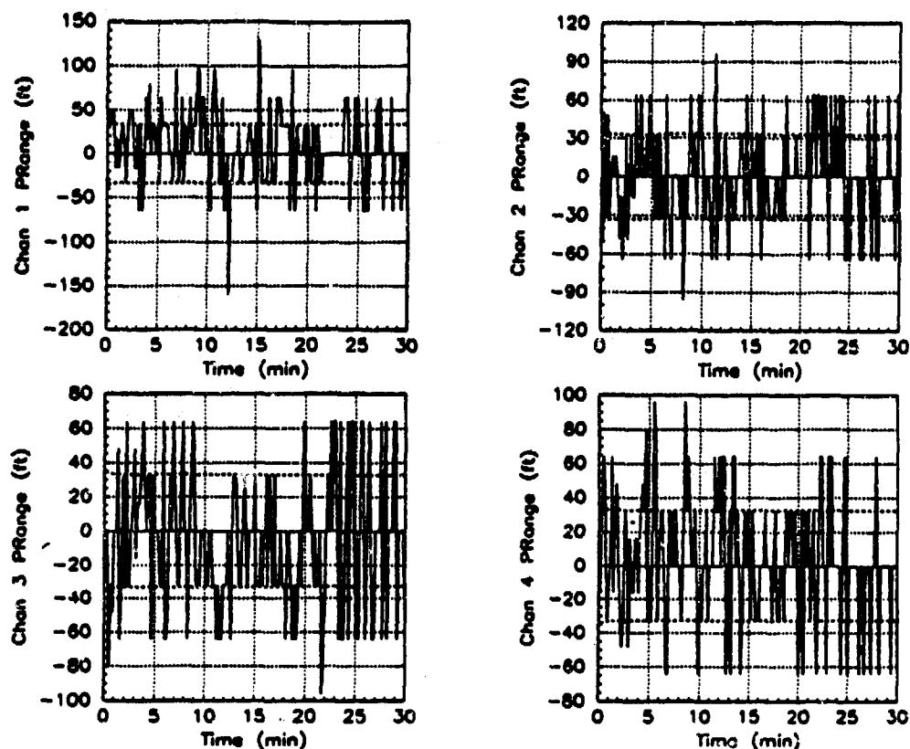
Figure 4.2. Pseudorange Residuals
