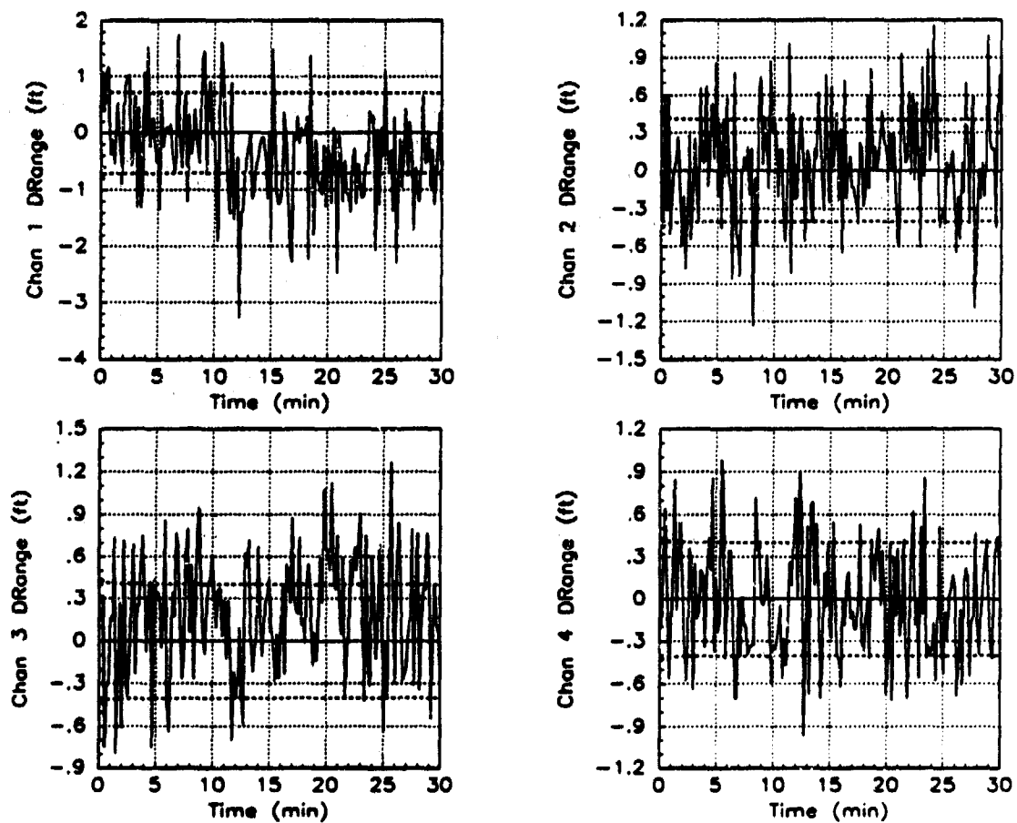
Figure 4.3. Delta-Range Residuals
