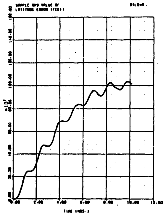
Figure G.1. Litton Static Navigation Errors
