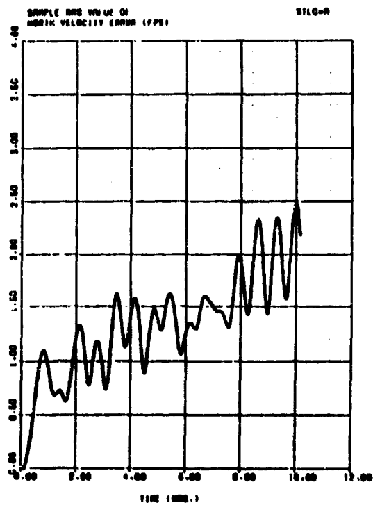
Figure G.2. Static Navigation Errors
