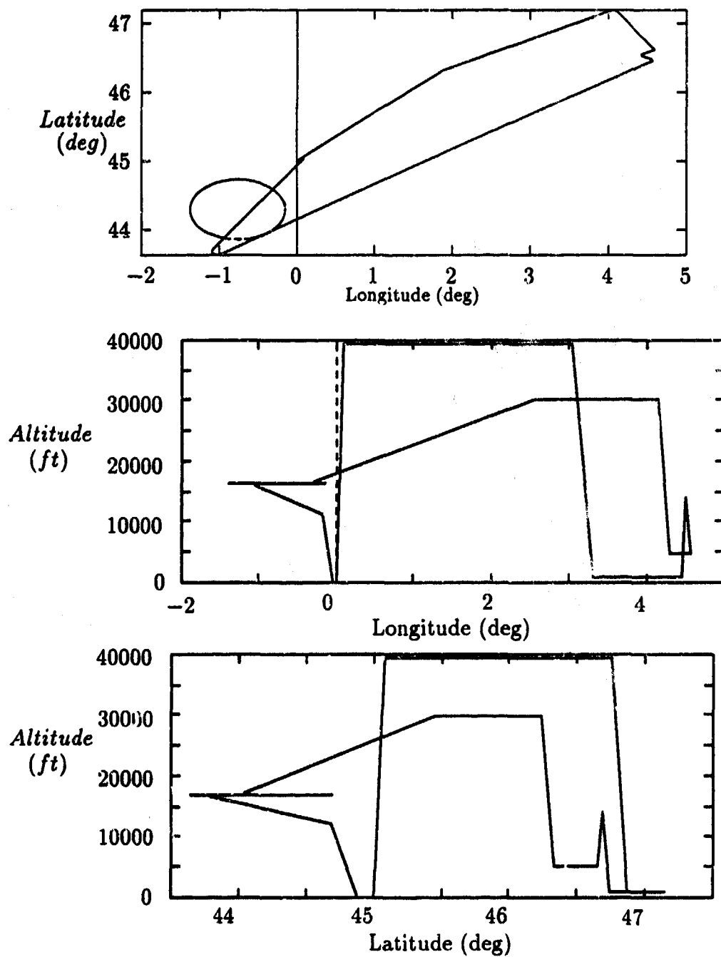
Figure 3.3. Fighter Flight Profile
