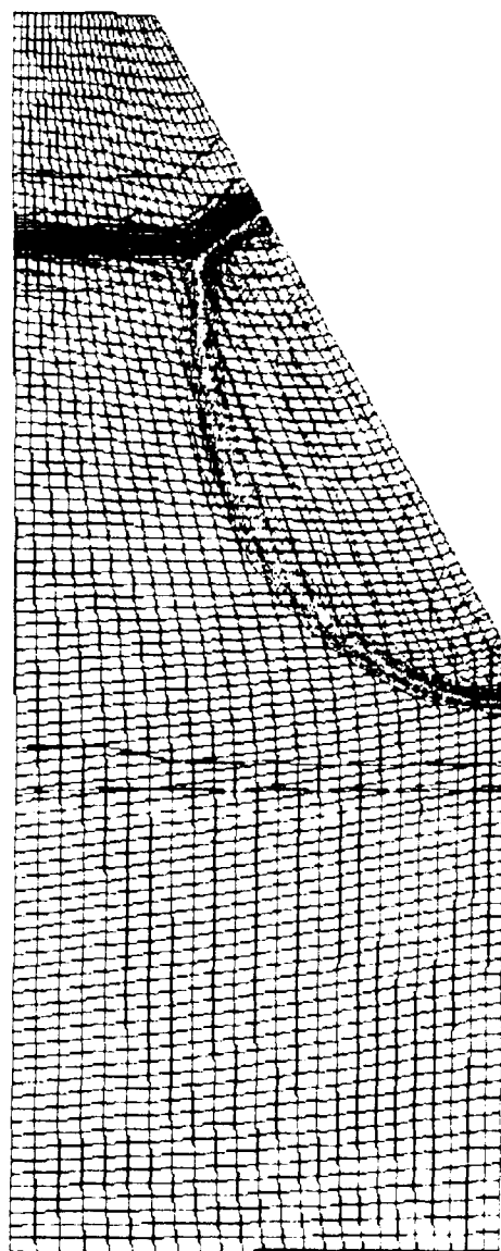
Figure 4. Density and Pressure Contours Superimposed on 98x25 Grid. M_I = 2.12 , 30 Degree Wedge
