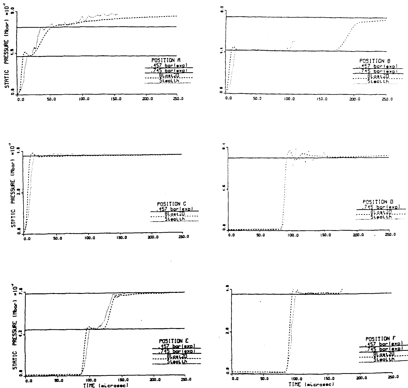
Figure 12. Pressure versus Time Histories, Positions A-F, BLAST2D 98x25 Grid, STEALTH 99x26 Grid
