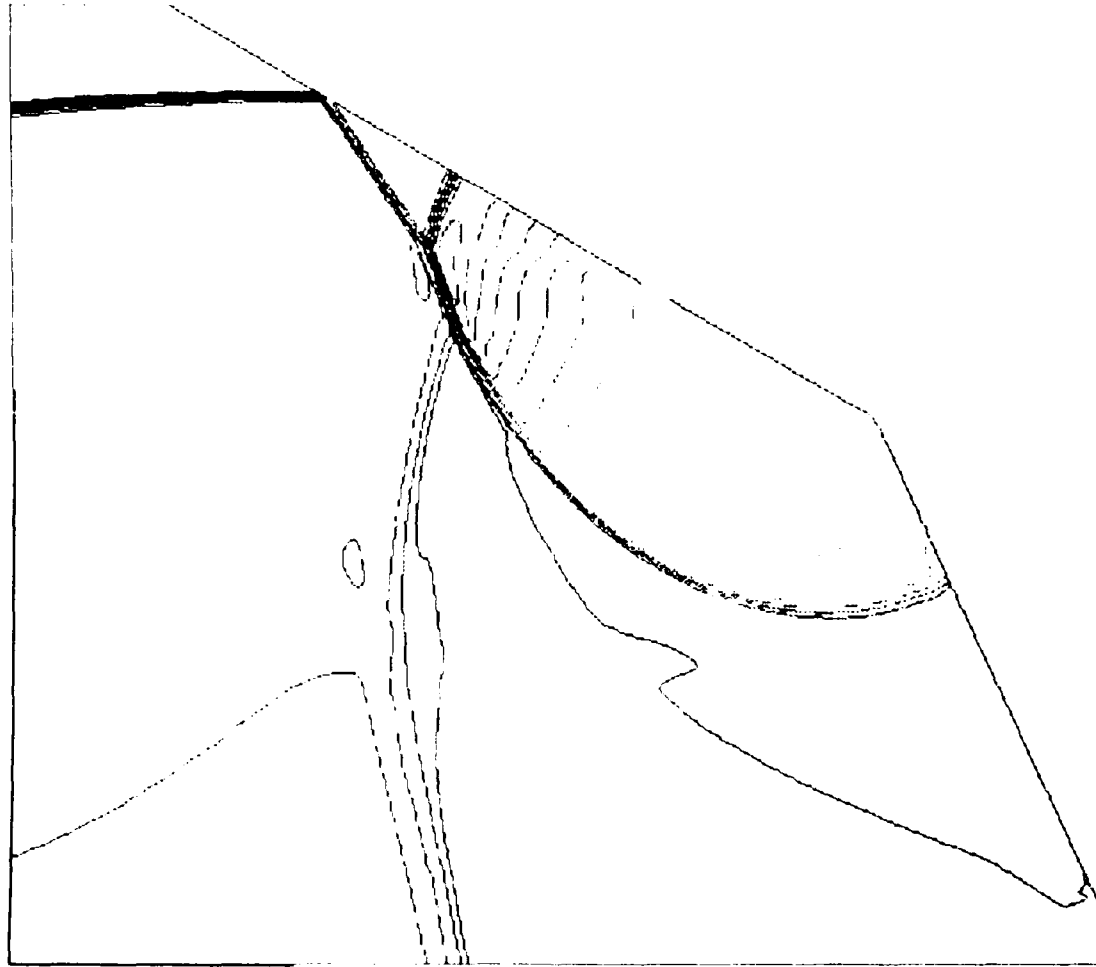
Figure 22. Density Contour Plot, 25 and 60 Degree Double Wedge
