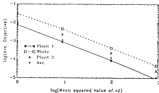
Figure 5: Simulation results obtained when true plant is P_1 and loop is driven by spectra shown in Figure 4.
