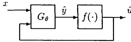
Figure 8: Feedback nonlinearity.
