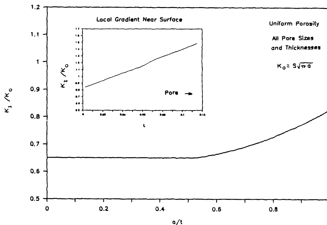
FIGURE 22. STRESS INTENSITY SOLUTION FOR UNIFORM POROSITY. INSET SHOWS THE DECAY OF THE STRESS INTENSITY AS THE CRACK GROWS AWAY FROM THE PORE STRESS GRADIENT TOWARD THE SURFACE
