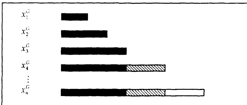
Figure 2.2b. Discounted Linear Objective Function
