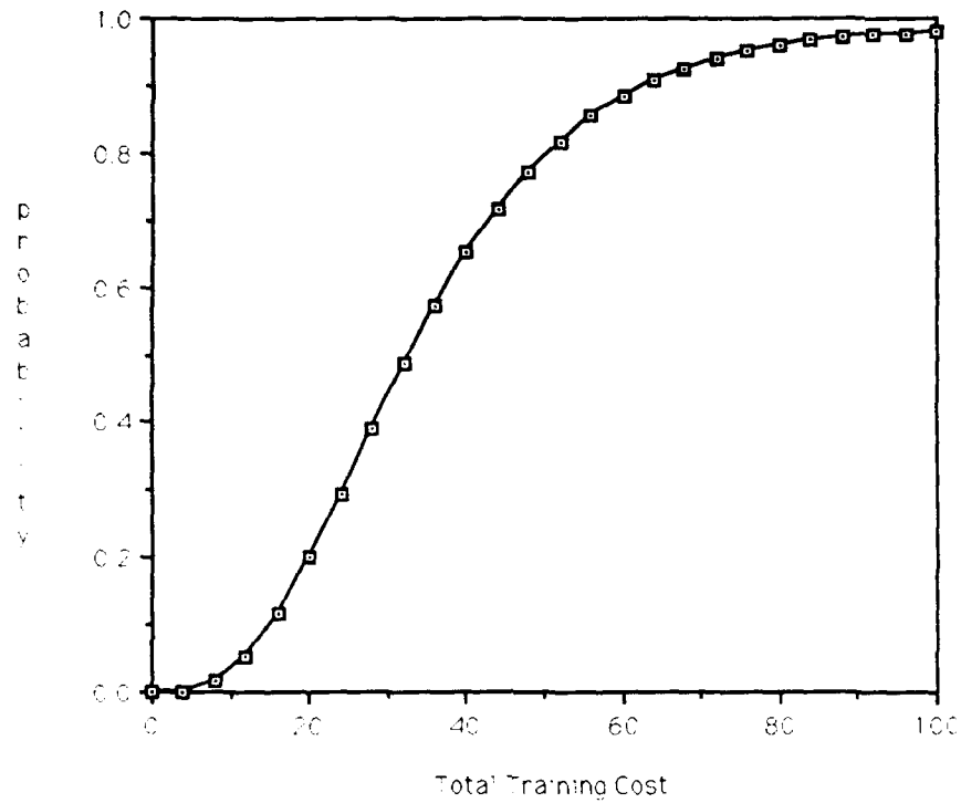
Figure 3.1 The Distribution of W(X^G)
