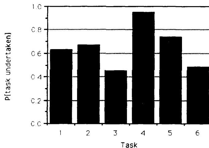
Figure 3.3. Probability each Task is Undertaken
