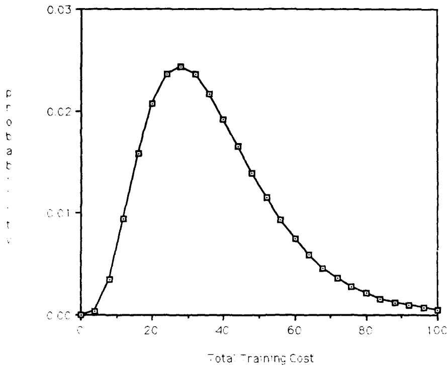
Figure 3.2. The Density of W(X^G)
