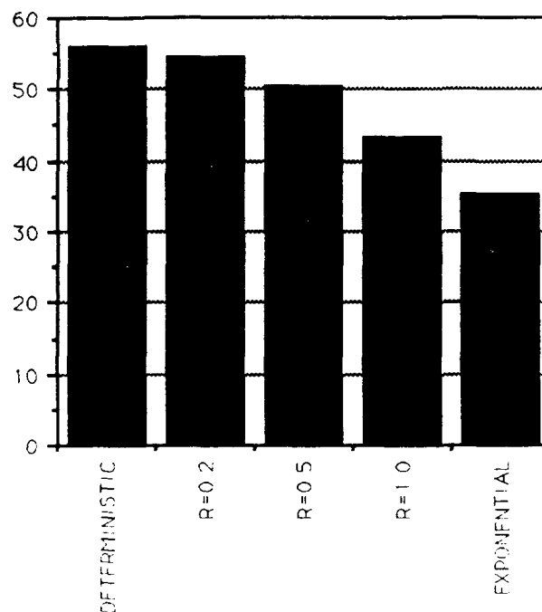
Figure 4.1a. Expected Value Bounds for Uniform Task Values
