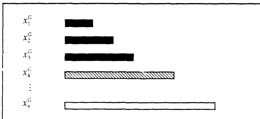
Figure 2.2a Linear Objective Function
