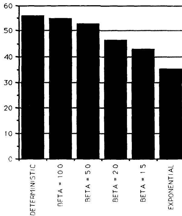
Figure 4.1b. Expected Value Bounds for Weibull Task Values
