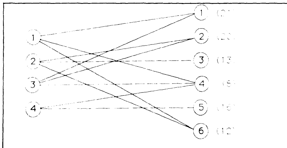
Figure 2.4. Bipartite Graph with Node Weights
