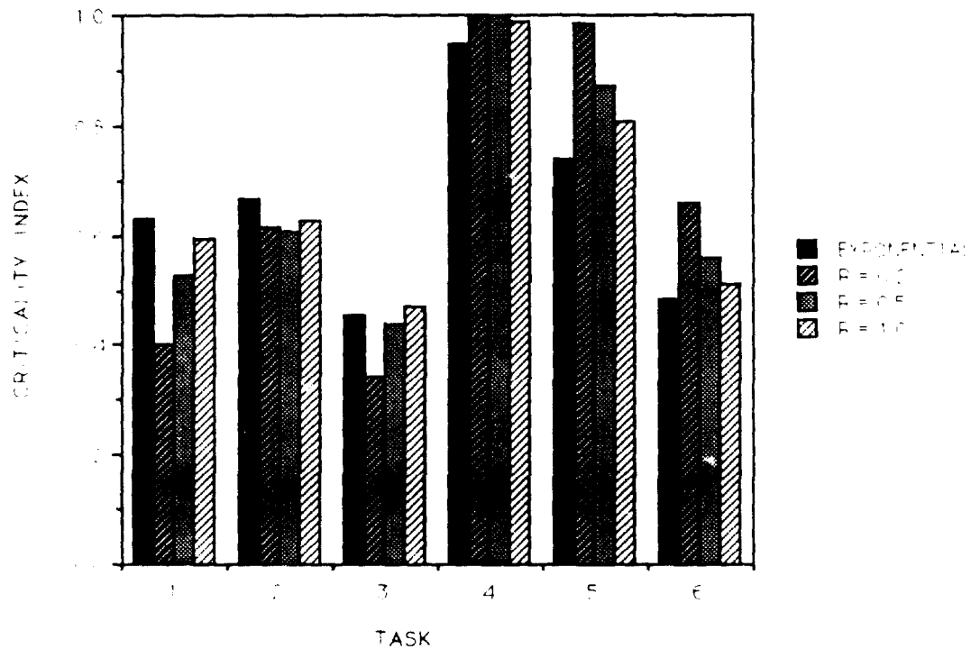
Figure 4.3a. Criticality indices from uniform task values
