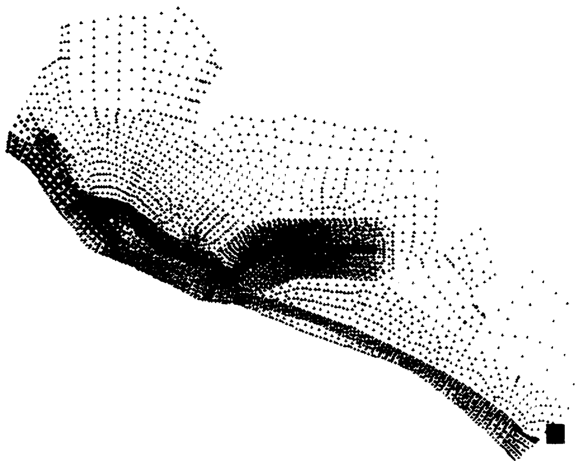
FIGURE E-14. Computed Bed Shear Stresses of Plan 1 Condition.
