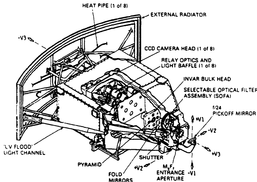
Figure 1: The Wide Field, Planetary Camera (WF/PC) (taken from [15])
