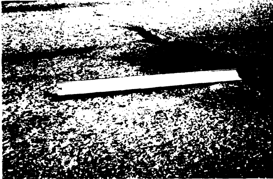
Figure A11. Low-severity bumps and sags.
