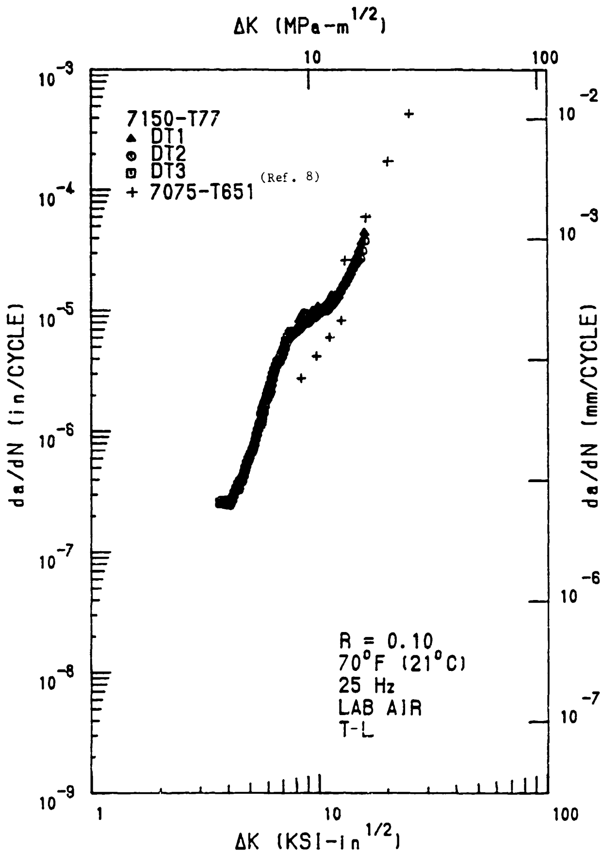
Figure 8. Fatigue Crack Growth Rate Data for 7150-T7751 T-L Orientation.
