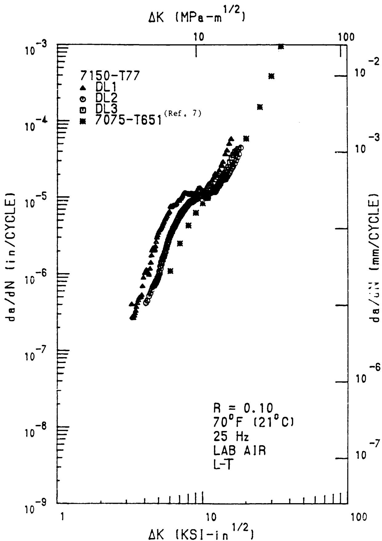
Figure 7. Fatigue Crack Growth Rate Data for 7150-T7751 L-T Orientation.
