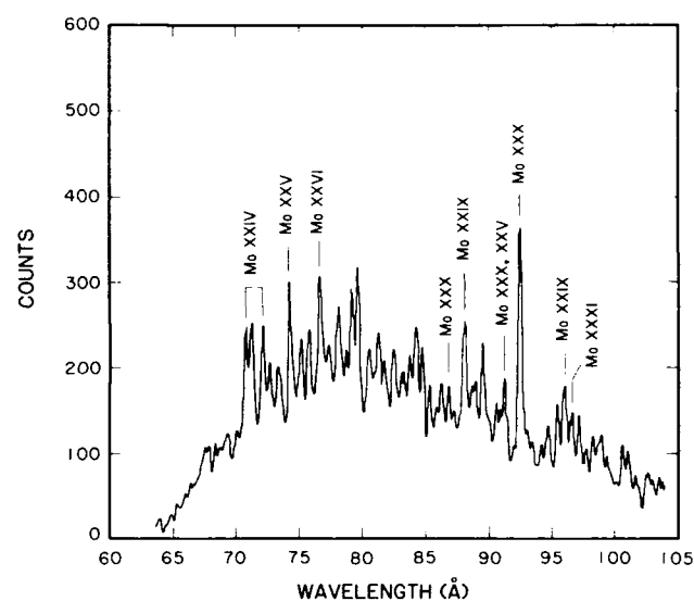
Fig. 2. Mo spectrum in the wavelength region 60–105 Å.
