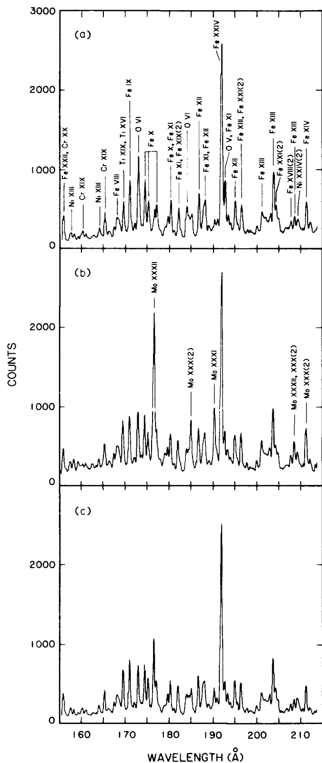
Fig. 1. Spectra recorded at intervals of 50 msec during a PLT discharge. Spectrum (a) was recorded just before injection, and spectra (b) and (c) were recorded after injection of Mo.
