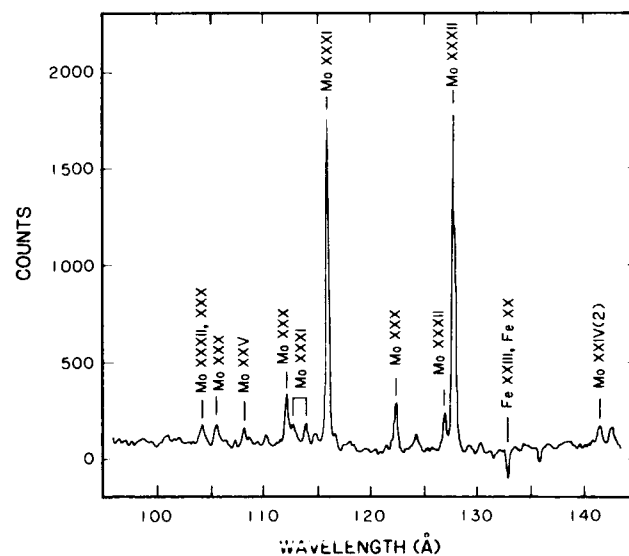
Fig. 3. Mo spectrum in the wavelength region 95-145 Å.
