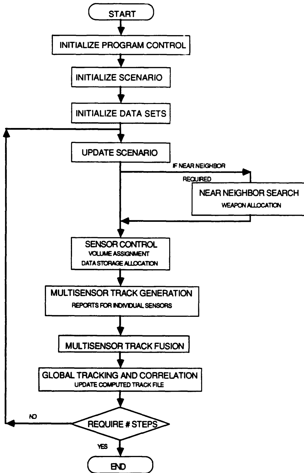
Figure 1: Block Diagram of the BEAST code
