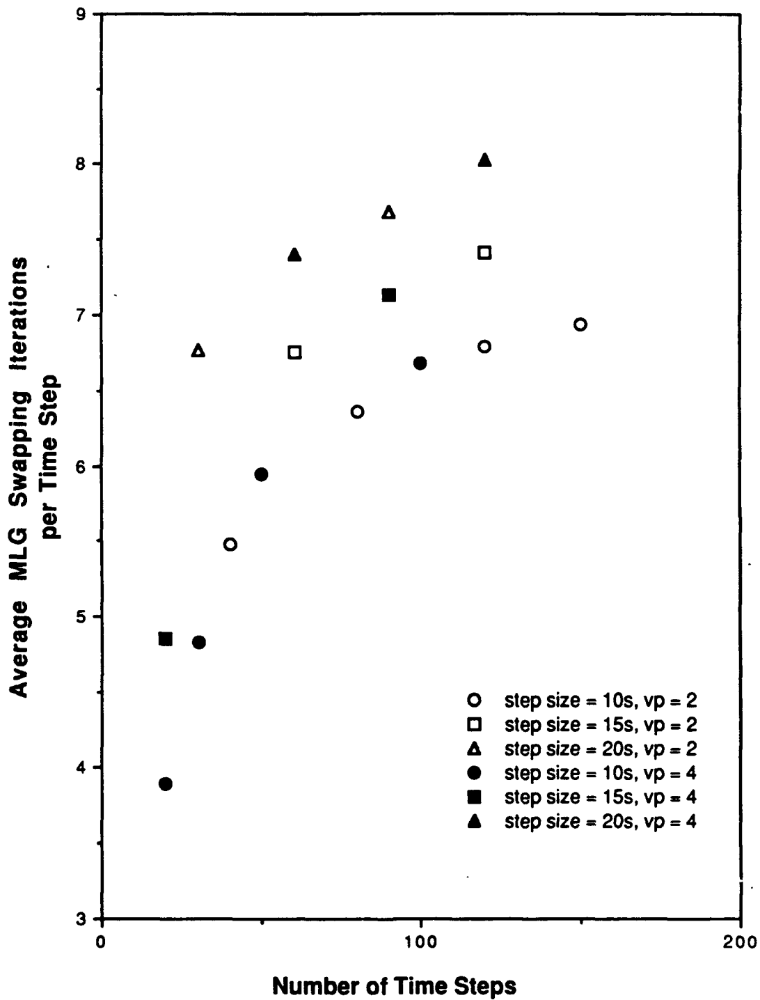
Figure 7: Average MLG Swaps versus Time Step for 32 x 32 x 32 System
