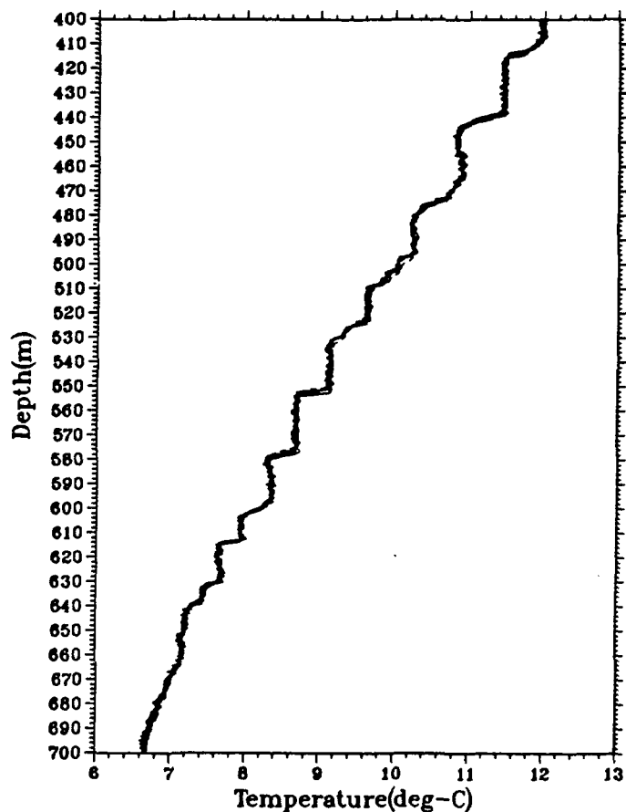
Figure 13. Expanded profile plots of temperature for (a) 0 - 200 m, and (b) 400 - 700 m. CTD data - dashed, XCTD data - solid. XCTD depths are recalculated with individually determined coefficients (Method-II, Case-I).
