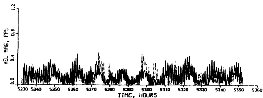
COMPUTED (SOLID) VS OBSERVED (DOTTED)
