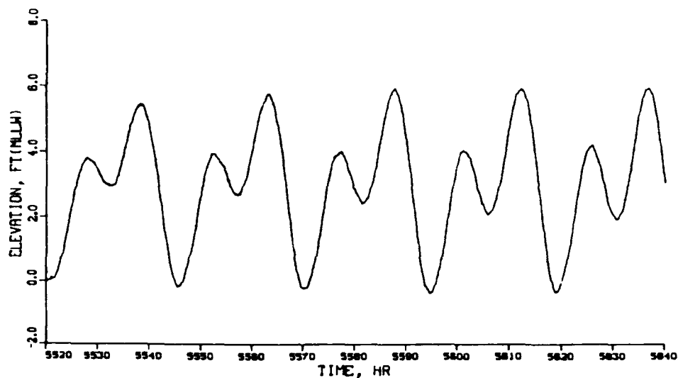
Figure 19. Ocean tide boundary condition for verification period
