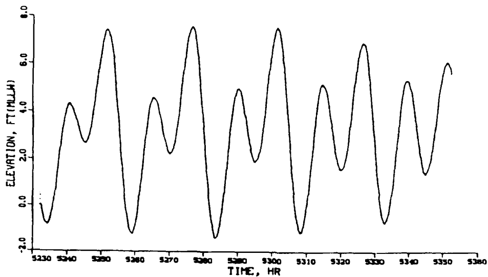
Figure 17. Ocean tide boundary condition for calibration period
