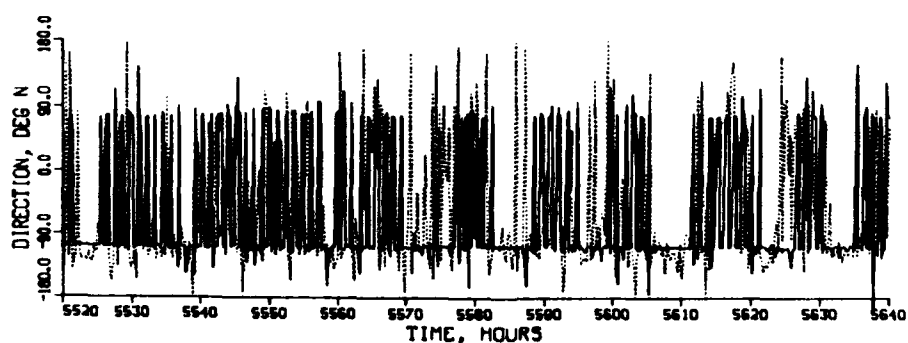
COMPUTED (SOLID) VS OBSERVED (DOTTED)
