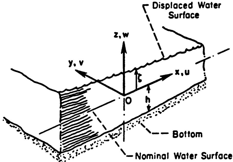
Figure 4. Coordinate system
