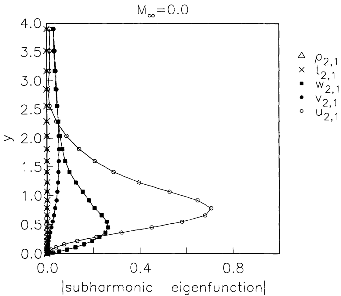
Fig.17: Subharmonic eigenfunction at M_\infty \approx 0.0 . The parameters are \alpha = 0.29 , \theta = 0^\circ , T_\infty = 520^\circ R , Re = 1675 , and A = 1.5\% .
