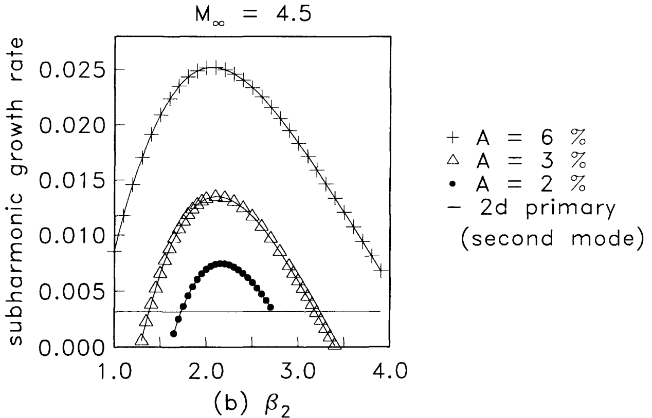
Fig.11: Subharmonic instabilities at M_\infty = 4.5 . (a) \alpha = 0.6, \beta = 0 and various A . (b) \alpha = 2.52, \beta = 0 and various A . — primary growth rate.
