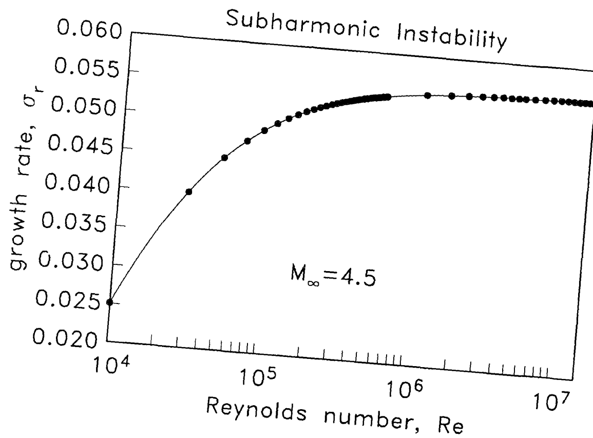
Fig.20: Subharmonic growth rate as a function of the Reynolds number.
