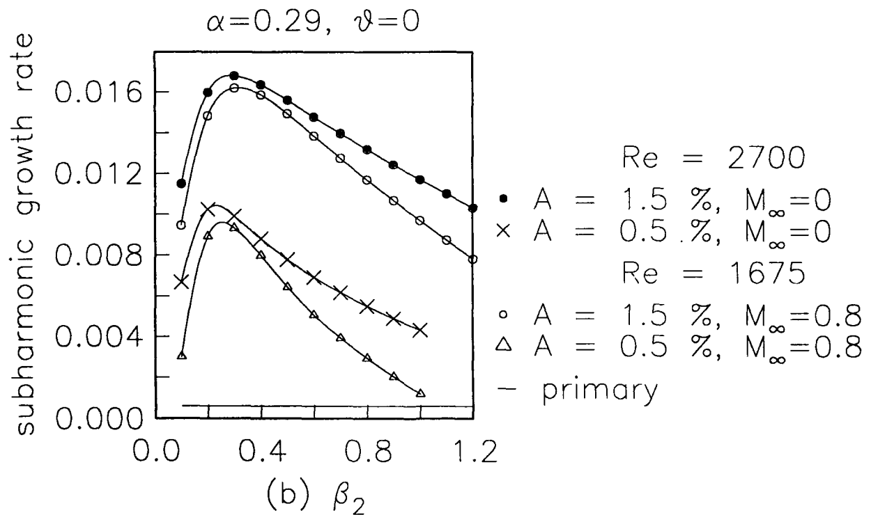
Fig.7: Comparisons between the subharmonic growth rates at M_\infty = 0.0 and M_\infty = 0.8 .
