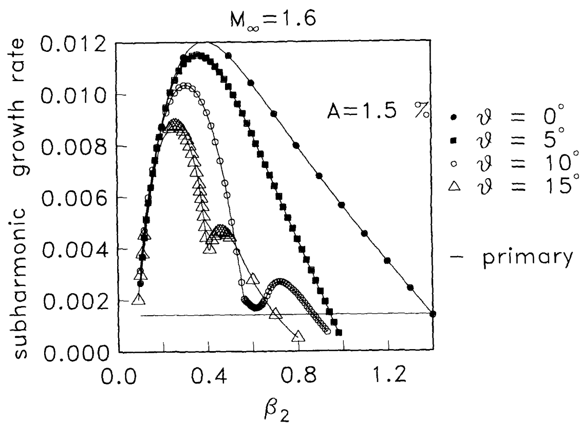
Fig.23: Subharmonic instabilities at M_\infty = 1.6 for various \theta . — primary growth rate at \theta = 45^\circ .
