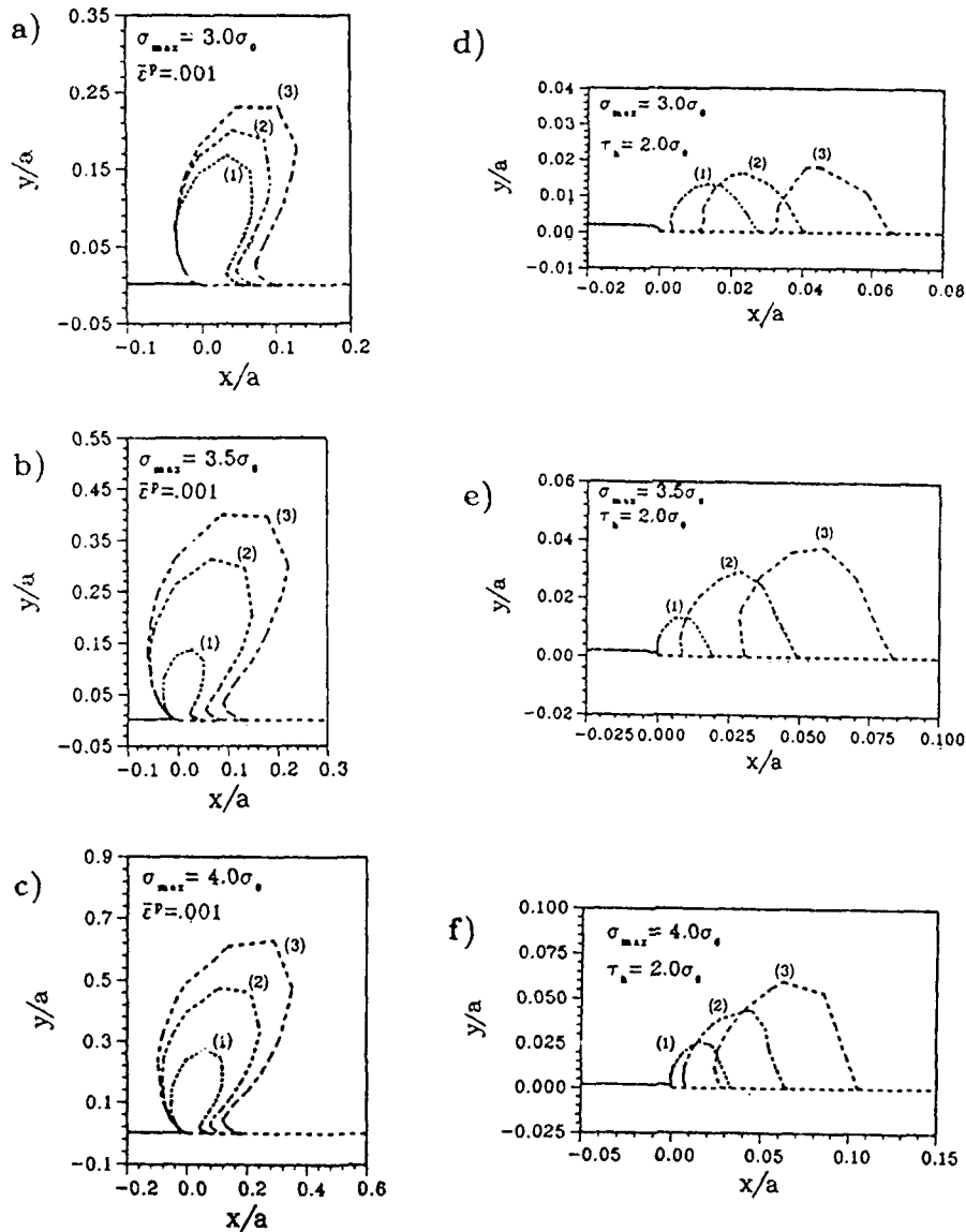
Fig. 18. (a)–(c) Contours of effective plastic strain \bar{\epsilon}^p = 0.001 ; (d)–(f) hydrostatic stress contours of \tau_h = 2.0\sigma_0 for different values of interface strength. The amount of crack growth is approximately the same for all three values of \sigma_{\max} ; curve (1) \Delta a = 0 ; curve (2) \Delta a \approx 10\delta_c ; curve (3) \Delta a \approx 45\delta_c .
