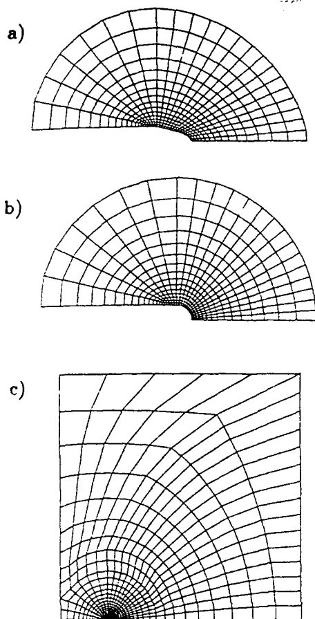
Fig. 5. Finite element meshes used in the study of interfaces containing long or intermediate-size flaws ( a_0/\delta_c \approx 1500 or 150): (a) notch with elliptical tip; (b) notch with circular tip; (c) remote mesh.
