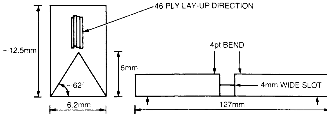
FIG. 4 TEST SPECIMEN
