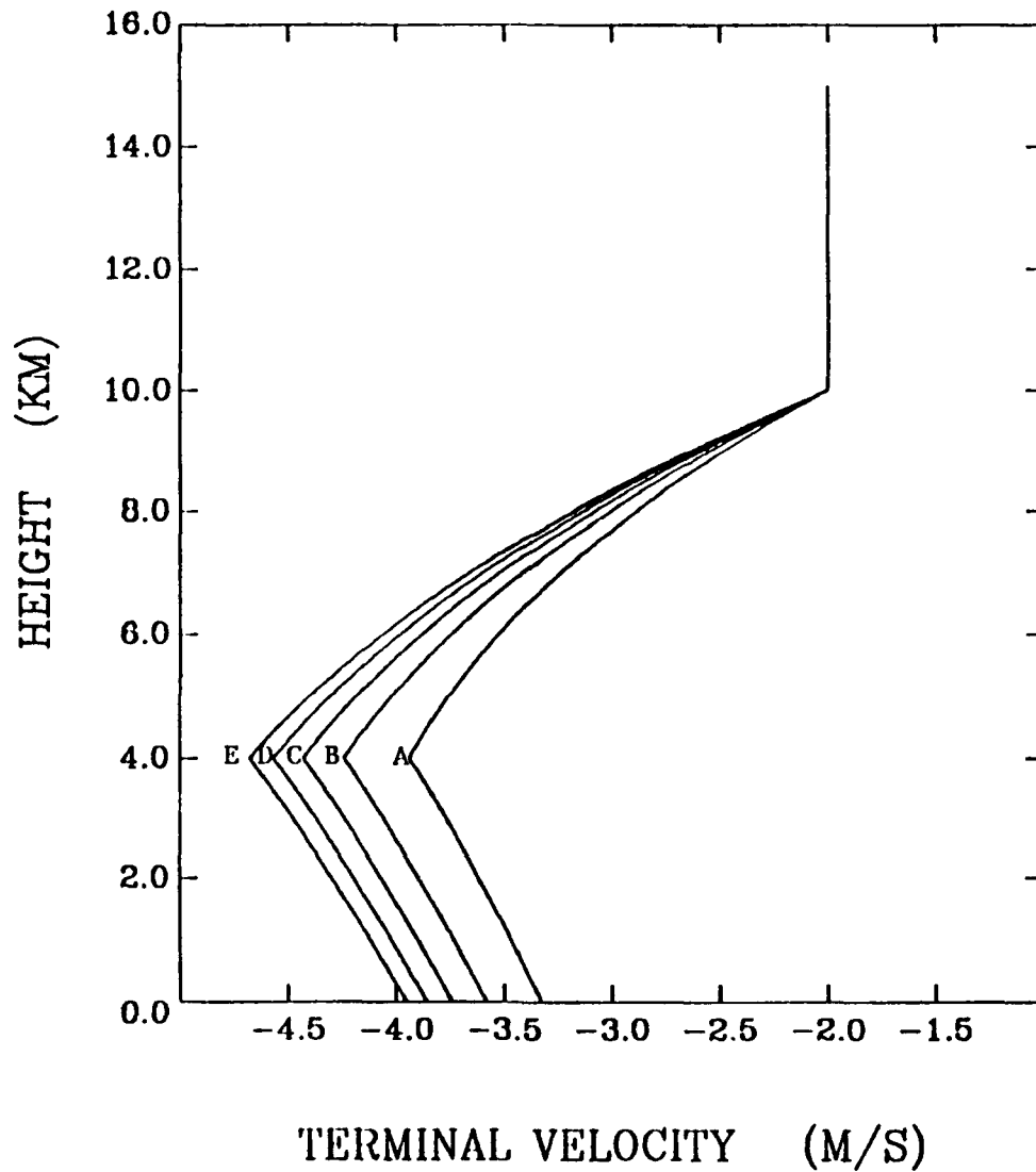
Fig. A1. Terminal velocities from the adjusted Joss and Waldvogel (1970) equations. Plotted lines are done for: (A) 10 dBZ, (B) 20 dBZ, (C) 30 dBZ, (D) 40 dBZ, and (E) 50 dBZ. Negative velocities denote downward speed. All plots have a value of -2 \text{ ms}^{-1} above the 10 km height level.
