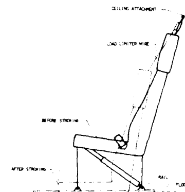
Figure 19. Schematic diagram of base-mounted seat (NASA)
