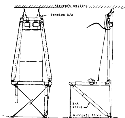
Figure 13. TH 60 Troop Seat
