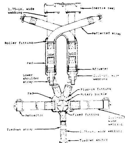
Figure 20. Reflected shoulder strap harness system
