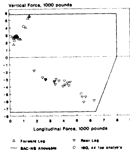
Figure 22. Graph showing Vertical Force (1000 pounds) vs. Longitudinal Force (1000 pounds) (NASA)
