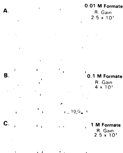
FIGURE 1 ESR spectra of DMPO-OH and DMPO-CO 2 - spin adducts obtained in the reaction of VO 2+ with H 2 O 2 in the presence of DMPO and varying concentrations of formate.
