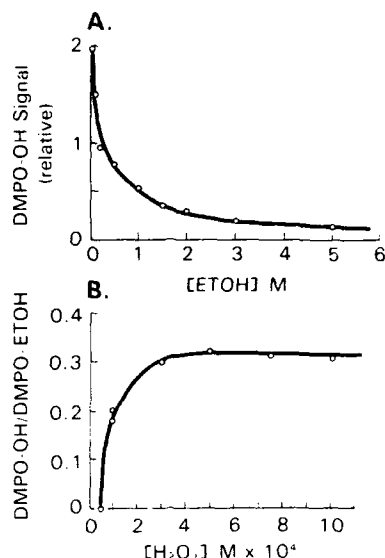
FIGURE 3 (A) DMPO-OH ESR signal intensity as a function of increasing concentration of ethanol in the \text{VO}^{2+}/\text{H}_2\text{O}_2 reaction. (B) DMPO-OH ESR signal intensity as a function of hydrogen peroxide concentration obtained during the \text{VO}^{2+}/\text{H}_2\text{O}_2 reaction in the presence of a constant concentration of ethanol.
