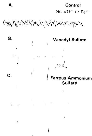
FIGURE 4 \text{DMPO-OH} ESR signal obtained in the reactions of vanadyl and ferrous ions with hydrogen peroxide at pH 5.5.
