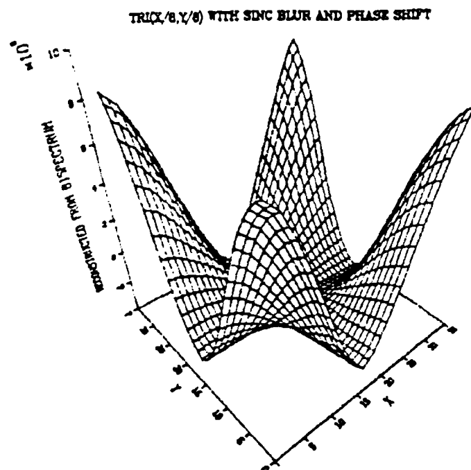
Figure 23b. Bispectrally Reconstructed Version of (a)
