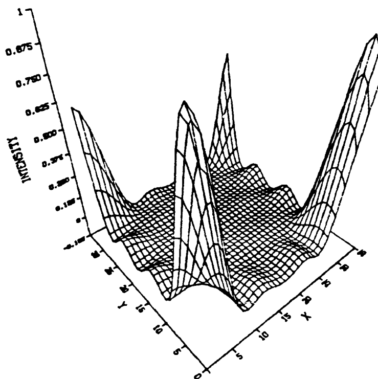
Figure 17a. Three-Dimensional Plot of Bispectrally-Reconstructed \text{Sinc}^2(X/16, Y/16)
