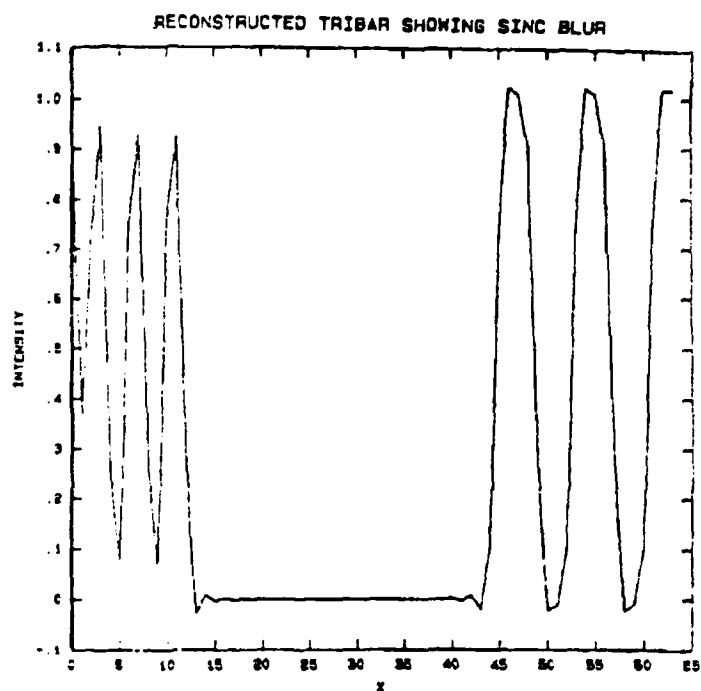
Figure 22b. Bispectrally Reconstructed Version of (a)
