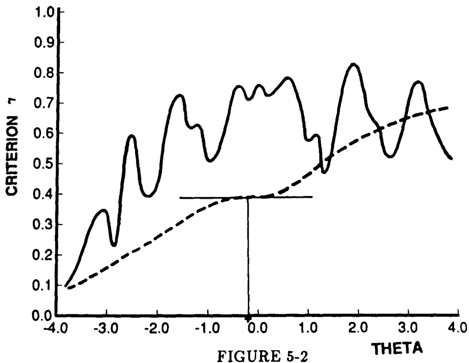
Relationships among \theta , \gamma , p_a , \xi(\gamma|\theta) and \zeta(\theta) .
