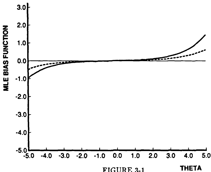
FIGURE 3-1 MLE Bias Functions of the Iowa Level 11 Vocabulary Subtest (Solid Line) and of Shiba's Test J1 of Word/Phrase Comprehension (Dashed Line), Following the Normal Ogive Model.
