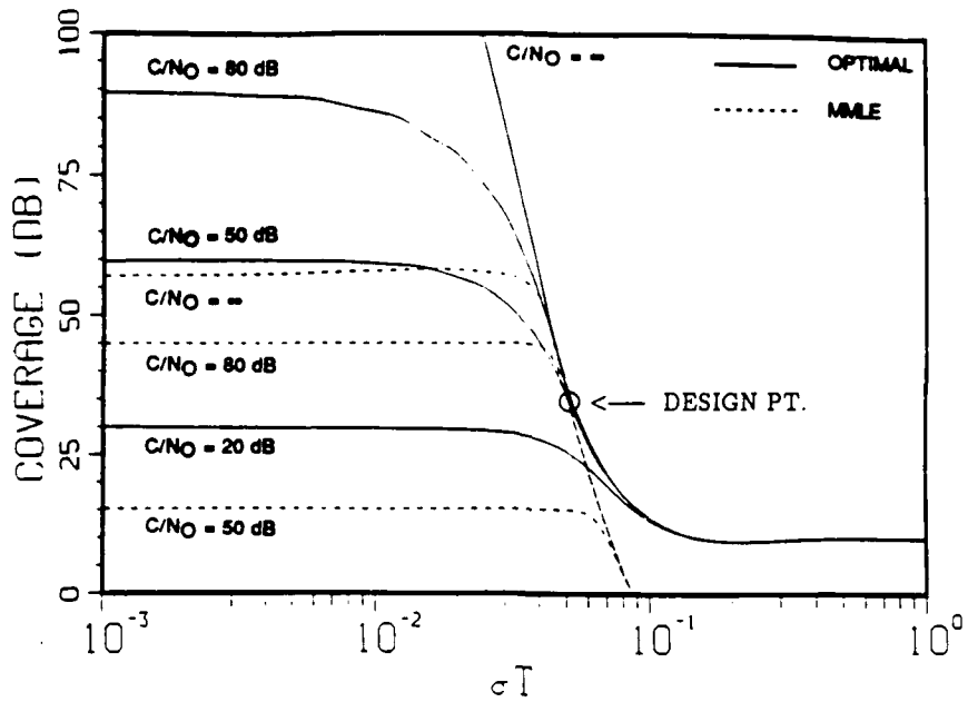
Fig. 21 — Coverage MMLE f = 0.2 , N = 10 \sigma_c T = 0.05 , C/N_0 = 20, 50, 80, \infty dB
