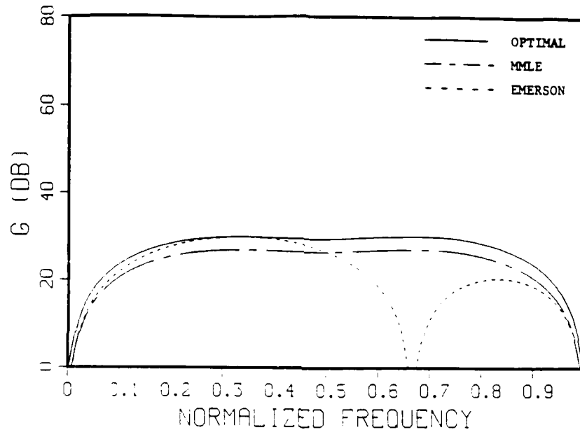
Fig. 7 — Gain-interference matrix (17). N = 3
