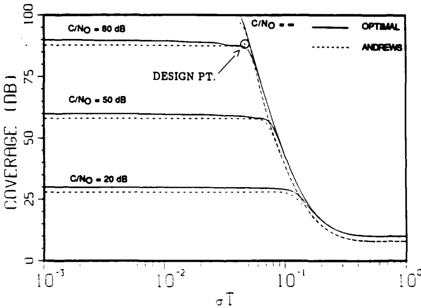
Fig. 18 — Coverage Andrews f = 0.5, N = 10 \sigma_c T = 0.05, C/N_0 = 20, 50, 80, \infty dB
