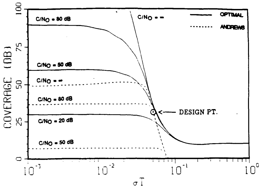
Fig. 19 — Coverage Andrews f = 0.2 , N = 10 , \sigma_c T = 0.05 , C/N_0 = 20, 50, 80, \infty dB
