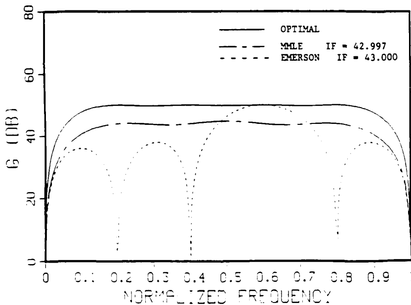
Fig. A1 — Interference matrix (17), N = 5
