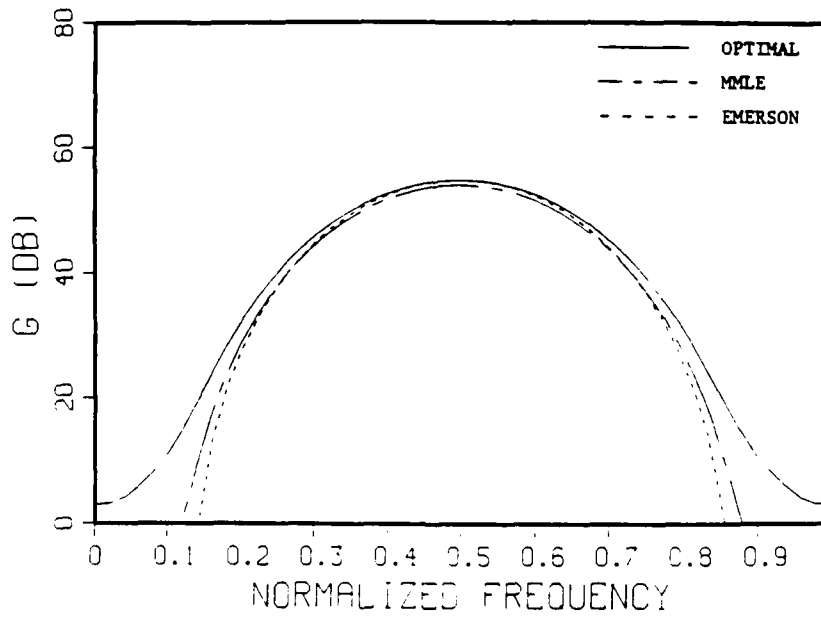
Fig. 2 — Gain-Gaussian clutter power spectrum N = 6 , \sigma_c T = 0.05 , C/N_0 = 50 dB
