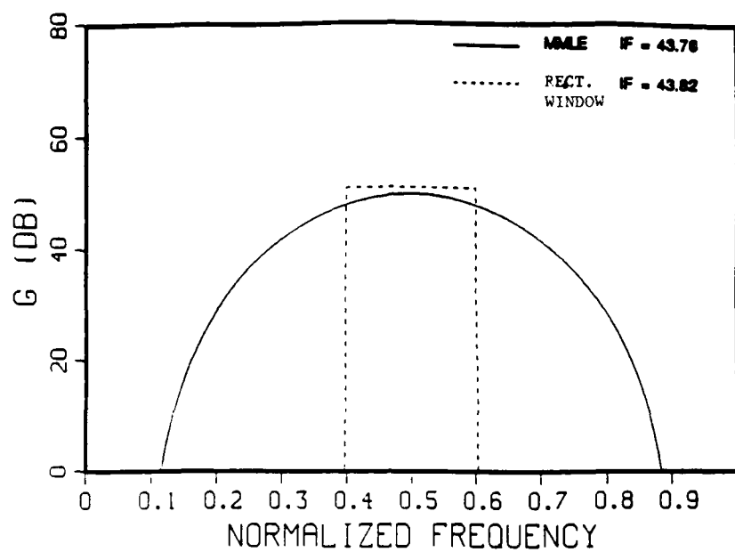
Fig. A2 — Improvement factors
