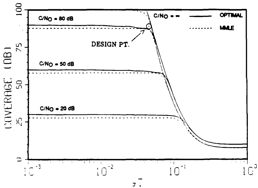
Fig. 20 — Coverage MMLE f = 0.5 , N = 10 , \sigma_c T = 0.05 , C/N_0 = 20, 50, 80, \infty dB
