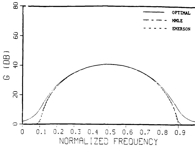
Fig. 1 — Gain-Gaussian clutter power spectrum N = 4 , \sigma_c T = 0.05 , C/N_0 = 50 dB
