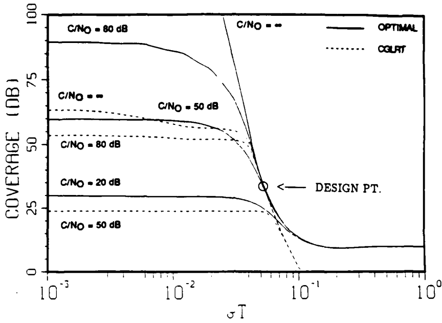
Fig. 17 — Coverage CGLRT f = 0.2, N = 10 \sigma_c T = 0.05, C/N_0 = 20, 50, 80, \infty dB
