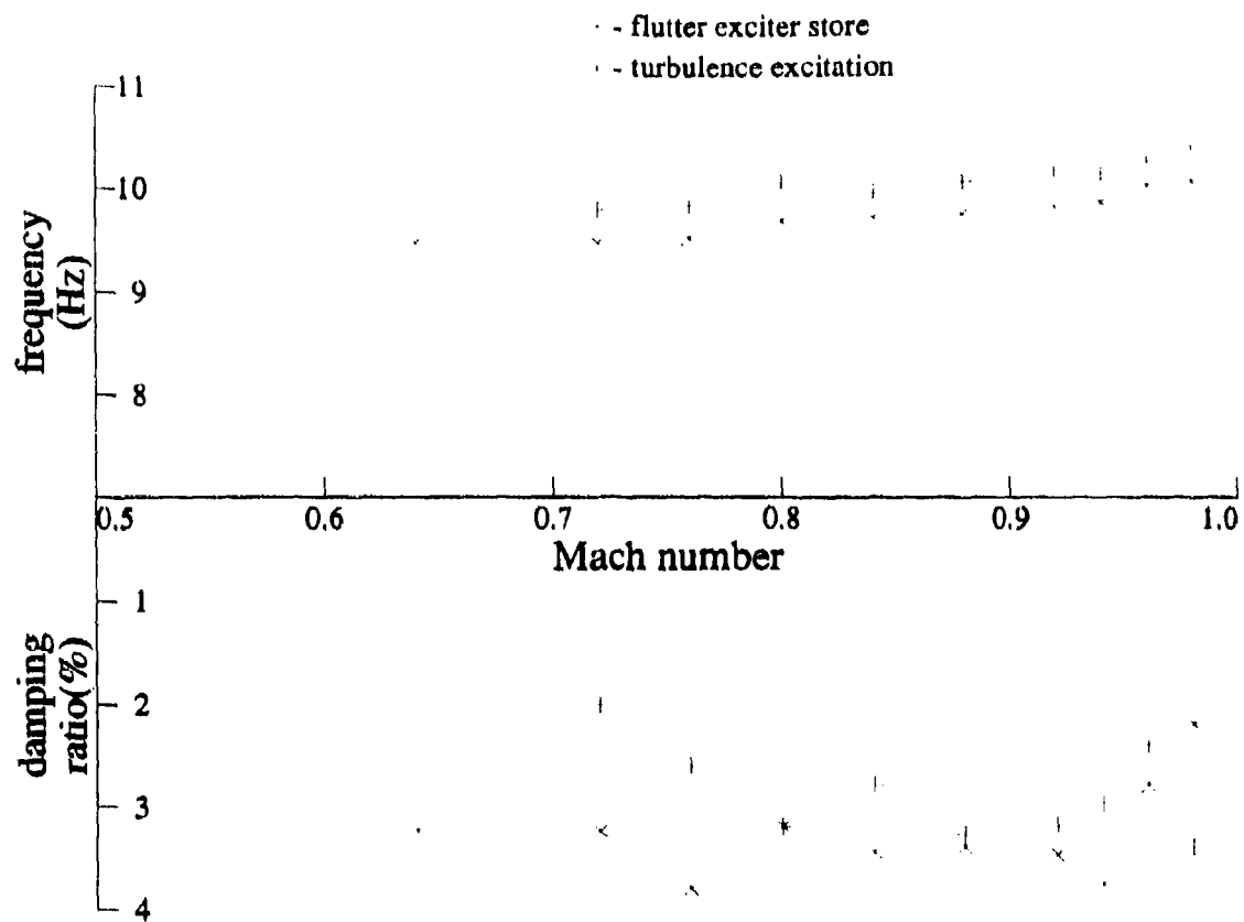
Figure 6. Comparison of two excitation methods
