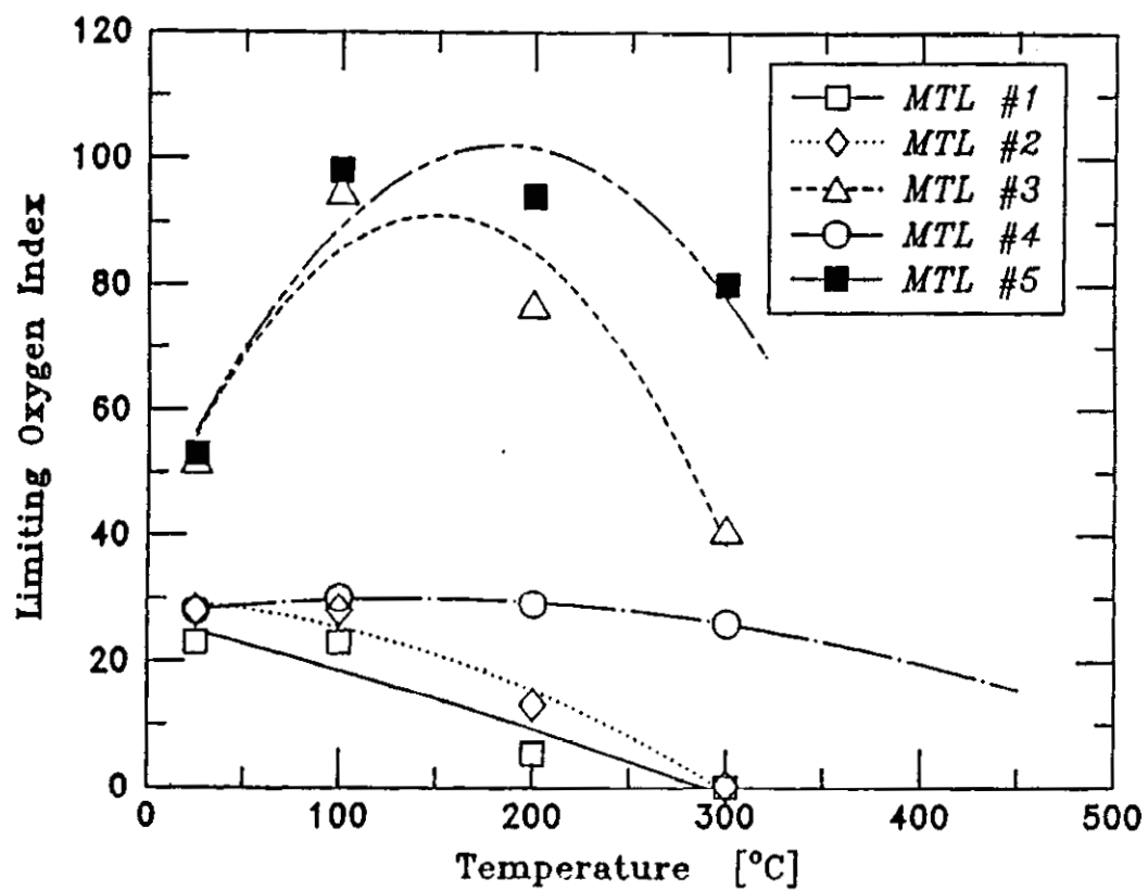
Figure 3. Limiting oxygen index as a function of environmental temperature in the oxygen index apparatus for composite materials.
